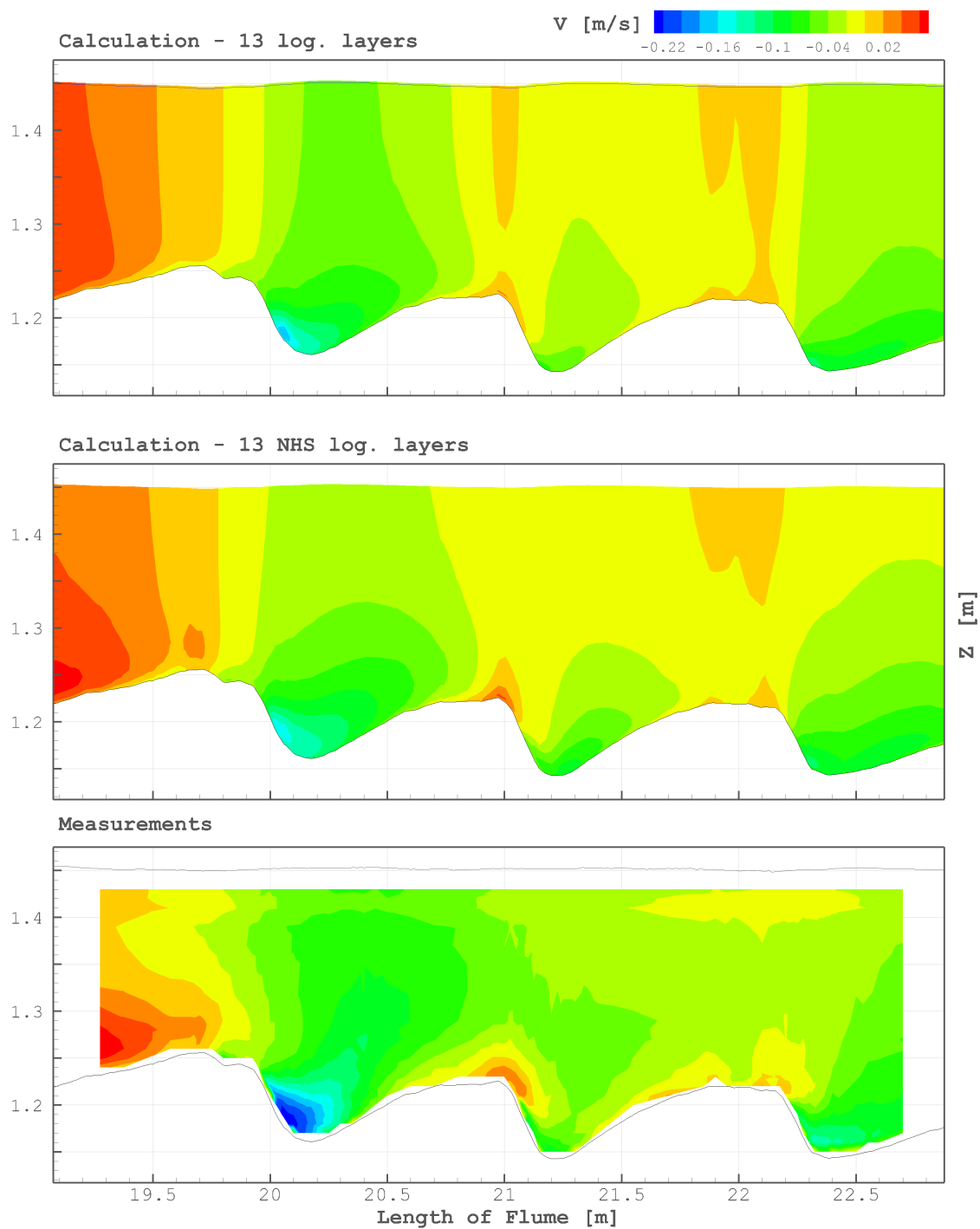
Figure 5.13: Comparison of velocity v [m/s] obtained with hydrostatic pressure approach (top) and non-hydrostatic pressure approach (NHS) (middle) to measurements (bottom). Data sets No. 10 and 13 of Table 5.1
