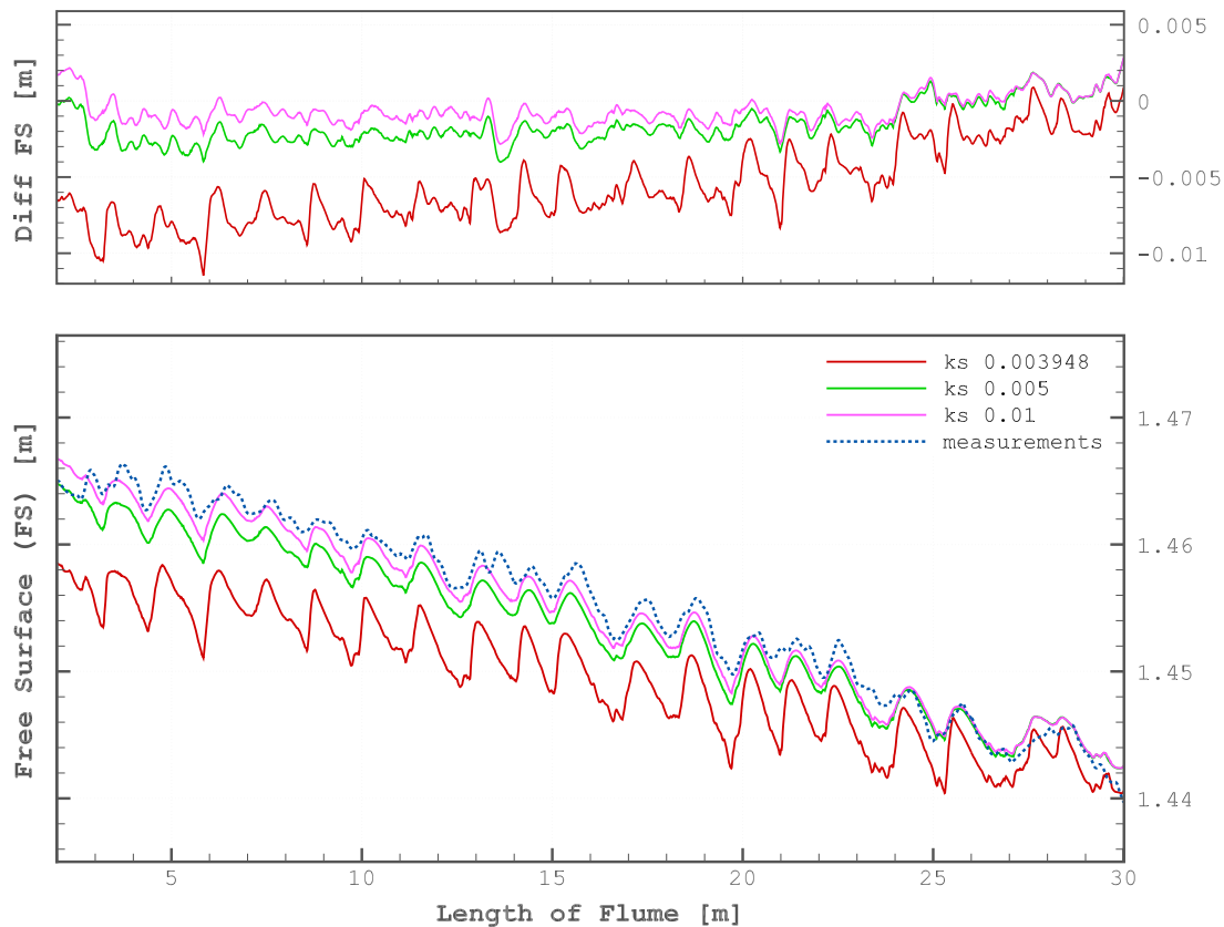
Figure 5.10: Free surface levels obtained with k_s of 0.00395 m, 0.005 m and 0.01 m and differences to measurements (top), calculations with fine mesh. Data sets No. 1, 2, 3 of Tbl. 5.1
