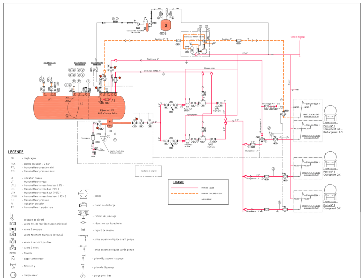
Figure 4-6 Diagramme PID
