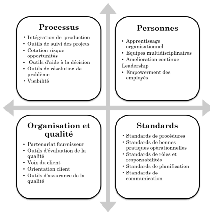
Figure 10 : Facilitateurs Lean.
