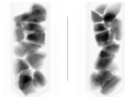
Figure 2.16: Two orthogonal projections of the specimen used for validating the D-DPC experimental test in Sec. 2.8
