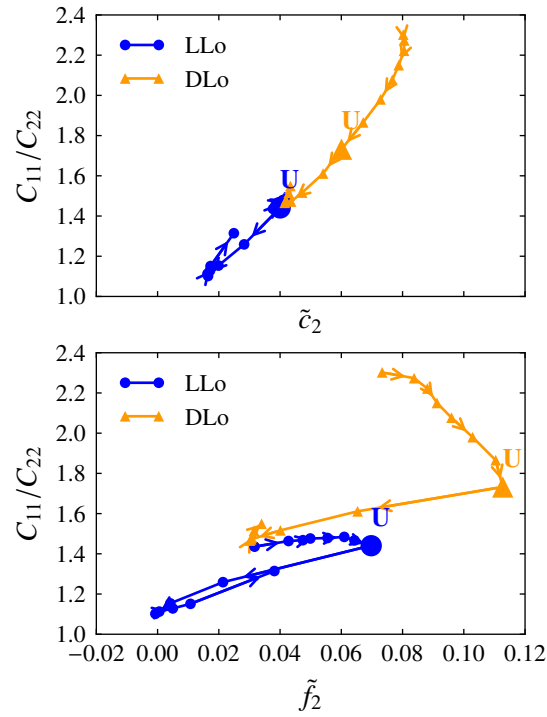
Figure 5.16: (top) Variations of the ratio C_{11}/C_{22} with \tilde{c}_2 and (bottom) \tilde{f}_2
