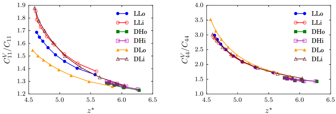
Figure 5.12: Ratios of Voigt estimates to true moduli C_{11} (left) and C_{44} (right) versus rattler-corrected coordination number z^* .
