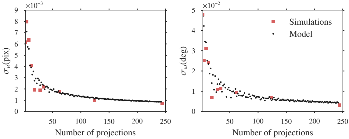
Figure 3.2: Noise error evolution as a function of the projections number for one grain: The squares link the number of projections used to the standard deviation of the obtained error. The standard deviations are computed from ten realizations. The black dots are the estimated noise error using the model developed in 3.2.
