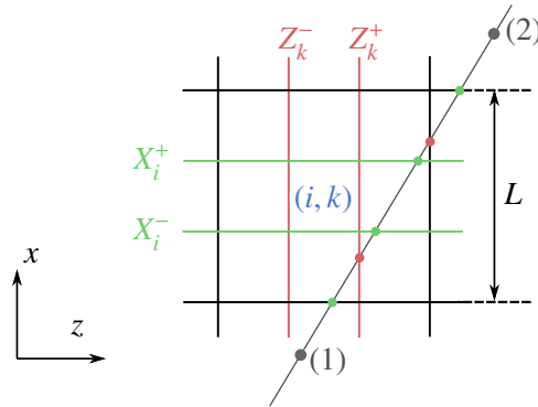
Figure 2.7: Illustration of the image definition by intersecting planes in Siddon's algorithms. The voxel (i, k) is defined from the intersection of the planes X_i^- and X_i^+ with the planes Z_k^- and Z_k^+ . A ray defined from points (1) and (2) is drawn and its intersections with X-planes and Z-planes provide the different \alpha 's.
