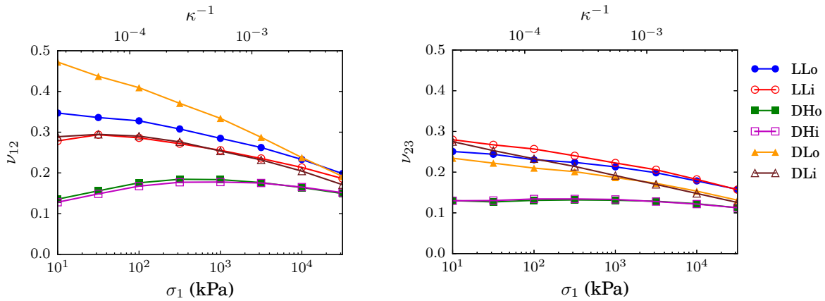
Figure 5.8: Poisson ratios (left) \nu_{12} and (right) \nu_{23} versus \sigma_1 or \kappa^{-1} .
