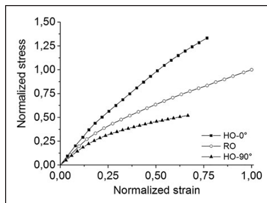
Figure 4. Normalized quasi-static tensile behavior of A-SMC composite at room temperature. One can mention that normalized stress (respectively strain) = stress (respectively strain)/ultimate stress (respectively strain) obtained for tests performed on RO-A-SMC serving as a reference.
