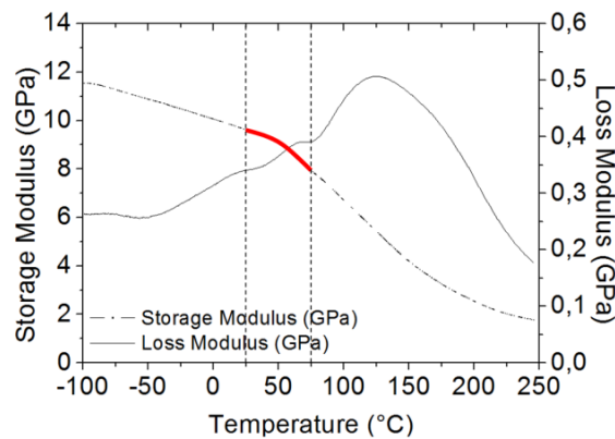
Fig. 4. DMTA test performed on RO-A-SMC
