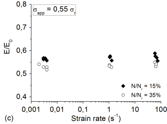
Fig. 13. Influence of strain rate on the elastic modulus:
