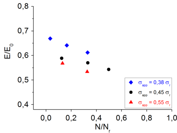
Fig. 14. Evolution of Young Modulus of fatigued samples under different conditions
