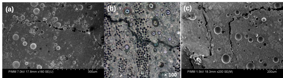
Fig. 17. Matrix microcracking from HO- 90^\circ tensile test interrupted during the gradual stress decrease (see Fig.14.b): a) Progressive “unbuttoning” at the HGM-matrix interfaces, b) Easy propagation through 90^\circ oriented bundle, c) Deviation of matrix micro-cracks by more disoriented bundles
