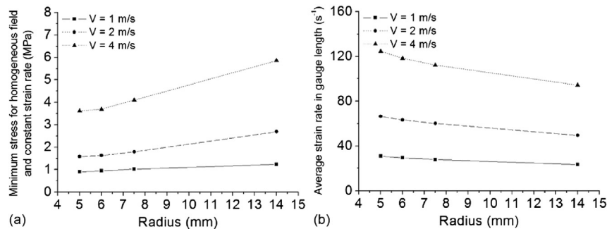
Fig. 4. Influence of the radius of the specimen; (a) Minimum stress for which homogeneous field and constant strain rate is obtained (b) Strain rate in the central zone.
