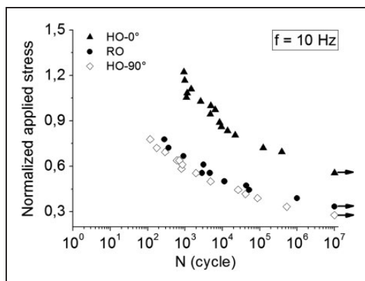
Figure 8. Normalized Wöhler curves for HO-0°, RO, and HO-90° samples at 10 Hz.
