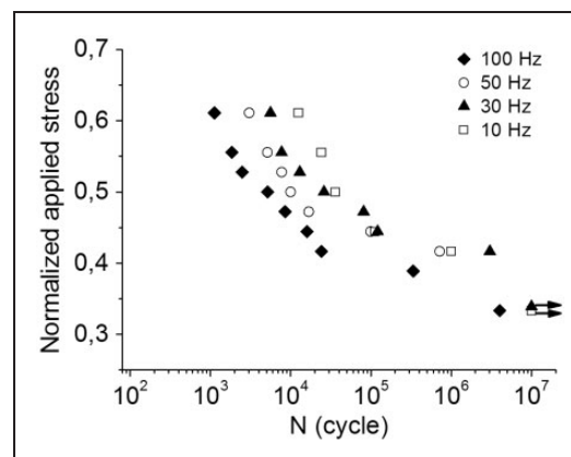
Figure 9. Normalized Wöhler curves at different frequencies for RO samples.
