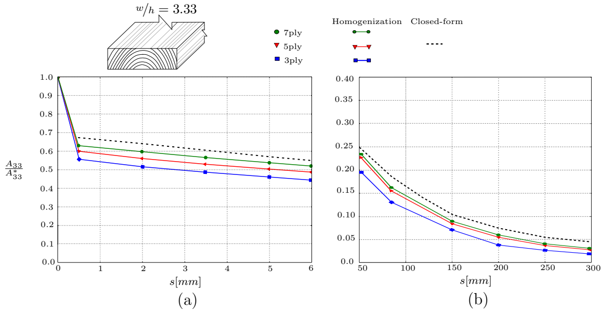
Figure 4.14: Variation of normalized in-plane shear stiffness \frac{A_{333}}{A_{33}^*} for (a) small and (b) large spaces for ratio w/h = 3.33 of lamellas and for 3, 5 and 7 layers
