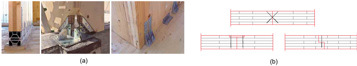
Figure 1.3: Connections in CLT construction: (a) metallic fasteners for anchoring CLT walls and (b) butt-joint between CLT panels (XlamDolomiti 2016)
