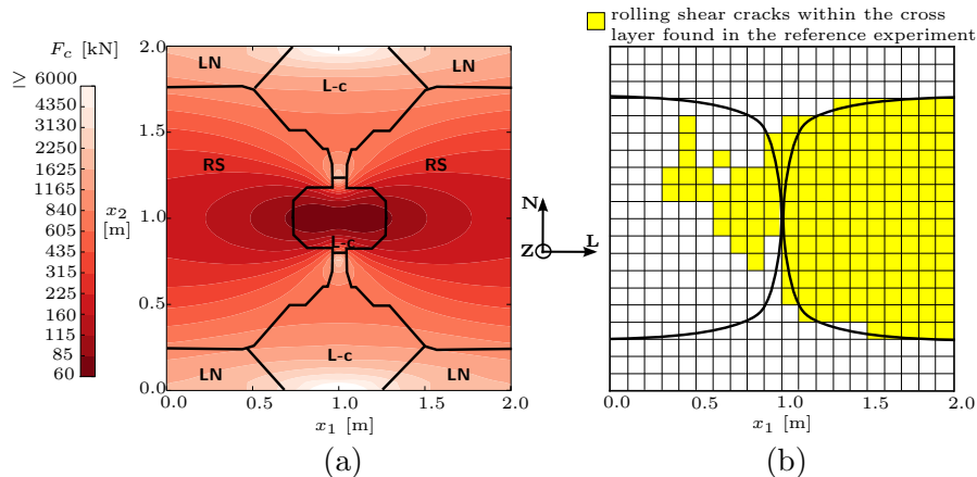
Figure 2.7: Horizontal section of the plate at x_3 = +13mm . Failure stages predicted with the discontinuous model (a) and the corresponding cracking pattern found in the reference experiment (b)
