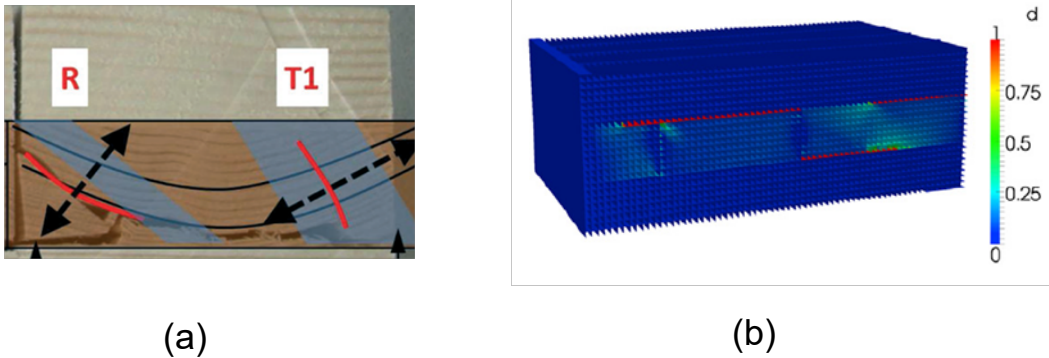
Figure 1.9: Stress concentration in laterally unglued transverse CLT boards due to free edges found (a) experimentally by Hochreiner et al (2013) and (b) numerically by Flores et al (2016) (b) for out-of-plane loads
