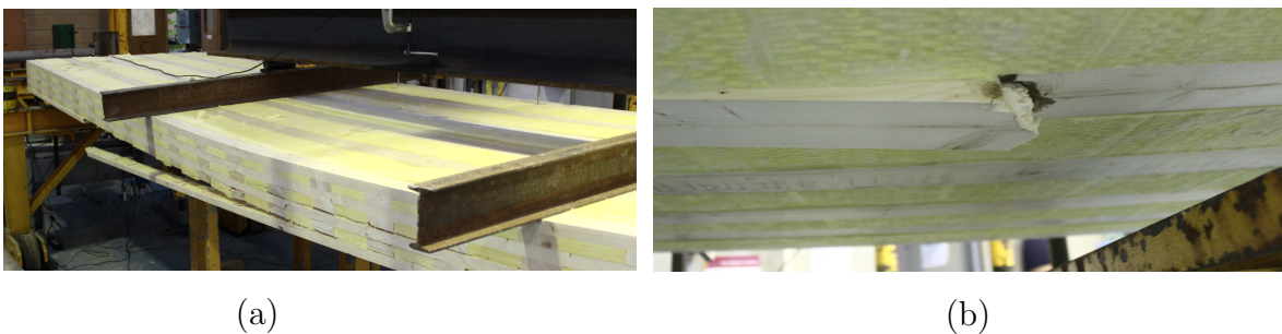
Figure 3.5: Tensile failure of s=150 mm panel (a) and detail of failure due to a local knot (b)
