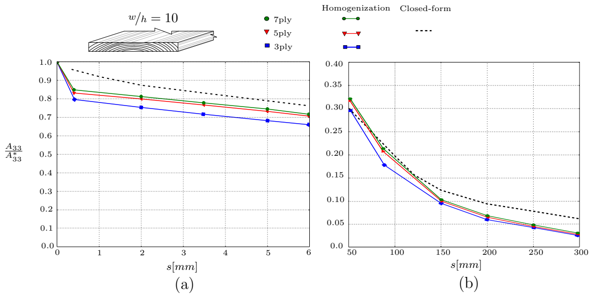
Figure 4.15: Variation of normalized in-plane shear stiffness \frac{A_{333}}{A_{33}^*} for (a) small and (b) large spaces for ratio w/h = 10 of lamellas and for 3, 5 and 7 layers
