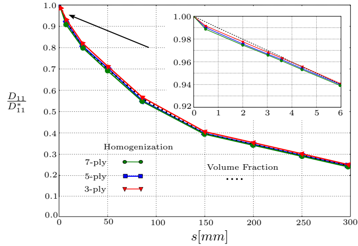
Figure 4.8: Variation of the normalized stiffness \frac{D_{11}}{D_{11}^*} as a function of spaces between lamellas
