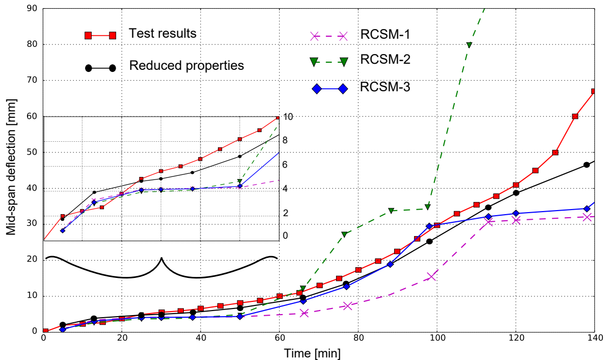
Figure 6.10: Comparison between the experimental and predicted mid-span deflection of Test-1
