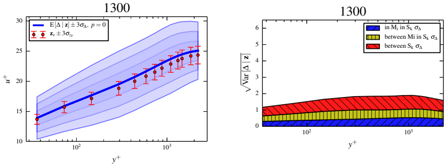
(a) The BMSA prediction for validation case 1300. (b) The BMSA standard deviation for validation case 1300.
