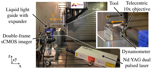
Fig. 1 Experimental setup for orthogonal cutting testing.
