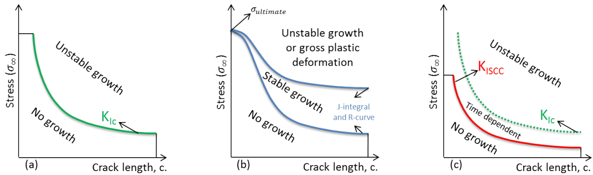
Figure 1.29: The cracking behavior as a function of the crack length and the stress intensity factor. From [12].
