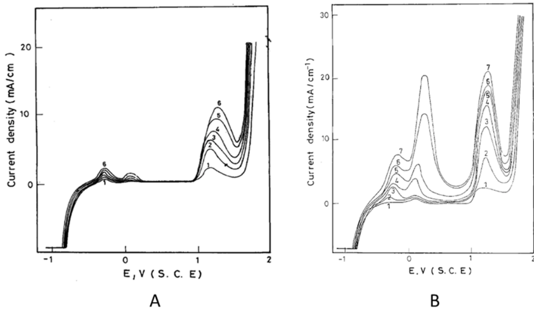
Figure 1.3: Polarization curves of 304 stainless steel produced at 25°C (A): using a sweep rate of 50 \text{ mV.s}^{-1} to check the effect of \text{H}_2\text{SO}_4 concentrations on the polarization curve. (1): 0.1 M, (2): 0.3 M, (3): 0.5 M, (4): 0.7 M, (5): 0.9 M, (6): 1 M. (B): using a 0.5 M \text{H}_2\text{SO}_4 solution to check the effect of different scan rates on the polarization curve. (1): 10 \text{ mV.s}^{-1} , (2): 50 \text{ mV.s}^{-1} , (3): 100 \text{ mV.s}^{-1} , (4): 250 \text{ mV.s}^{-1} , (5): 500 \text{ mV.s}^{-1} , (6): 750 \text{ mV.s}^{-1} , (7): 1 \text{ mV.s}^{-1} . From [4].
