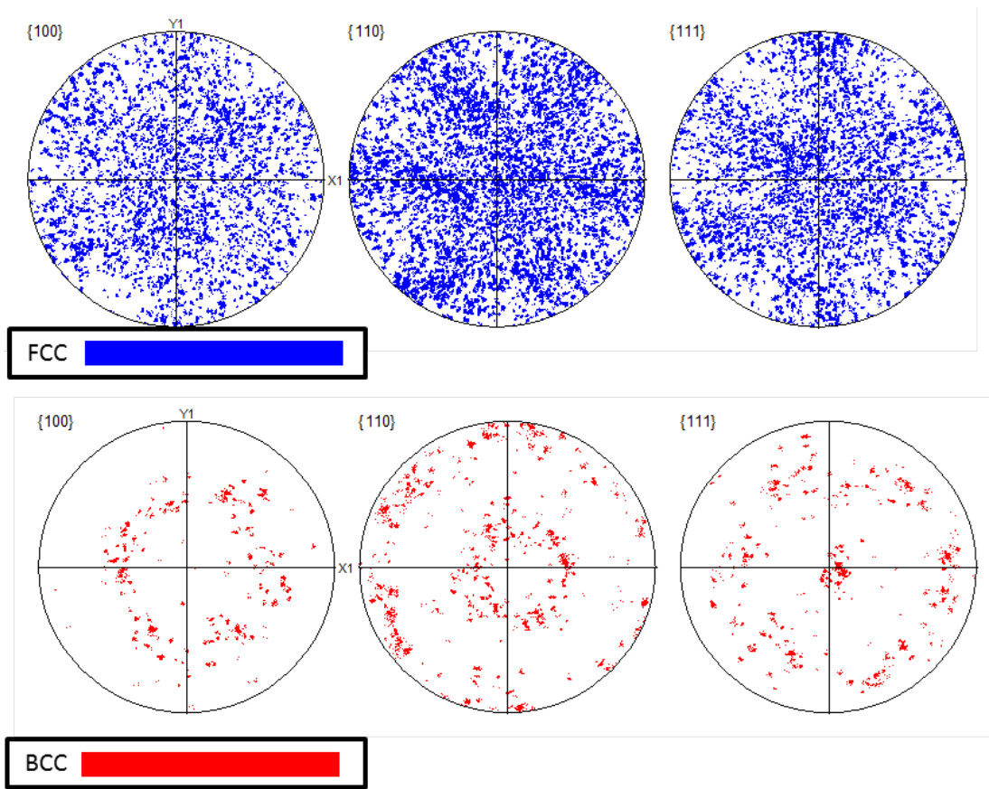
Figure 3.10: Pole figures of FCC and BCC grains in the base material.
