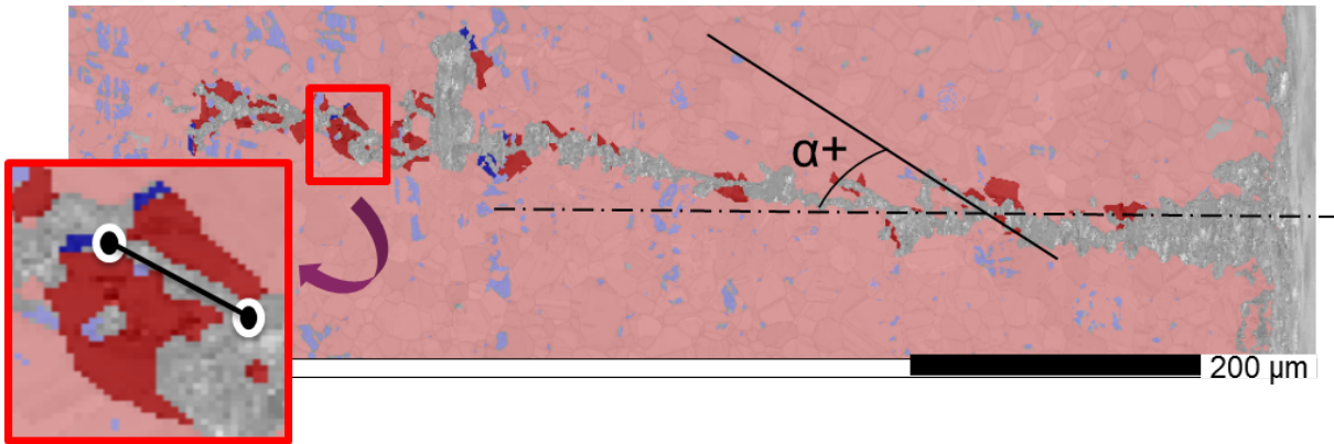
Figure 6.7: Isolation of TGSCC grains in EBSD map.
