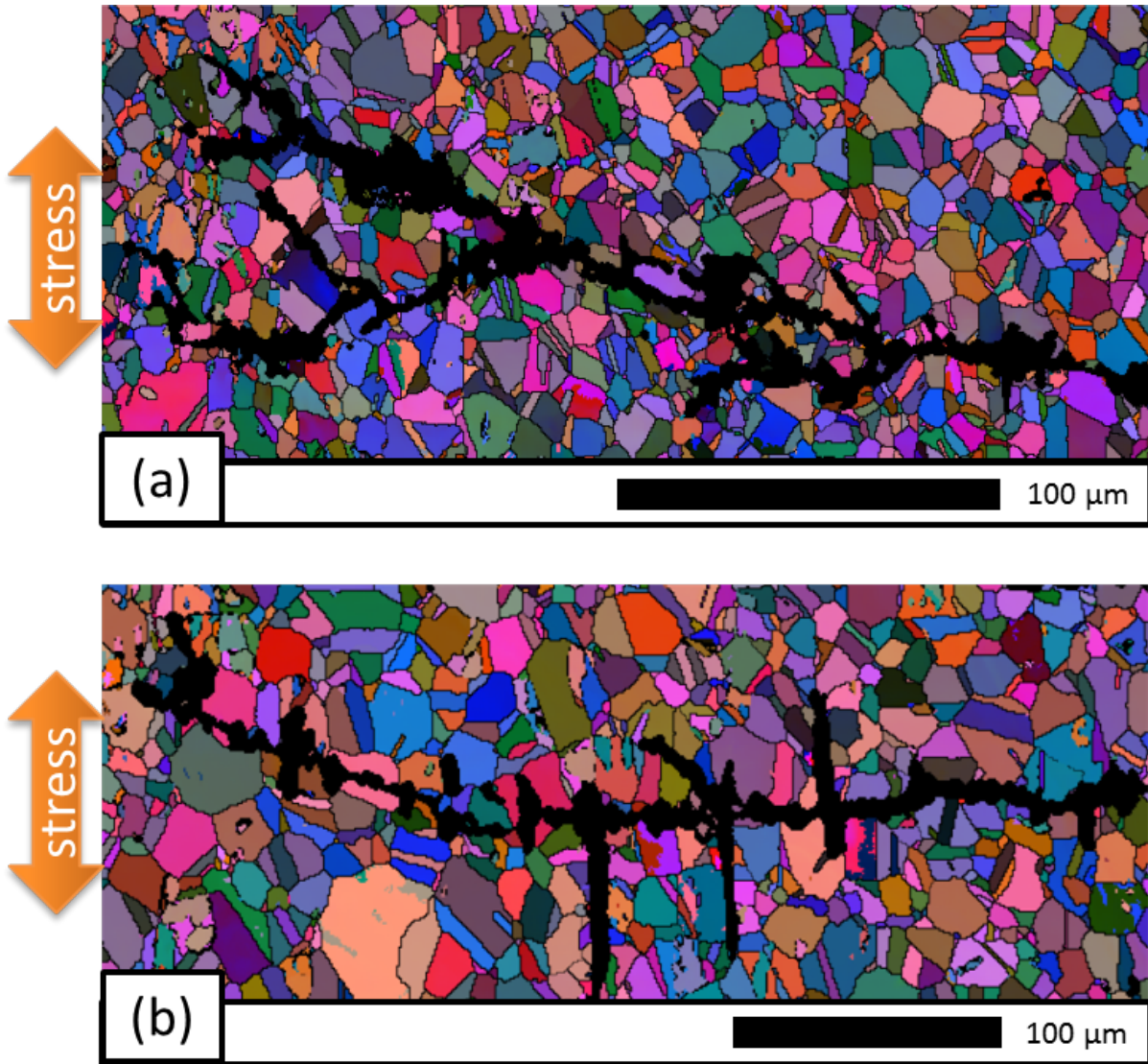
Figure 6.32: Cross-section EBSD maps of SCC test of \sigma = 250 MPa, after 21 days in 2 M \text{H}_2\text{SO}_4 + 2 M NaCl. (a) and (b) are two cracks selected for analysis.
