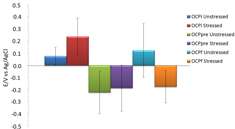
Figure 4.30: Illustration of OCP i , OCP pre , and OCP f values for polished stressed and unstressed samples in 5 M H 2 SO 4 + 0.05 M NaCl (flow cell).
