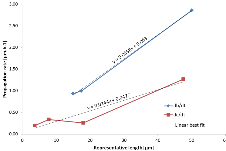
Figure 7.4: Illustrating the crack representative length along ( b ) and ( c ) direction vs the corresponding propagation rate.
