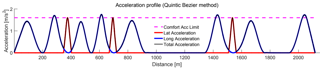
(b) Acceleration profile from the Quintic Bézier method
