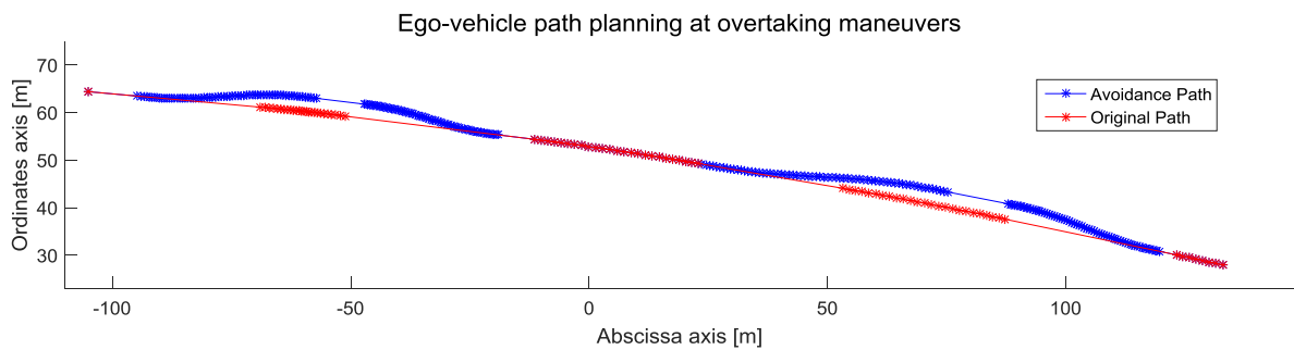
(b) Path planning for avoidance maneuvers.
