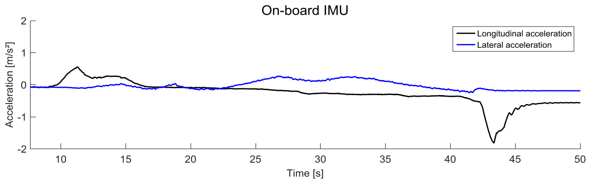
(c) Accelerations from the onboard IMU
