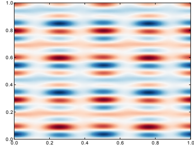
(e) BSE susceptibility, \omega = 14eV
