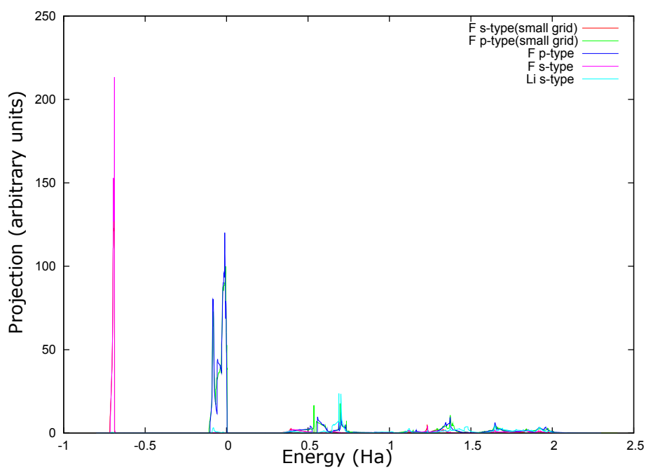
(b) Projected Density of States in the LDA approximation
