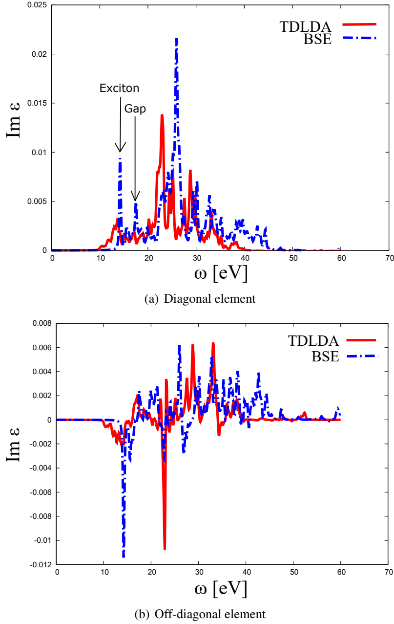
Figure 4.3 – Lithium Fluoride: comparison of diagonal and off-diagonal elements of \Im \epsilon for \mathbf{q} = (0, -0.25, -0.25) , \mathbf{G} = 0 , \mathbf{G}' = (1, 1, 1) , obtained using the BSE and TDLDA
