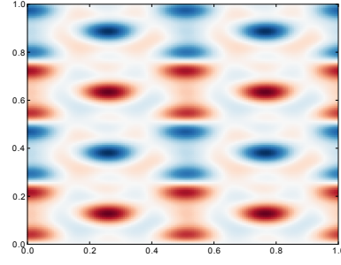
(b) RPA susceptibility, \omega = 25.6eV
