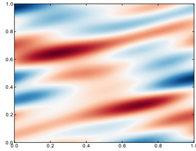
Figure 4.7 – Lithium Fluoride: the induced density, when V_{ext}(r) = \sum_q e^{iqr} is a superposition of 6 plane waves with different q -vectors, taken for 1 g and 1 g' . The response function used is the BSE one.
