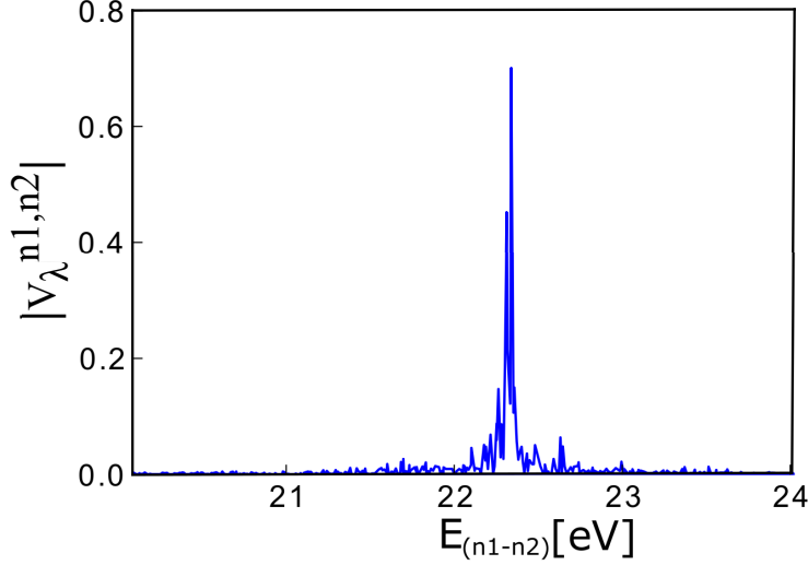
Figure 3.2 – The absolute value of coefficients V_{\lambda}^{n1,n2} in terms of the LDA energy E_{(n1-n2)} = \epsilon_{n2} - \epsilon_{n1} , for a transition given by its energy \epsilon_{\lambda} = 22.2 eV
