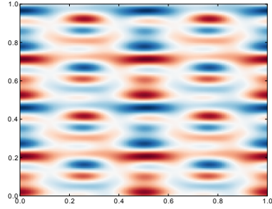
(c) TDLDA susceptibility, \omega = 14eV
