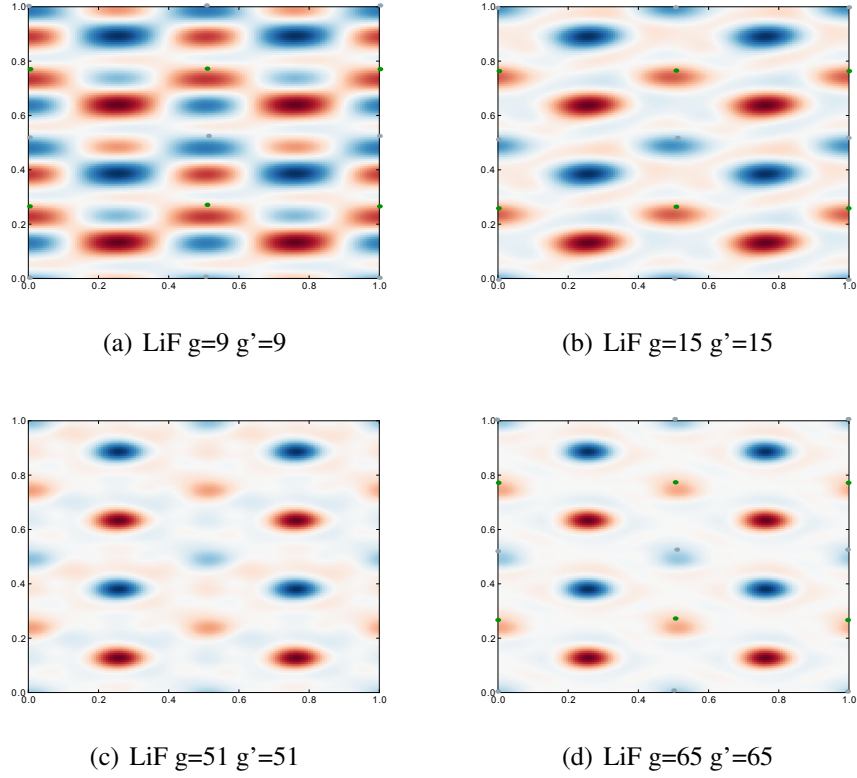
Figure 4.6 – Lithium Fluoride: number g of G vectors required to converge the induced charge density. V_{ext}(r) = e^{iq_0 r} \sum_{G'} e^{iG' r} is a superposition of g' plane wave. The response function used is the BSE one.
