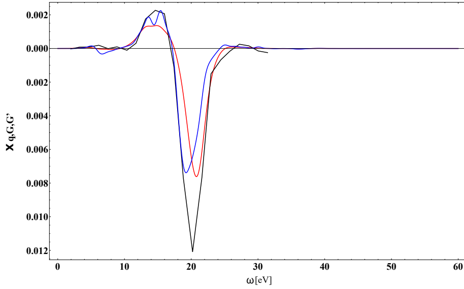
Figure 4.2 – Imaginary part of the off-diagonal element of the Bulk Silicon susceptibility obtained using the BSE (blue) and TDLA (red) compared to the experiment (black) from [104]. Here \mathbf{q}=0.5(1,1,1) , \mathbf{q}'=-0.5(1,1,1)
