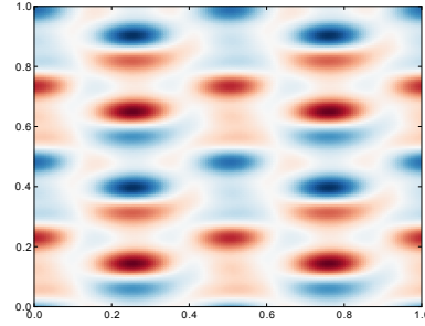
(f) BSE susceptibility, \omega = 25.6eV
