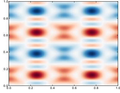
(a) RPA susceptibility, \omega = 14eV
