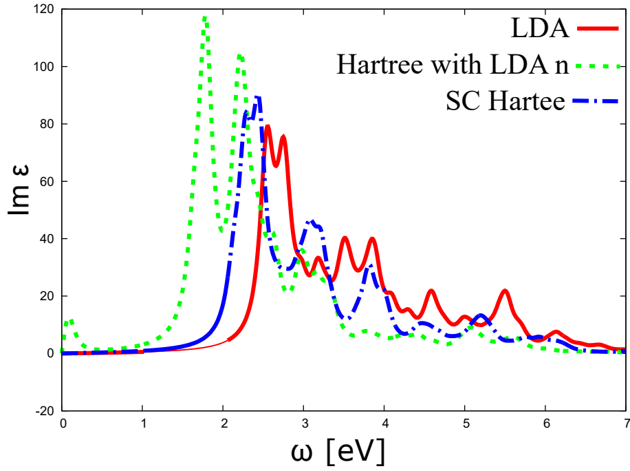
Figure 2.14 – Bulk Silicon \text{Im } \epsilon ( q=0 ) in the RPA approximation, including the local fields effect, obtained using the DP code, for LDA, self-consistent Hartree and Hartree with LDA density
