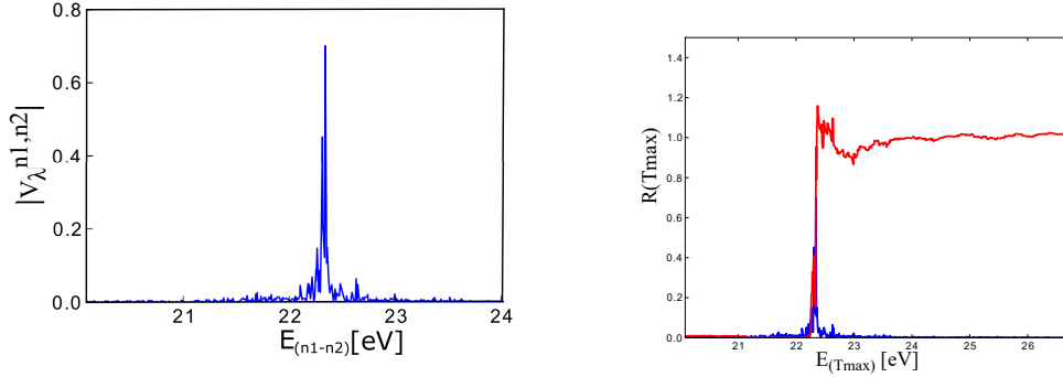
(a) Coefficients of an eigenvector of the effective hamiltonian in transition space, for a transition given by its energy \varepsilon_\lambda = 22.2 eV. (b) Coefficients of an eigenvector of the effective hamiltonian in transition space and partial sums of these coefficients Eqn. 3.21
