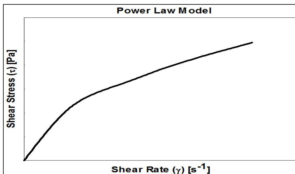
Figure 1.1.7: Flow curve for a Power Law fluid exhibiting N < 1
