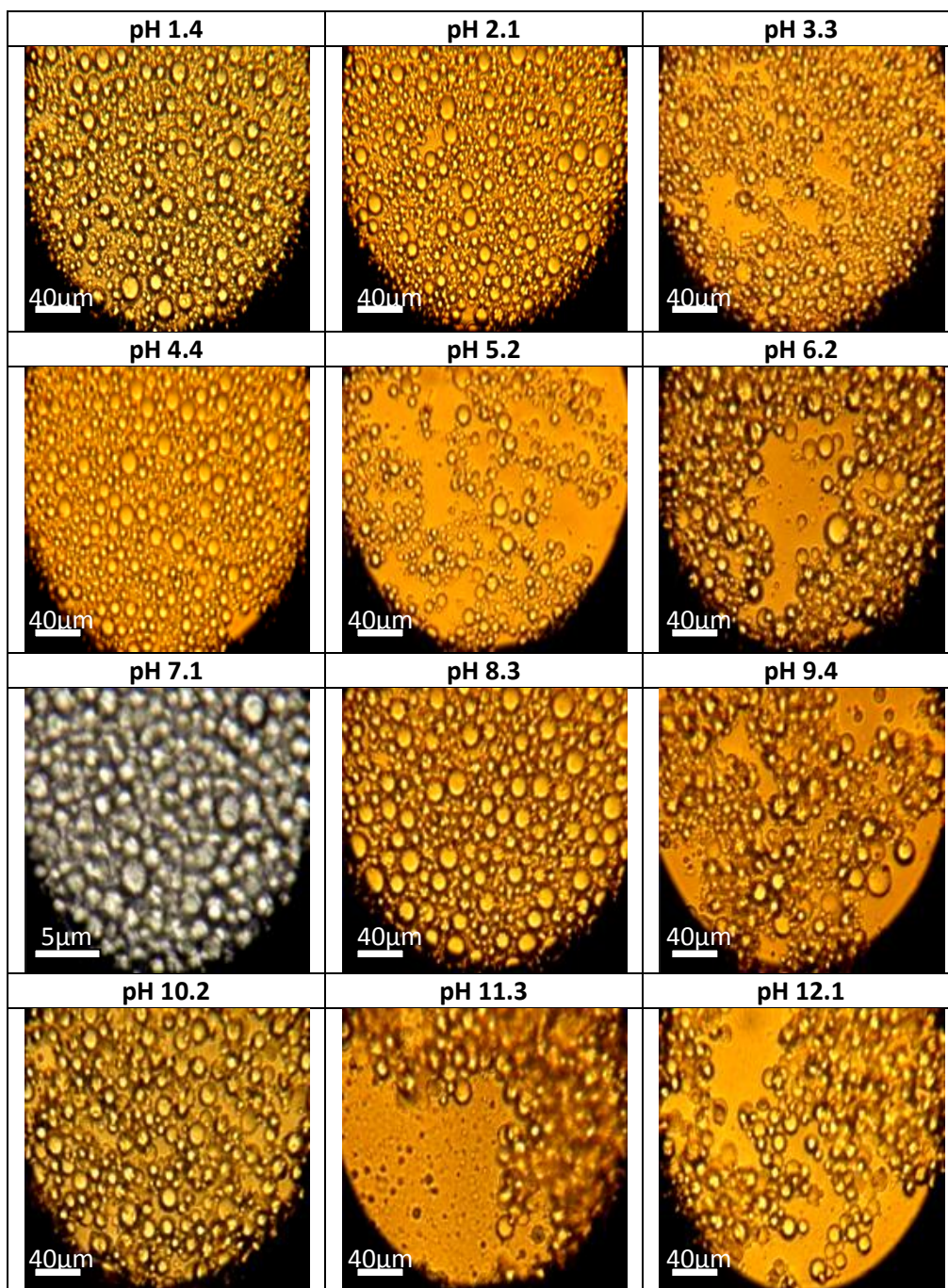
Figure 4.10: Effect of pH on the morphology of the WBMs prepared with AEROSIL R816
