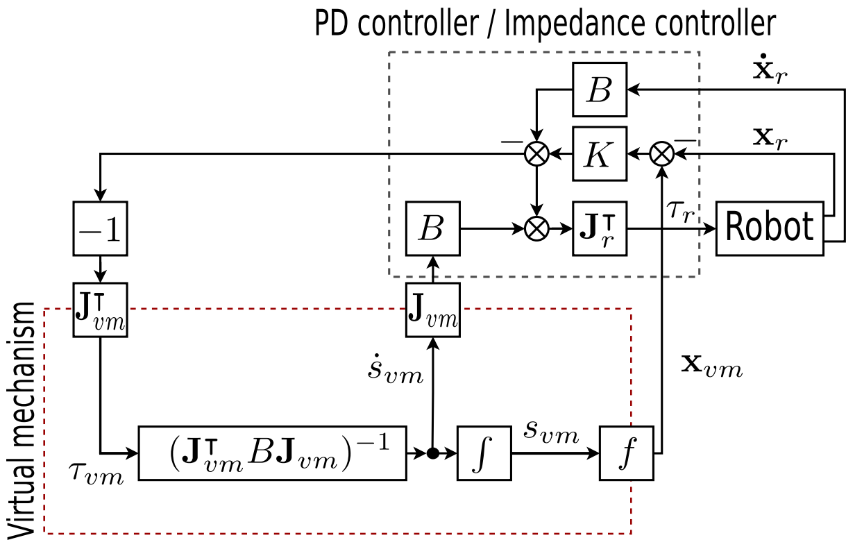
Figure 2.6: Control scheme for the virtual mechanism.
