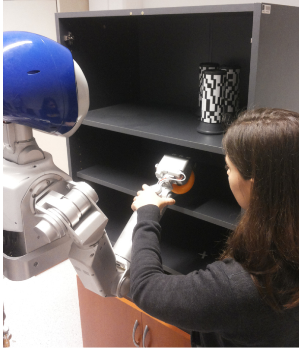
Figure 2.3: Image taken from the experiment conducted with the Meka robot at ENSTA-ParisTech (section 6.1). The task consisted in using virtual guides assistance to facilitate the placement of objects in a cupboard with shelves while avoiding collisions with them. Within the virtual guide formalization, it is important to distinguish between three participators: 1) the human operator, who exerts forces on the robot end-effector 2) the robot 3) the virtual mechanism, which constrains the movement of the robot.
