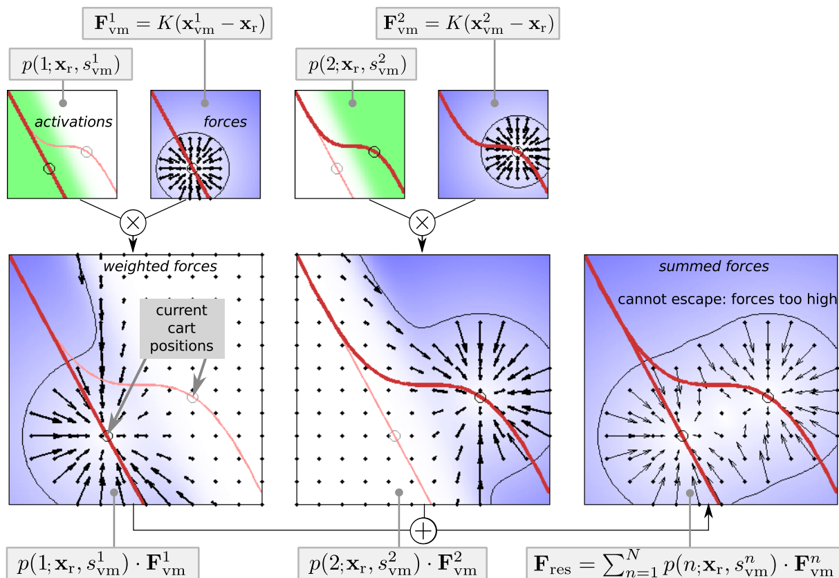
Figure 5.2: Scaling the forces of multiple virtual guides with probabilistic virtual mechanisms, using the first interaction mode (hard virtual guides). Each graph represents the value of one equation, depicted above/below the graphs. These illustrations are based on synthetic data. Since they represent a static snapshot, damping terms are omitted for simplicity.
