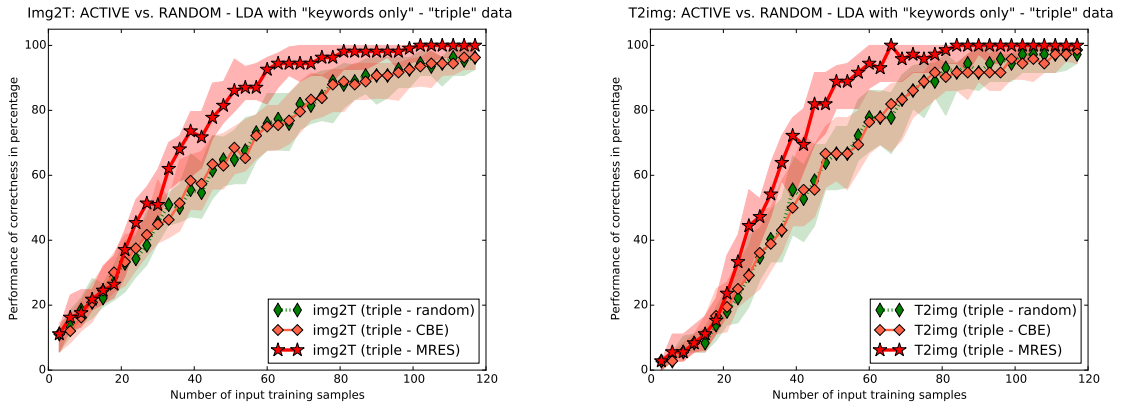
(c) “Img2T” results using KW&T from S-OBJ-C
