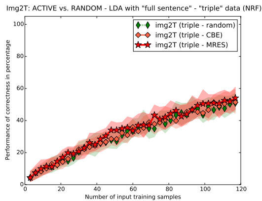
(e) “Img2T” results using FS&T from S-OBJ-C
