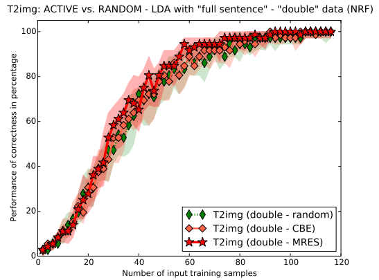
(d) “T2img” results using FS&D from S-OBJ-C
