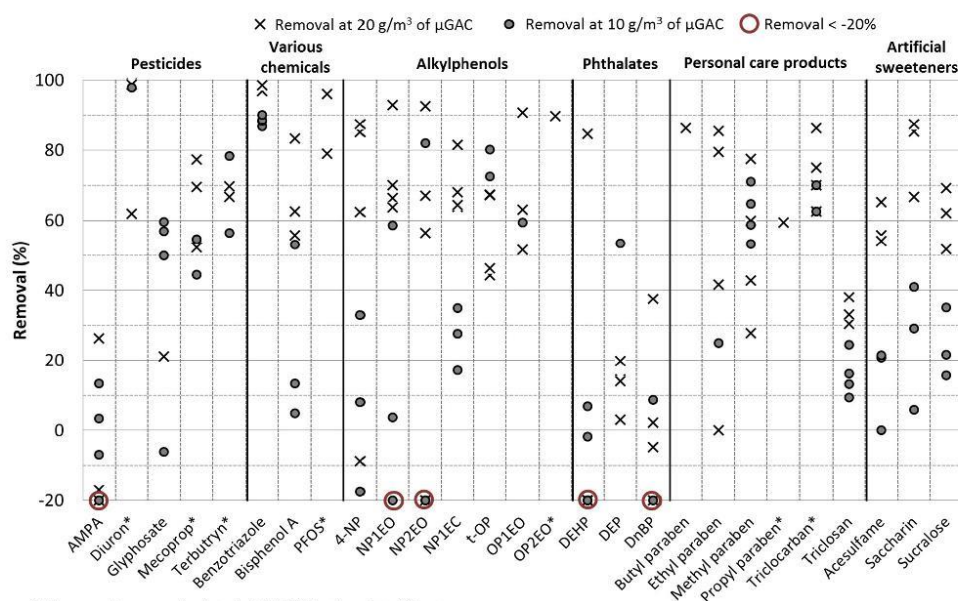
Fig. 4. Removals of the other emerging pollutants by the \mu GAC fluidized bed pilot in stabilized phase at 10 and 20 \text{g}_{\text{GAC}}/\text{m}^3 .
