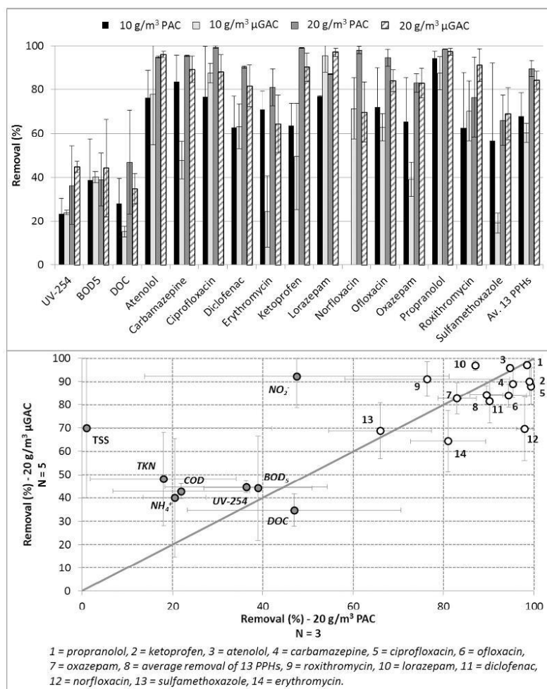
Fig. 5. Comparison of the fluidized bed performances operating with PAC and \mu GAC.
