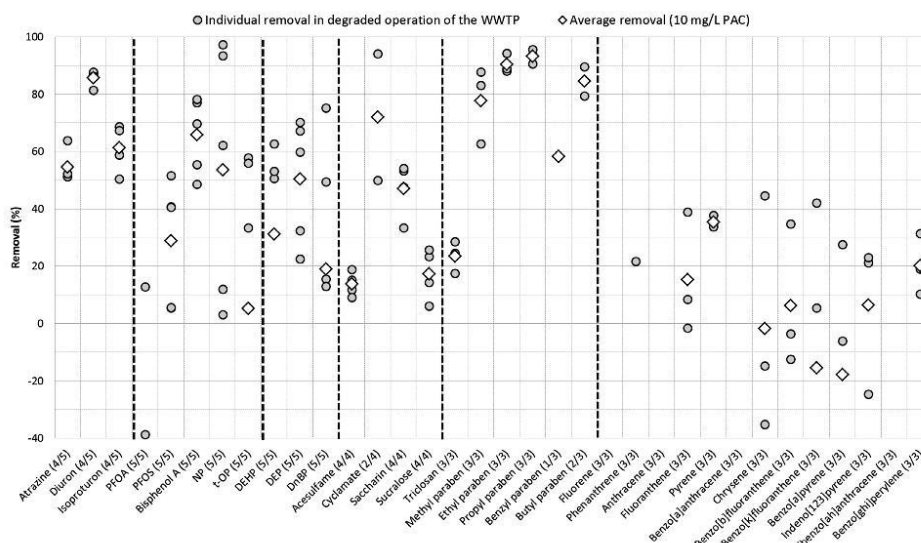
Fig. 3 – Removals of the other emerging micropollutants by PAC, in degraded configuration of the WWTP.
