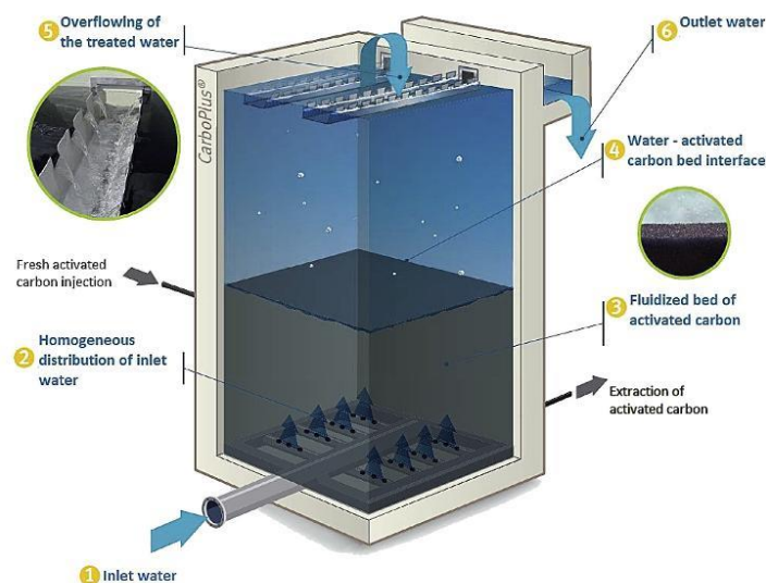
Fig. 1 – Layout of the 20 m 3 (5 m × 4 m 2 ) CarboPlus ® pilot (SAUR source).
