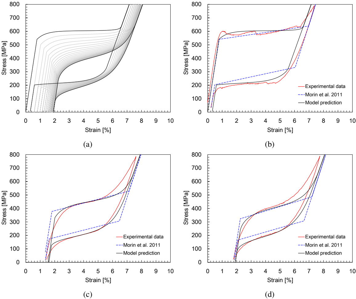
Figure 5.6 Cyclic stress-strain behavior of NiTi SMA at strain rate of 1 \times 10^{-3} s^{-1} : (a) evolution of stress-strain curves with the number of cycles, (b) comparison for the 1st cycle, (c) comparison for the 10th cycle, (d) comparison for the stabilized cycle.
