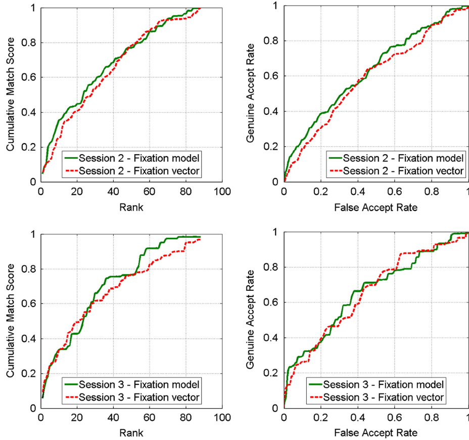
Figure 6.12: GAS performance.
