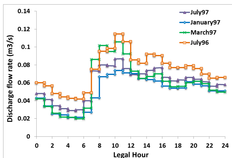
Figure 2-5: Daily cycle of dry weather flow at Marais sewer outfall measured during 4 campaigns
