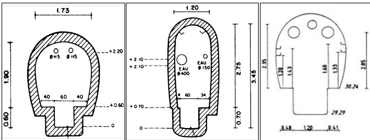
Figure 2-2: Typical sections of the main channels: (Left) SG, (Middle) VdT, (Right) Riv
