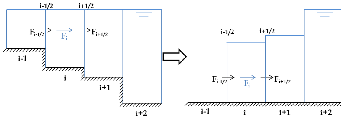
Figure 1-4: Illustration of the flow variables perceived by a non-well balanced scheme
