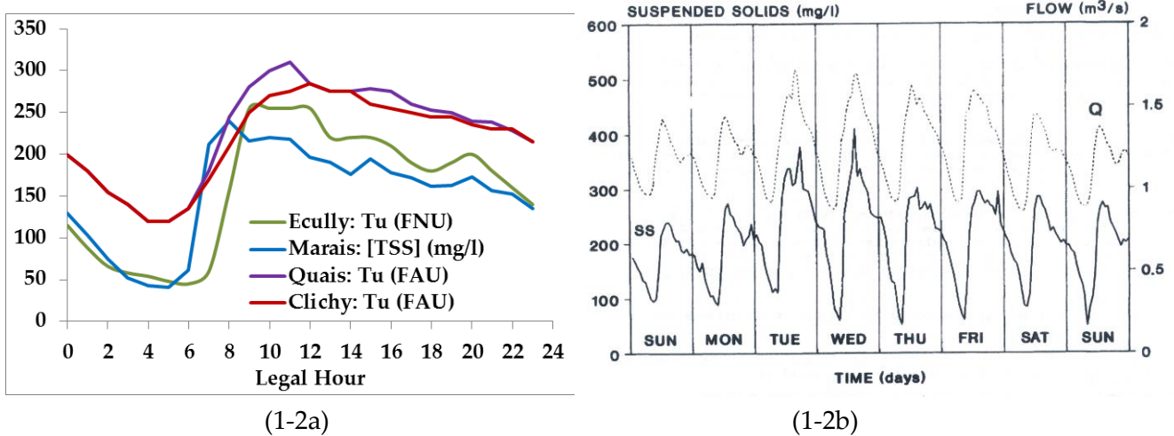
Figure 1-2: Daily cycle of wastewater TSS concentration at sewer outfalls during dry weather on: (1-2a) Ecully, Marais, Quais, and Clichy, (1-2b) Brussels main trunk
