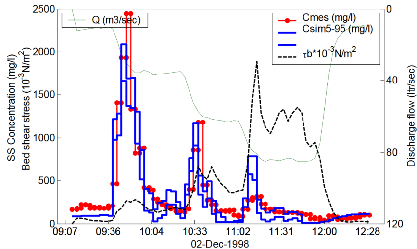
Figure 2-14: Measured and modelled suspended solid concentration versus time with 5-95% prediction interval obtained by MCMC calibration for the experiment of 02/12/1998 (Kanso et al., 2005)
