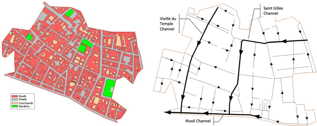
Figure 2-1: (Left) Surface distribution of the Marais site between roads, roofs, and courtyards; (Right) Principal and secondary channels in the Marais sewer system
