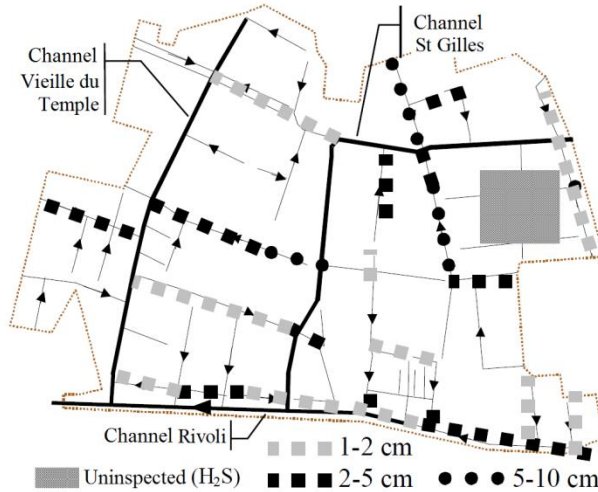
Figure 2-9: Coarse granular deposits observed on the upstream sewer of the Marais site
