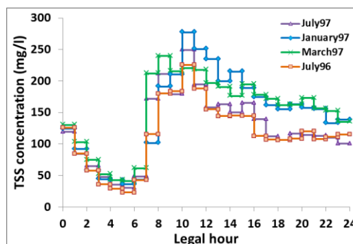
Figure 2-7: Daily cycle of dry weather TSS concentration at Marais sewer outfall measured during 4 campaigns
