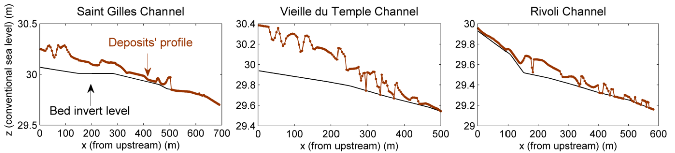
Figure 2-10: Bed invert level and coarse granular deposits profile on the three main channels of Marais catchment
