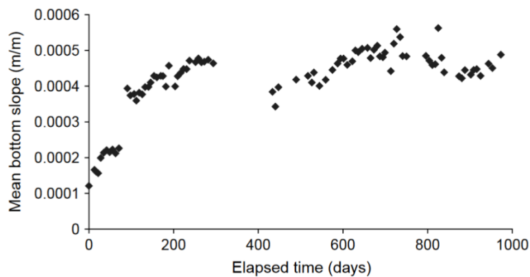
Figure 1-1: Asymptotic variation of the mean bottom slope in Lacassange sewer (Bertrand Krajewski et al., 2006)
