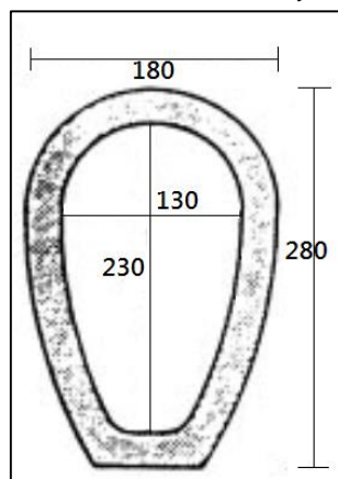
Figure 2-2: Typical sections of the main channels: (Left) SG, (Middle) VdT, (Right) Riv
