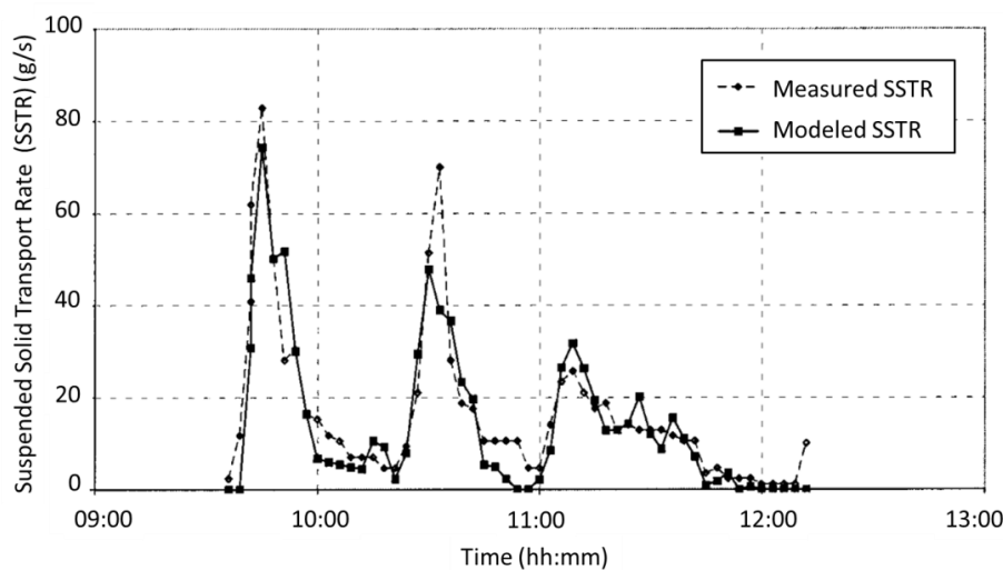
Figure 2-15: Measured and modelled suspended solid transport rate versus time for the deposits' parameters optimized using genetic algorithm to minimize the mean absolute error for the experiment of 02/12/1998 (Tait et al., 2003)
