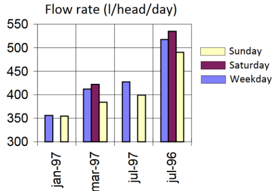
Figure 2-4: Comparison of average flow rate of dry weather flow at Marais sewer outfall between weekdays and weekends measured during 4 campaigns
