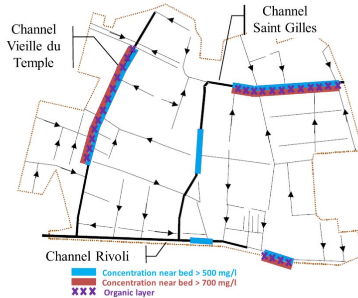
Figure 2-12: Organic layer cartographies obtained by Ahyerre (1999) (concentration near bed > 500 mg/l), and by Oms (2003) (using the endoscope)
