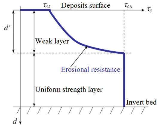
Figure 1-3: Variation of the erosional resistance of in-sewer sediments as described by (Skipworth et al., 1999)
