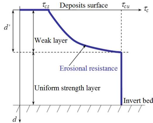
Figure 1-3: Variation of the erosional resistance of in-sewer sediments as described by (Skipworth et al., 1999)
