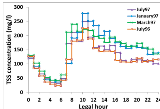
Figure 2-7: Daily cycle of dry weather TSS concentration at Marais sewer outfall measured during 4 campaigns
