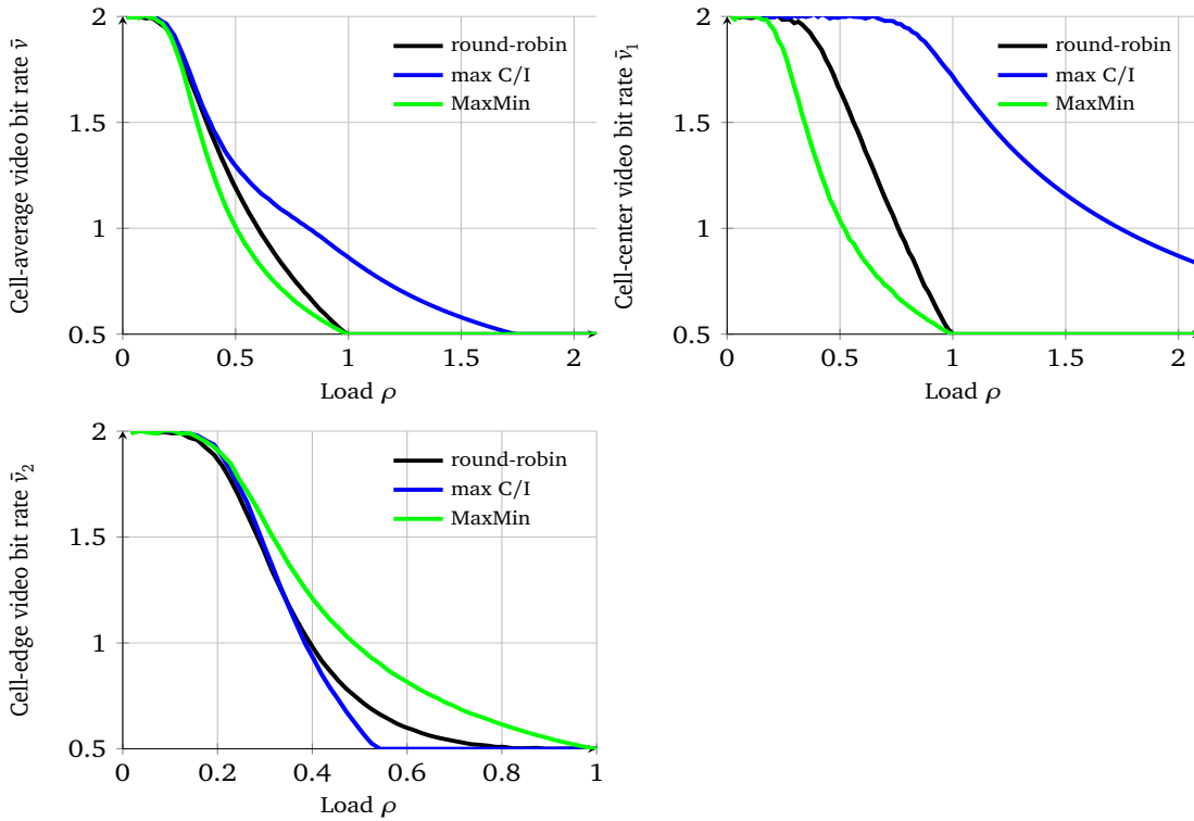
Figure II.23: Video bit rate performance for two regions without mobility.
