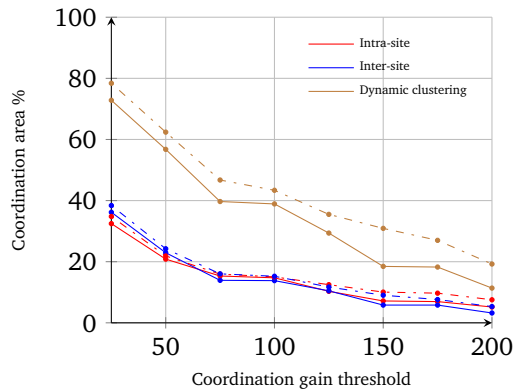
Figure III.47: Mean coordination area under different clustering methods with K_{max} = 2 (solid lines) and K_{max} = 3 (dashed lines).
