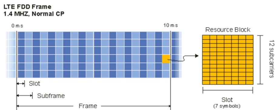
Figure I.3: LTE Frame.
