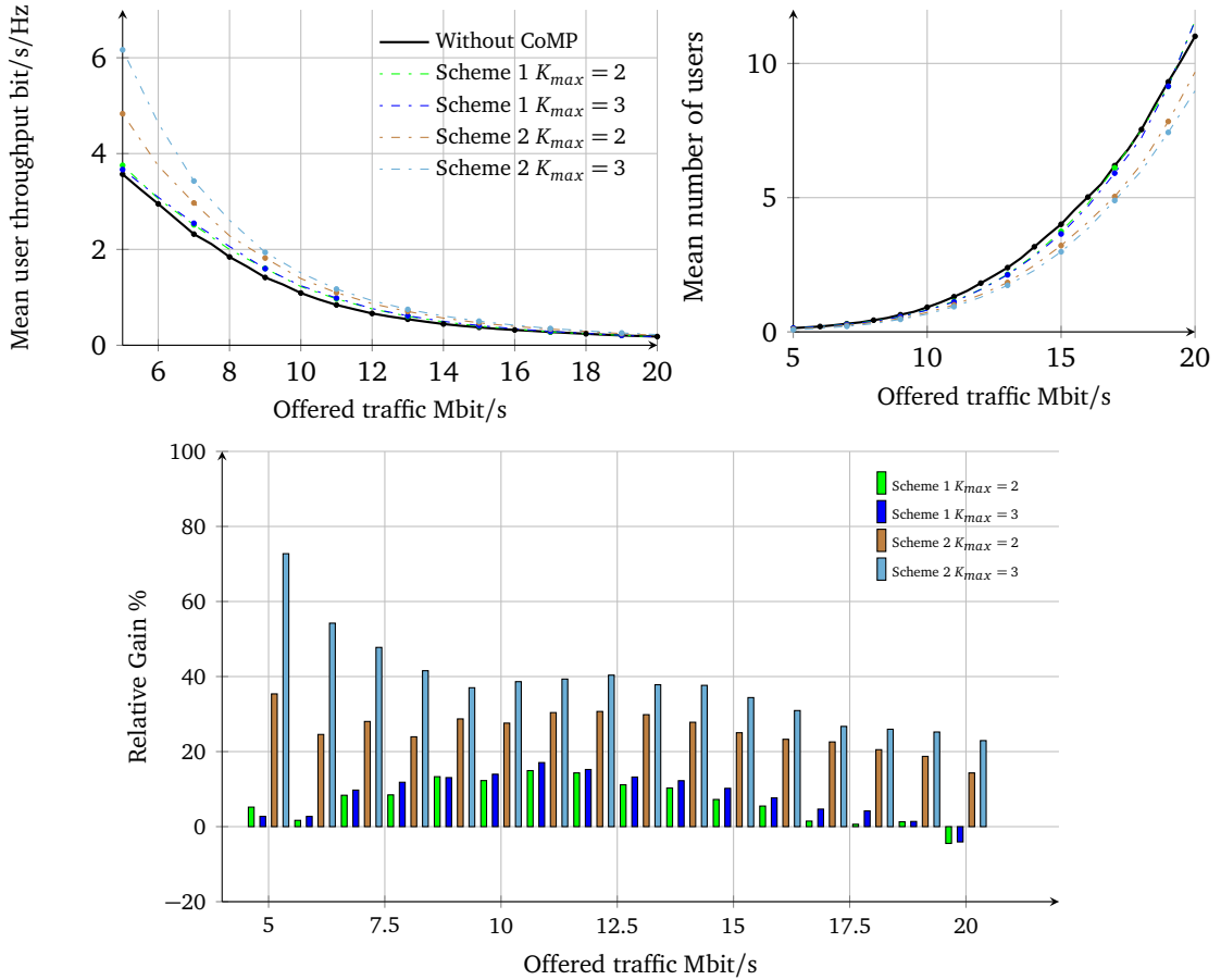
Figure III.53: Throughput performance obtained by system-level simulation for Intra-site gain-based JT under iterative scheduler.
