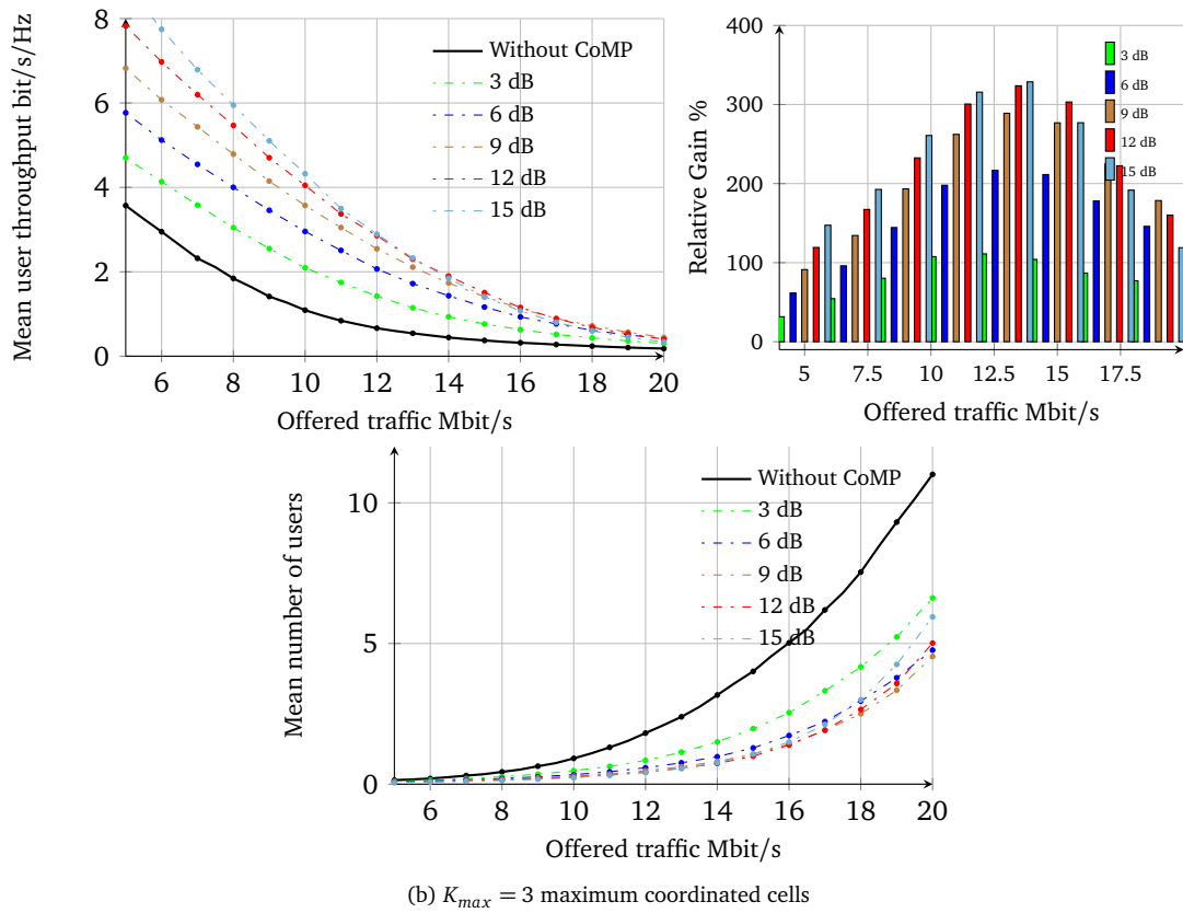
Figure III.40: Throughput performance obtained by system-level simulation for Dynamic clustering JT Scheme 2.
