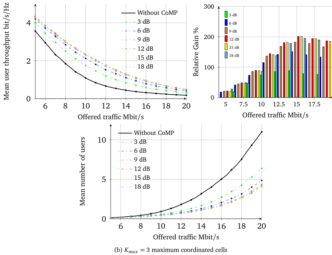
Figure III.67: Throughput performance obtained by system-level simulation for Dynamic clustering DPB.
