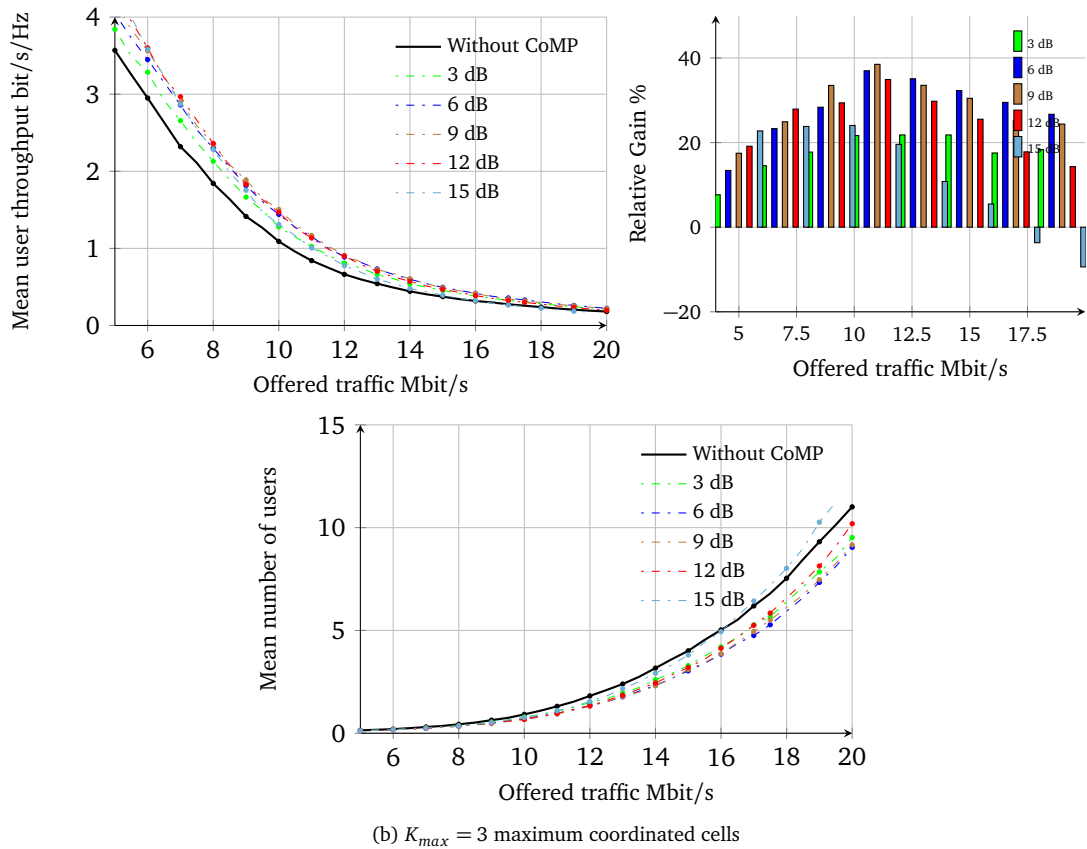
Figure III.34: Throughput performance obtained by system-level simulation for Intra-site JT Scheme 2.
