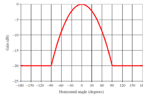
Figure 3: Antenna pattern for tri-sector cells
