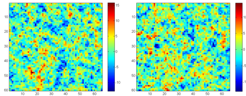
Figure 4: Shadowing map
