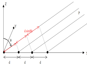
Figure IV.4: Uniform linear antenna array.
