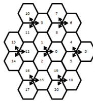
Figure 1: 7 tri-sector sites
