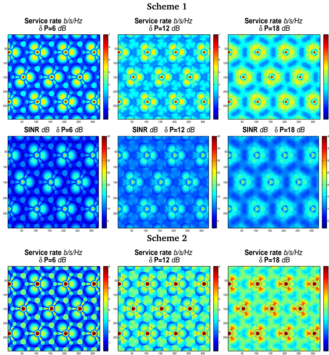
Figure III.15: Service rate and SINR maps for Dynamic clustering with K = 3 .
