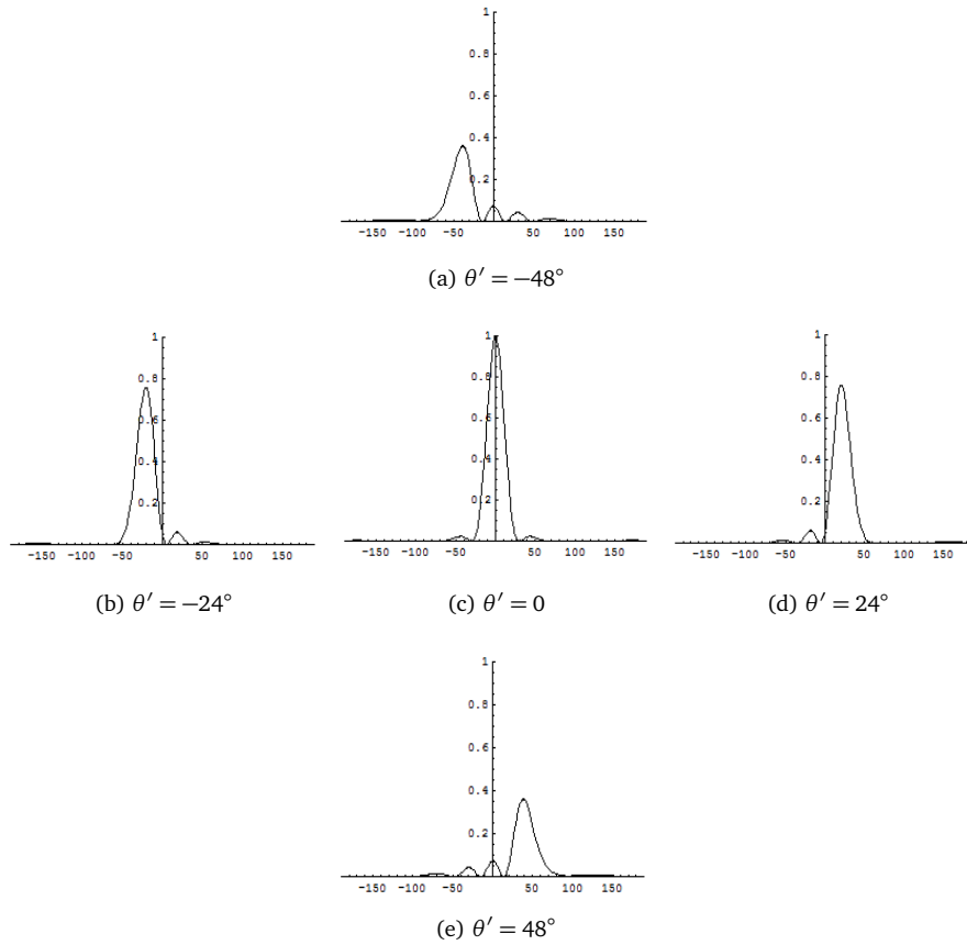
Figure IV.6: Normalized received power with respect to the direction of the user for N = 4 considering a codebook of size N_B = 5 .
