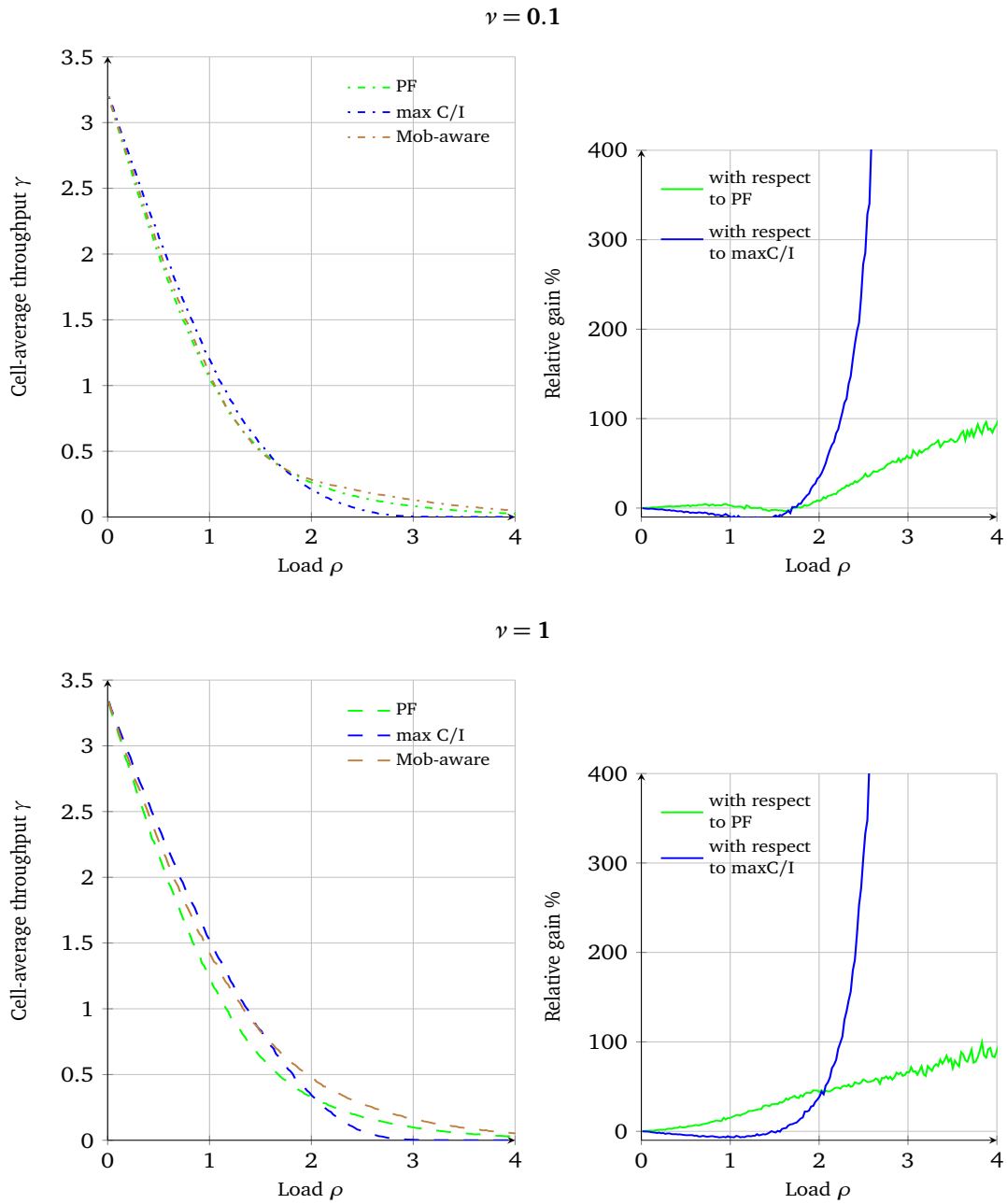
Figure II.14: Throughput performance for two regions with two classes of mobility and 50% mobile users.
