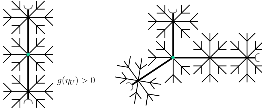
FIGURE 1. Star-shaped domains
