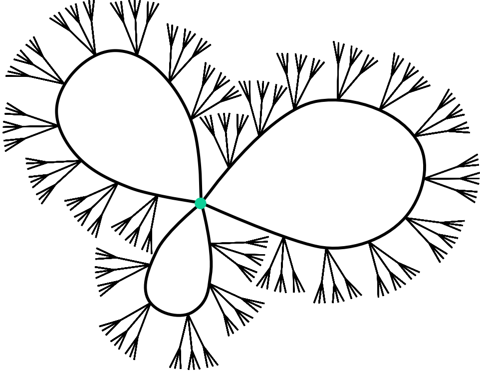
FIGURE 2. Curve with only one node and skeleton with first Betti number 3
