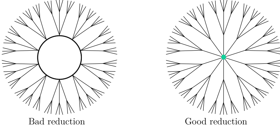
FIGURE 1. Elliptic curves
