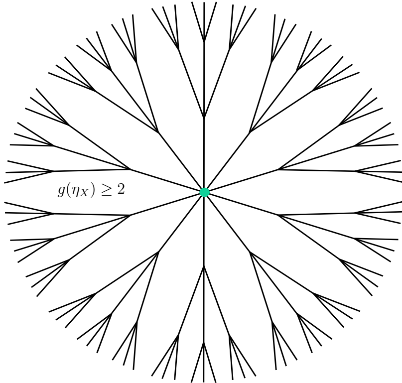
FIGURE 3. Curve with good reduction
