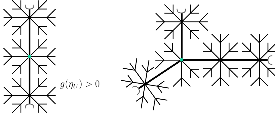
FIGURE 1. Star-shaped domains
