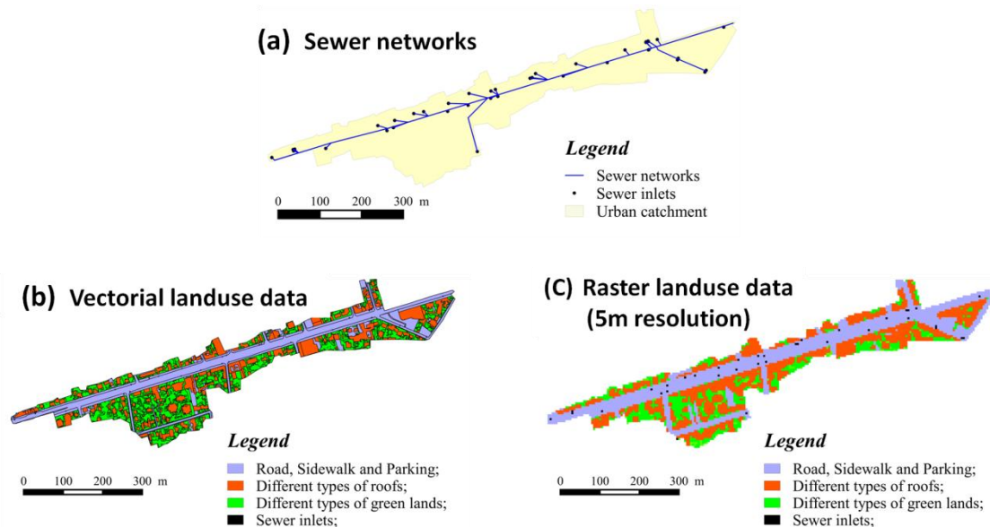
Figure 5. Input data for TRENNOE: (a) Separate stormwater sewer networks, (b) Vectorial landuse data; (c) Raster landuse data with 5m resolution.
