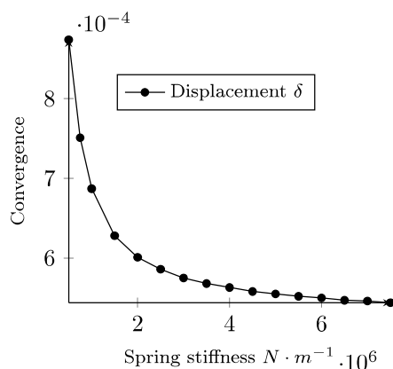
(a) Influence of spring stiffness on displacements
