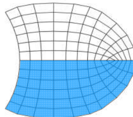
Figure 7.30 – Load distribution: the vertical load is applied to the blue area only.
