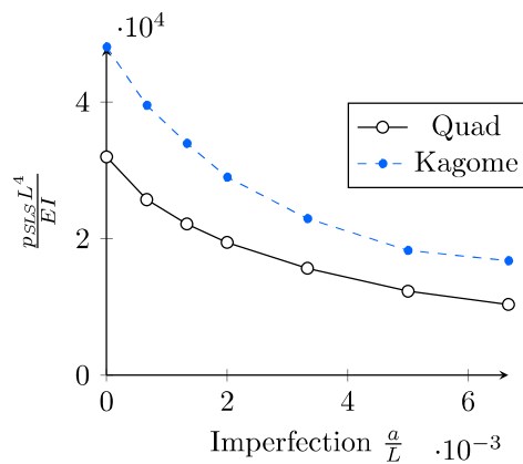
Figure 7.13 – Non-dimensional SLS load for Kagome and Quad gridshells
