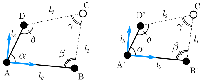
Figure 4.11 – Two quads related by a Combescure transformation.
