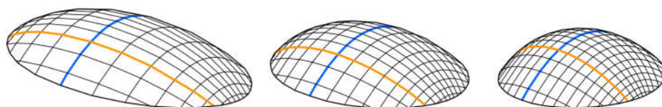
Figure 3.20 – Perspective view of the three domes as edge offset meshes.
