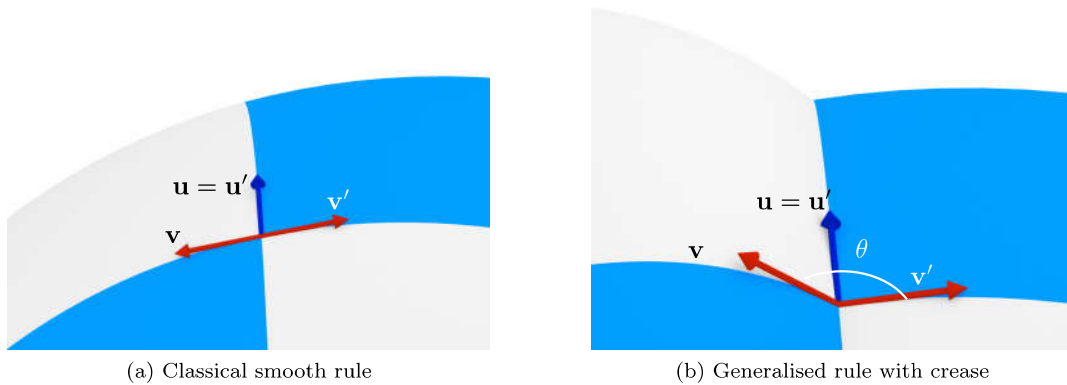
Figure 4.22 – Reflection rule for cyclidic patches.
