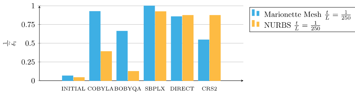
Figure 6.26 – Optimal values found for the minimisation of displacement under non-symmetrical load ( t/L = 1/250 ).
