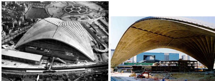
Figure 4.7 – The CNIT: a creased shell designed by Nicolas Esquillan
