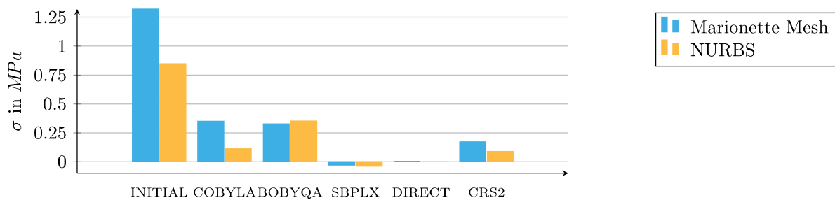
Figure 6.12 – Optimal values found for the minimisation of the maximal tensile stress under self-weight.
