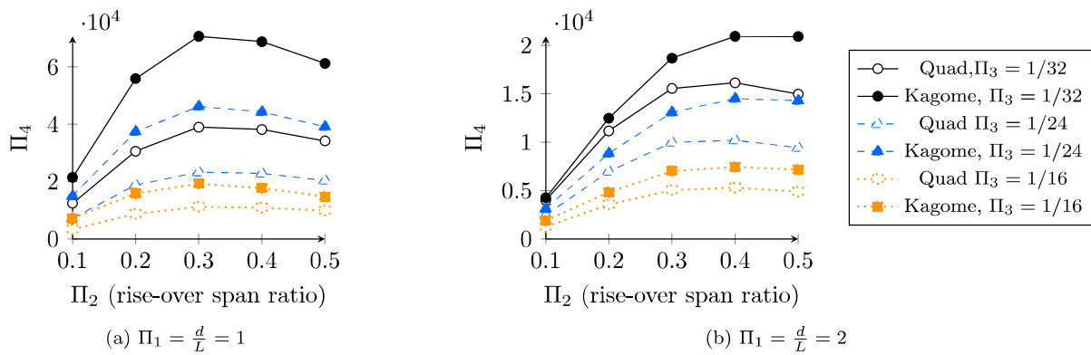
Figure 7.18 – Comparison of the buckling capacity of Kagome and quadrangular gridshells for the dome geometry.
