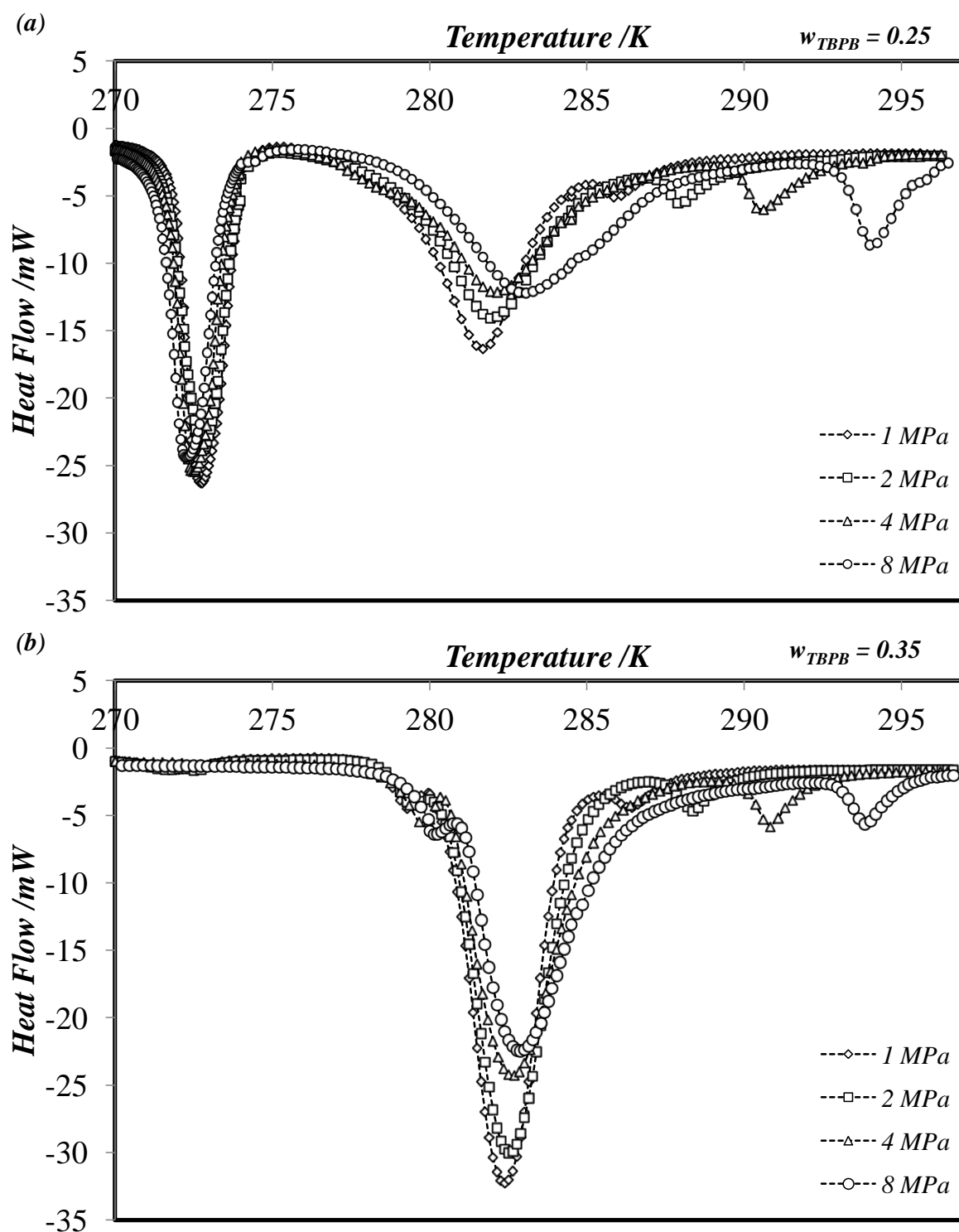
Figure 4.4. DSC curves from TBPB aqueous solutions in presence of \text{CH}_4 at heating rate of 0.5 \text{ K min}^{-1} : (a) w_{TBPB} = 0.25 ; (b) w_{TBPB} = 0.35 .
