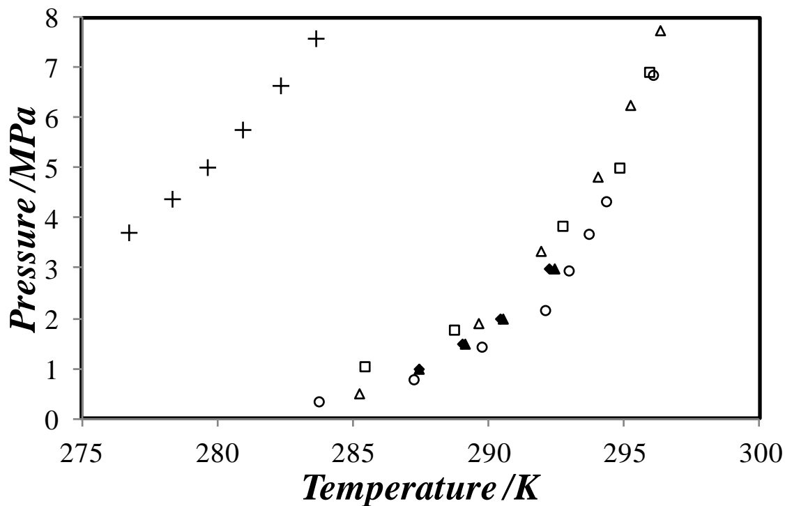
Figure 4.15. Equilibrium hydrate formation for CH 4 in pure water and for CH 4 in TBPO solution at w_{TBPO}=0.26 and 0.30 ; ◆, TBPO+CH 4 + H 2 O at w_{TBPO} = 0.26 , this study; ▲, TBPO+CH 4 + H 2 O at w_{TBPO} = 0.30 , this study; □, TBPO+CH 4 + H 2 O at w_{TBPO} = 0.26 , data from Cha et al. [121]; △, TBPO+CH 4 + H 2 O at w_{TBPO} = 0.30 , data from Cha et al. [121]; ○ TBPO+CH 4 + H 2 O at w_{TBPO} = 0.26 , data from Du et al. [122]; +, CH 4 + H 2 O, data from Adisasmito et al. [108].
