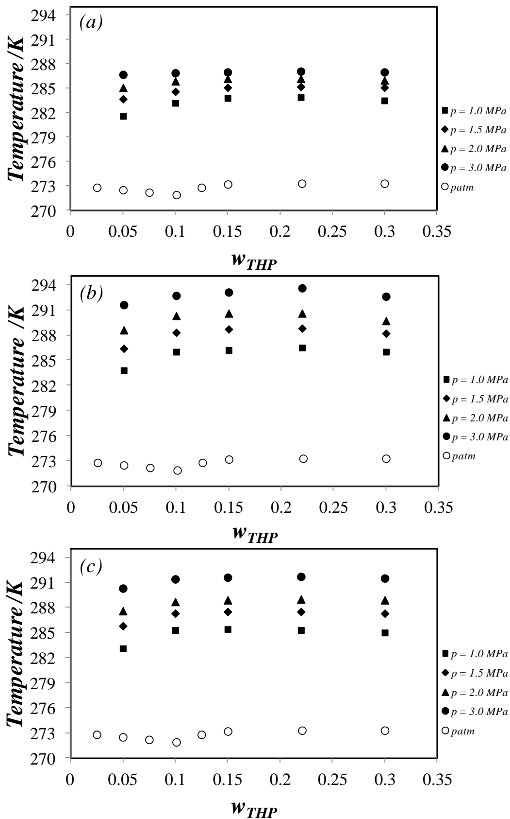
Figure 4.27. Temperature phase boundaries for single THP hydrate and THP/Gas gas hydrate: (a) \text{CO}_2 ; (b) \text{CH}_4 ; (c) \text{CO}_2+\text{CH}_4 (Gas mixture containing 40 \pm 1 mol.% of \text{CO}_2 ).
