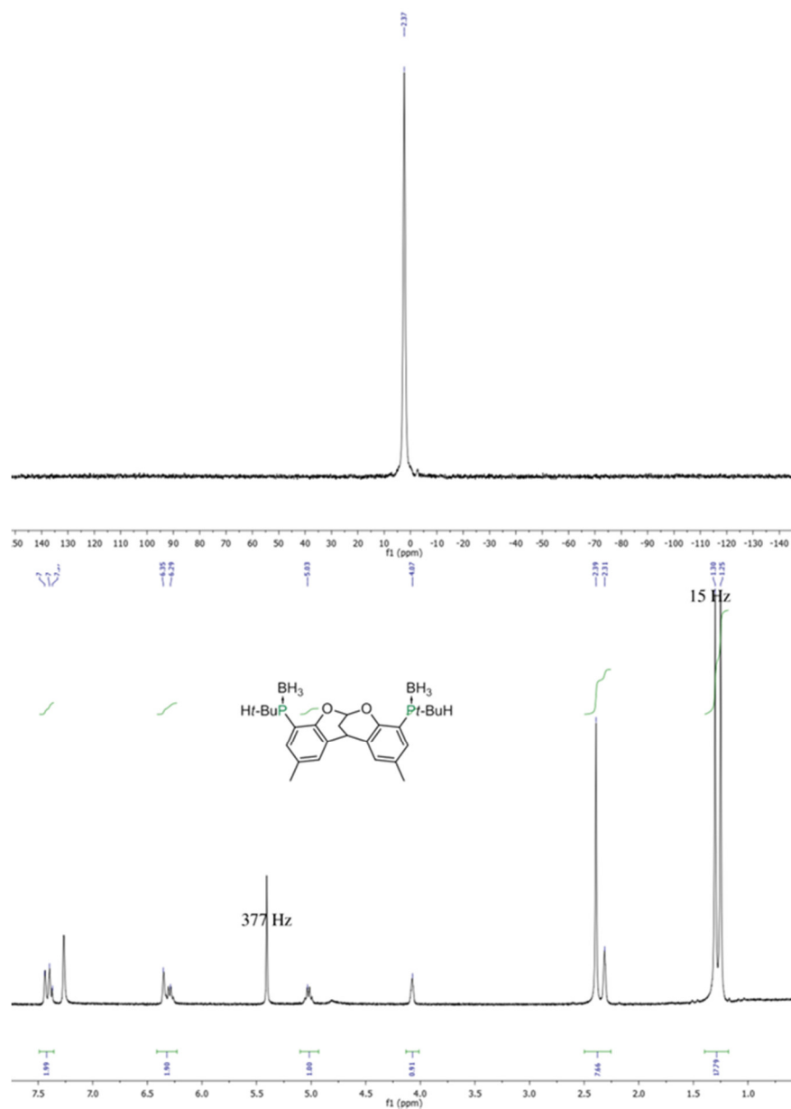
Figure 30: The ^{31}\text{P}\{^1\text{H}\} -NMR (above) and ^1\text{H} -NMR (below) spectra of the isolated form of meso -38c. A dichloromethane impurity is present.
