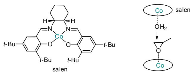
Figure 10: Enantioselective sandwich-type two center catalysis by Jacobsen et. al. 33
