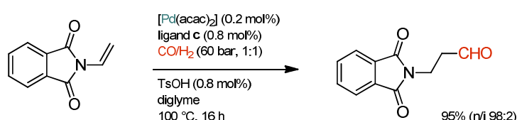
Scheme 66: N -selective palladium catalyzed hydroformylation of N -vinylphthalimide. 123,319
