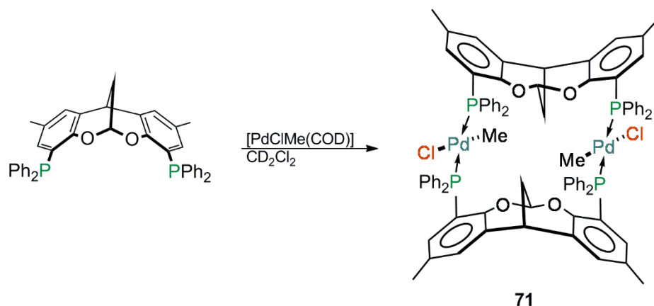
Scheme 56: Reaction of DBDOCphos with PdClMe(COD). a Study of solution spectra under the coordination conditions employed by Valbuena to obtain the \mu^2 -chloro complex 72 , showed the majority formation of the dimeric dipalladium trans -configured complex 71 .
