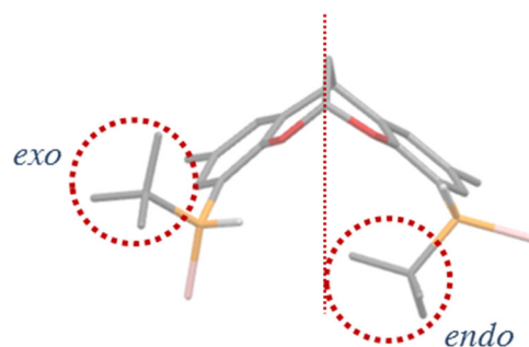
Figure 34: X-Ray structure of rac - 38c . Note the very different positions in space of the two BH 3 functionalities. Non-relevant hydrogen atoms have been hidden for the sake of clarity.
