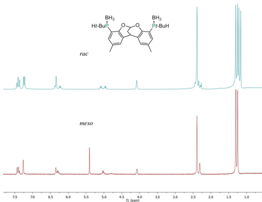
Figure 31: The ^1\text{H} -NMR spectra of the isolated rac -(above) and meso -(below) forms of 38c . The spectra show clearly only one P–H coupling in the meso form, indicating equivalent P-atoms.
