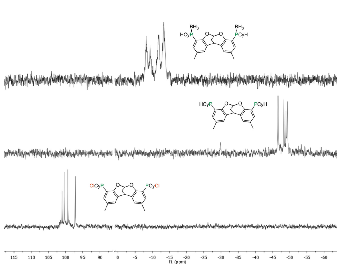
Figure 32: The ^{31}\text{P}\{^1\text{H}\} -NMR spectra demonstrate that using \text{R} = \text{Cy} the synthesis of pure secondary phosphine is applicable, in contrast to the t\text{-Bu} group the boronation step is not diastereoselective. The spectrum was cut between 90 and 0 ppm to amplify the resonances.
