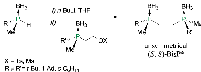
Scheme 29: Synthesis of unsymmetrical BisP* diphosphine by Imamoto et. al. 170
