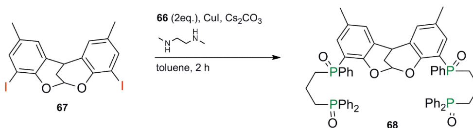
Scheme 54: A copper coupled approach to tetraphosphine tetraoxide 68 through reaction of 66 with DBDOC diiodide.
