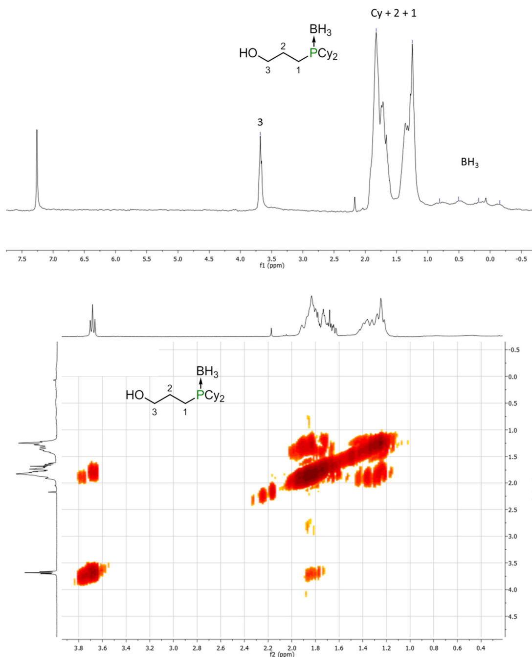
Figure 39: ^1\text{H-NMR} (in \text{CDCl}_3 ) on the top and the corresponding COSY ((in \text{CDCl}_3 )) the of the alcohol 45 with R = Cy.
