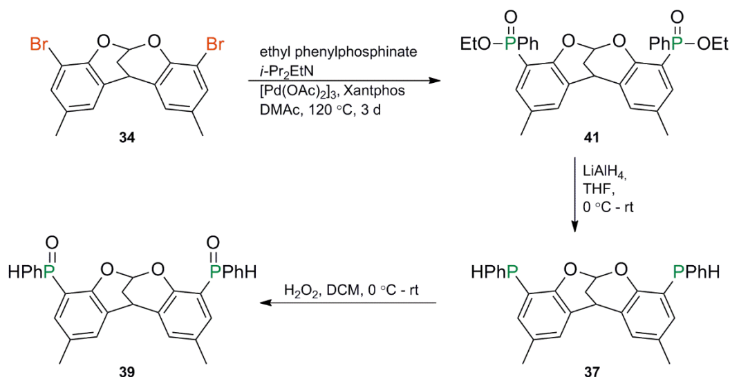
Scheme 27: Phosphorylation with ethyl phenylphosphinate. After palladium-catalyzed cross-coupling using \text{Pd}(\text{OAc})_2 as precursor and Xantphos as ligand in combination with the Hünig base in DMAc under reflux 3d, the backbone phosphinate products were subsequently reduced ( 37 ) and oxidized to give the stable secondary phosphine oxides ( 39 ). 158,186,206
