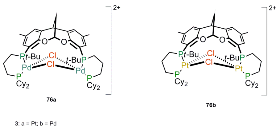
Figure 59: Coordination of tetraphosphines to PtCl_2 centres. Chloride-bridged possibilities can not be definitively eliminated by ^{31}P -NMR spectra.
