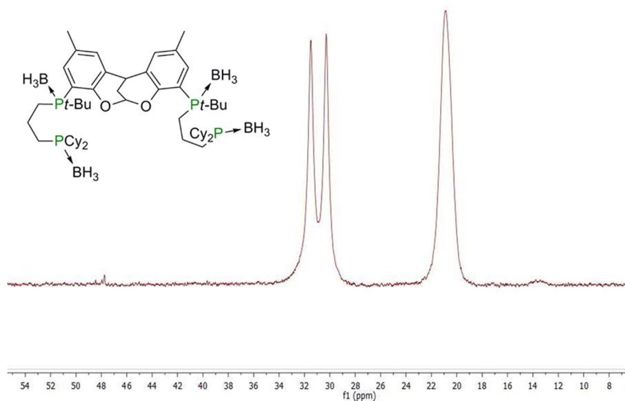
Figure 49: Synthesis of the tetraphosphine borane 58 ( \text{R} = \text{Cy} ) by nucleophilic substitution of metallated rac 38c . This synthesis using the dicyclohexanylphosphine- substituted side-arm showed 15 % formation of a sideproduct suspected to be the meso -form.
