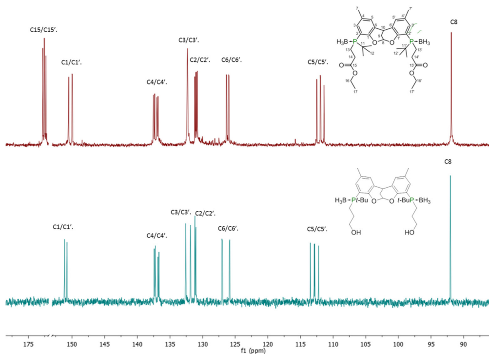
Figure 46: ^{13}\text{C}\{^1\text{H}\} -NMR spectra of the aromatic region of compounds 40 and 60 . The reduction of 40 with lithium aluminium hydride to 60 does not change the stereoinformation on the phosphorus atoms (only one resonance at C8 and the same pattern in the aromatic region), cut between C15 and C1.
