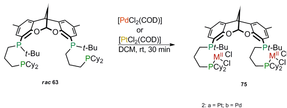
Scheme 59: Coordination of tetraphosphines to PtCl_2 centres. Treatment of the free rac -tetraphosphine ligand with 2 eq. [MCl_2(COD)] ( M = Pt, Pd ) probably leads to a homobimetallic complex with square planar 16 VE coordination ( d^8 ).
