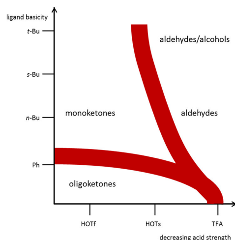
Figure 63: Schematic description of chemoselectivity as a function of ligand and acid properties. X-axis shows increasing pK_a : HOTf (- 5.1) < HOTs (- 2.7) < TFA (- 0.7) and Y-axis: Increasing ligand basicity: DPPP < DcBPP < DsBPP < DtBPP. 131
