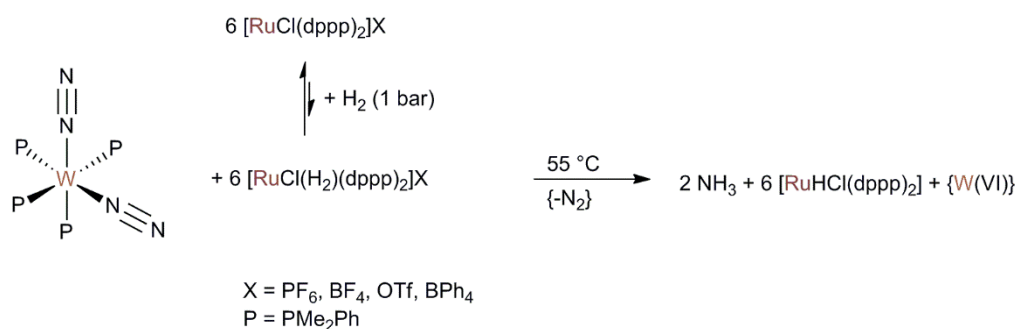
Scheme 2: The bimetallic reduction of N 2 to NH 3 at 55 °C and 1 atm developed by Morris and Hidai et. al. 39,41–44
