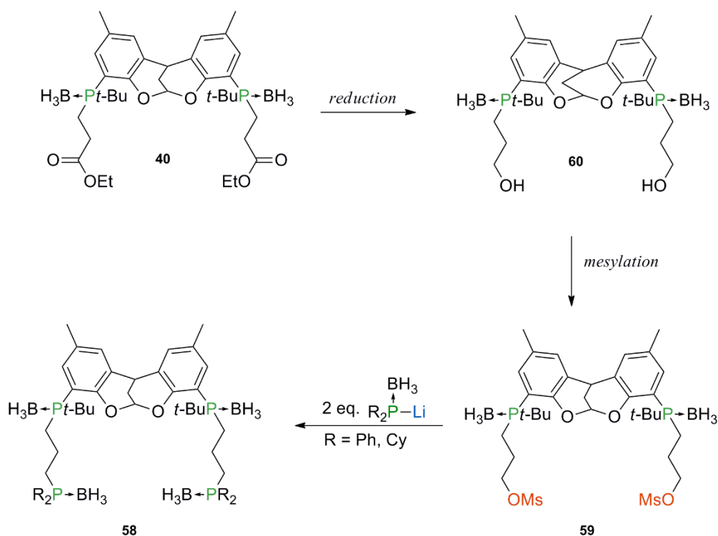
Scheme 40: Generation of tetraphosphine boranes rac 58 from rac 40 . The process involves reduction with lithium aluminium hydride ( 60 ), followed by mesylation with MsCl ( 59 ) and substitution of the backbone-side-arm ester 40 . All steps could be achieved with retention of configuration.
