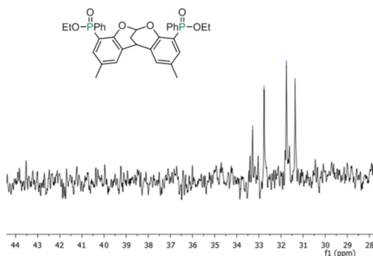
Figure 37: Phosphinylation of DBDOCB 2 . The ^{31}\text{P}\{^1\text{H}\} -NMR spectrum of 41 after work-up shows four resonances, which do not couple to protons, indicating the completion of the phosphorylation and suggesting the formation of the three diastereomers. 158,206
