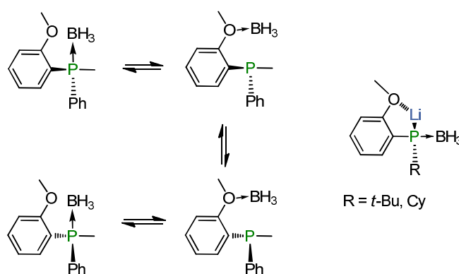
Scheme 37: Inversion of tertiary phosphine boranes bearing anisole substituents. This phenomenon, observed by Imamoto and co-workers, 167 occurs upon warming when with non-bulky groups are present. However bulky groups like t -Bu and Cy stabilize the alkali cation, minimizing or avoiding racemization. 176
