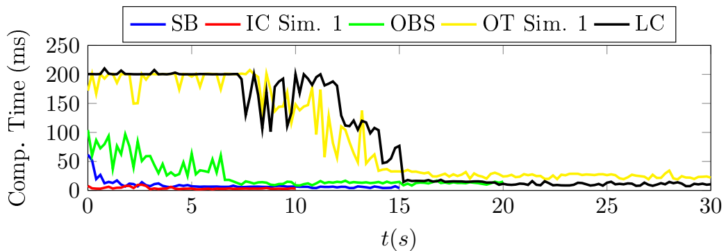
Figure 4.17: Statistics of computation time for different simulations
