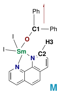
Figure 3.26: Label for the different atoms in M
