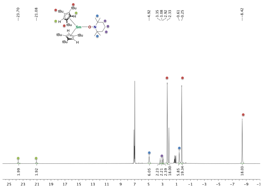
Figure 3.5: ^1\text{H} NMR of \text{Cp}_2^{\text{ttt}}\text{Sm}(\text{tempo}) in \text{toluene-d}_8
