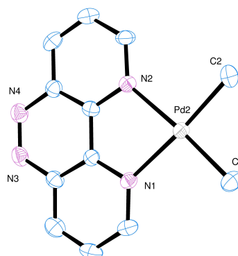
Figure 4.6: ORTEP of the X-Ray diffraction structure of (taphen)PdMe 2
