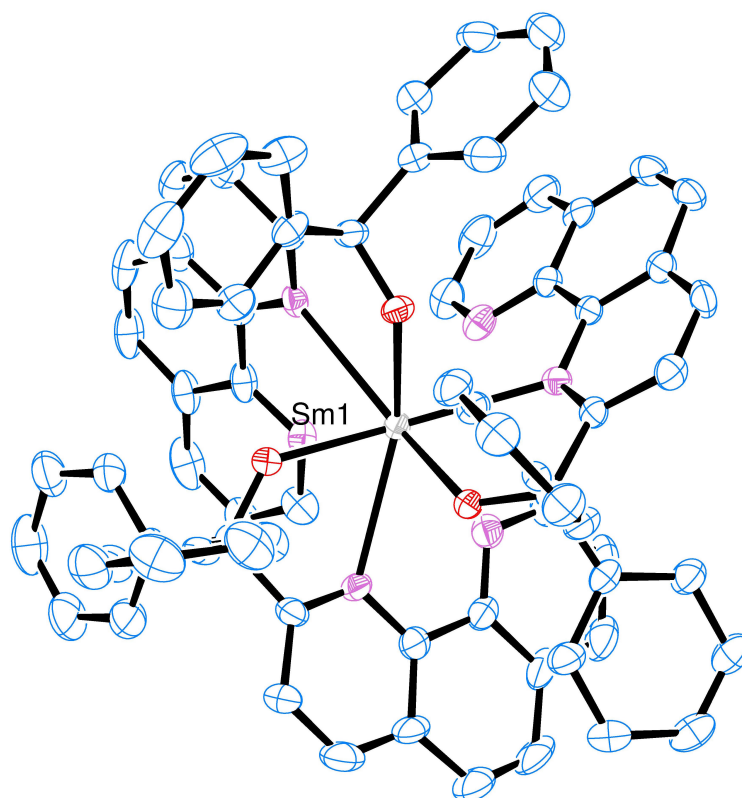
Figure 3.32: ORTEPs of the X-Ray structure of the intermediate structure, toluene molecules and the uncoordinated iodide were removed from the plots for clarity
