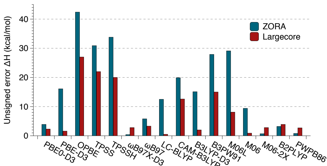
Figure 2.11: Unsigned error of \Delta H using LC-ECP and ZORA3 calculations with different density functionals
