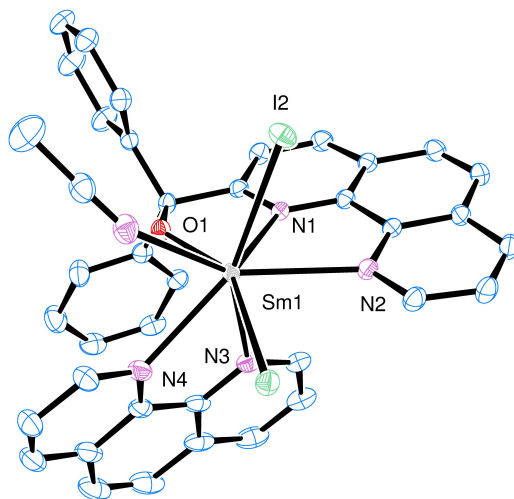
Figure 3.20: ORTEP of the X-Ray structure of \text{I}_2\text{Sm}(\text{phenO})(\text{MeCN})(\text{phen}) ; selected distances in angstroms: Sm – O 2.129(1), Sm – N1 2.544(2), Sm – N2 2.681(2), Sm – N3 2.606(2), Sm – N4 2.622(2), Sm – I1 3.2828(2), Sm – I2 3.1819(2)
