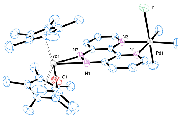
Figure 4.16: ORTEP of the X-Ray diffraction structure of \text{Yb}(\text{taphen})\text{PdMeI}
