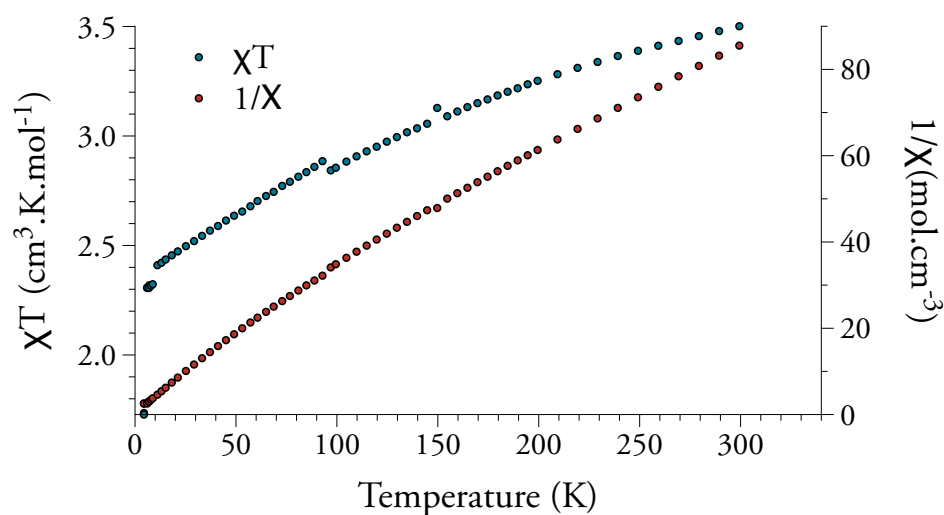
Figure 4.11: Temperature dependent magnetic data for \text{Yb}(\text{tapen})\text{Pd} from 5 K to 300 K at 0.5 T 1/\chi vs T is given as filled red dots, \chi T vs. T as filled blue dots
