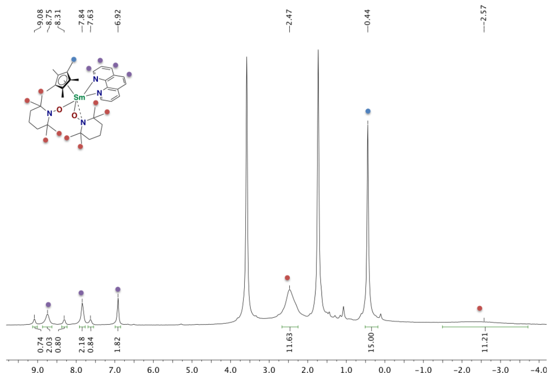
Figure 3.8: ^1\text{H} NMR of \text{Cp}^*\text{Sm}(\text{tempo})_2(\text{phen}) in \text{thf-d}_8
