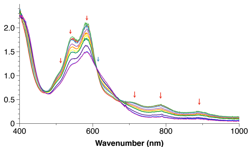
Figure 2.17: UV Visible spectrum of the equilibrium with \text{TmCp}_2^{\text{ttt}}\text{phen} at different temperature, green being 100°C and purple being 0°C; excitations of the monomer are indicated with red arrows and excitations of the dimer are indicated with blue arrows
