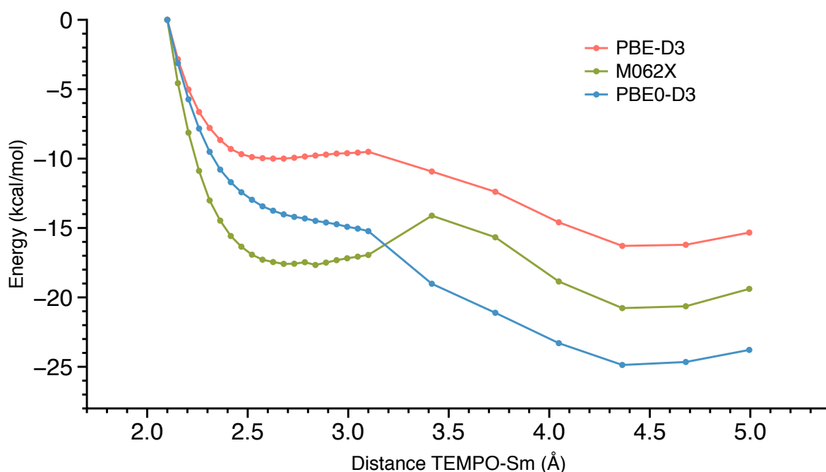
Figure 3.13: Potential energy surface of the reaction between tempo and \text{Cp}_2^*\text{Sm}(\text{phen}) , when changing the distance between the oxygen of tempo and the samarium ion from 2.0 and 5.0 Å using different density functionals
