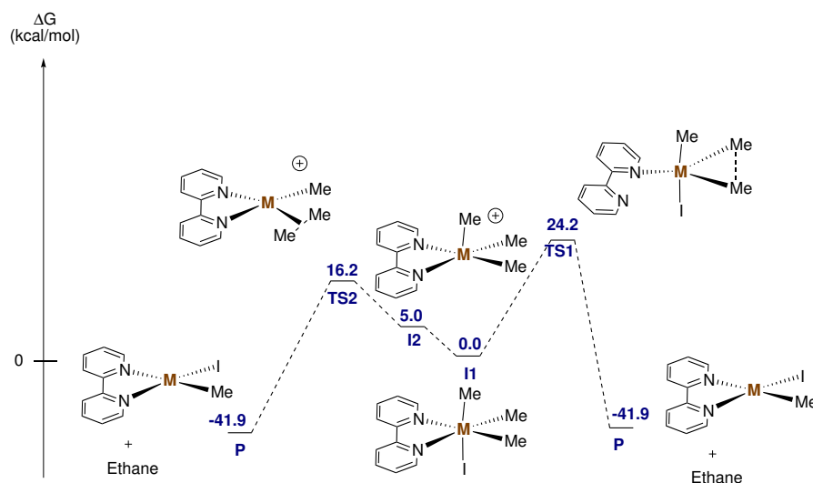
Figure 4.29: Mechanism for the reductive elimination of ethane upon oxidative addition of MeI on bipyridine palladium complexes in acetone
