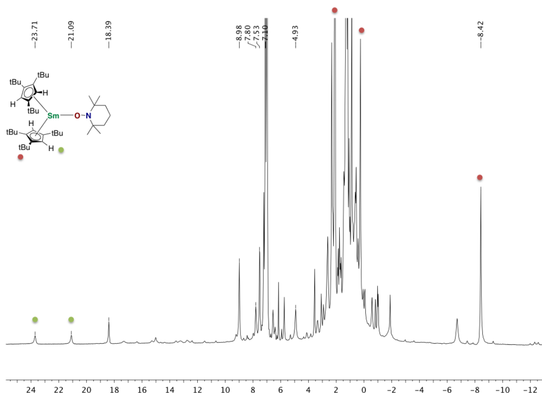
Figure 3.9: ^1\text{H} NMR of (\text{Cp}_2^{\text{ttd}}\text{Sm}(\text{phen}))_2 after addition of one equivalent of tempo in \text{toluene-d}_8
