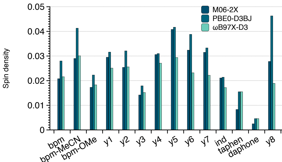
Figure 4.36: Löwdin spin density on the palladium for the radical complexes using different density functionals M06-2X, ωB97X-D3, PBE0-D3BJ
