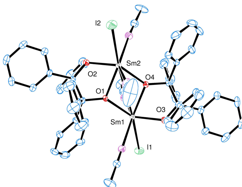
Figure 2.23: X-Ray Crystallographic structure of the dimer of benzophenone; significant bond distances: C-C (avg) 1.619(6) Å, Sm1-O3 2.132(3) Å, Sm1-O4 , Sm1-O1 2.317(3) Å, Sm1-O4 2.348(3) Å, Sm2-O2 2.132(3) Å, Sm2-O4 2.306(3)Å, Sm2-O1 2.338(3) Å, Sm-N (MeCN - avg) 2.557(3) Å, Sm-I (avg) 3.1475(3) Å
