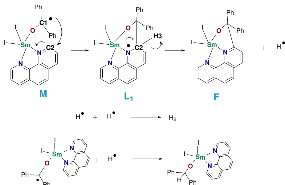
Figure 3.24: Mono-molecular mechanism
