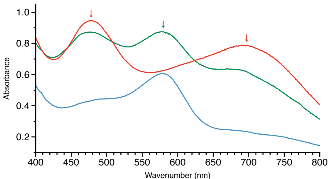
Figure 2.24: UV-visible spectrum in pyridine of I_2Sm(pyr) (red) at room temperature and of I_2Sm(bph) at room temperature (blue) and at 100 °C (green); green arrow indicates the peak of benzophenone ketyl radical and red arrows indicate the peak of pyridine radical
