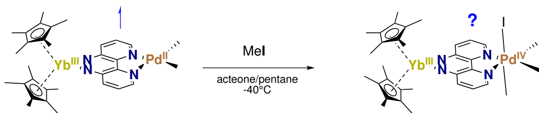
Figure 4.15: Scheme of the addition of MeI on \text{Yb}(\text{taphen})\text{Pd} forming \text{Yb}(\text{taphen})\text{PdMeI}
