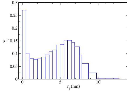
Figure 10.19: Regularized pore size distribution based from the experimental isotherm in Fig. 10.16.
