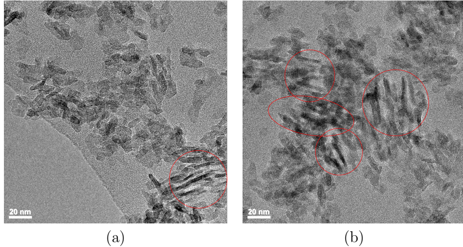
Figure 8.6: TEM image of crushed powder of mesoporous alumina. Local alignments are encircled in red.
