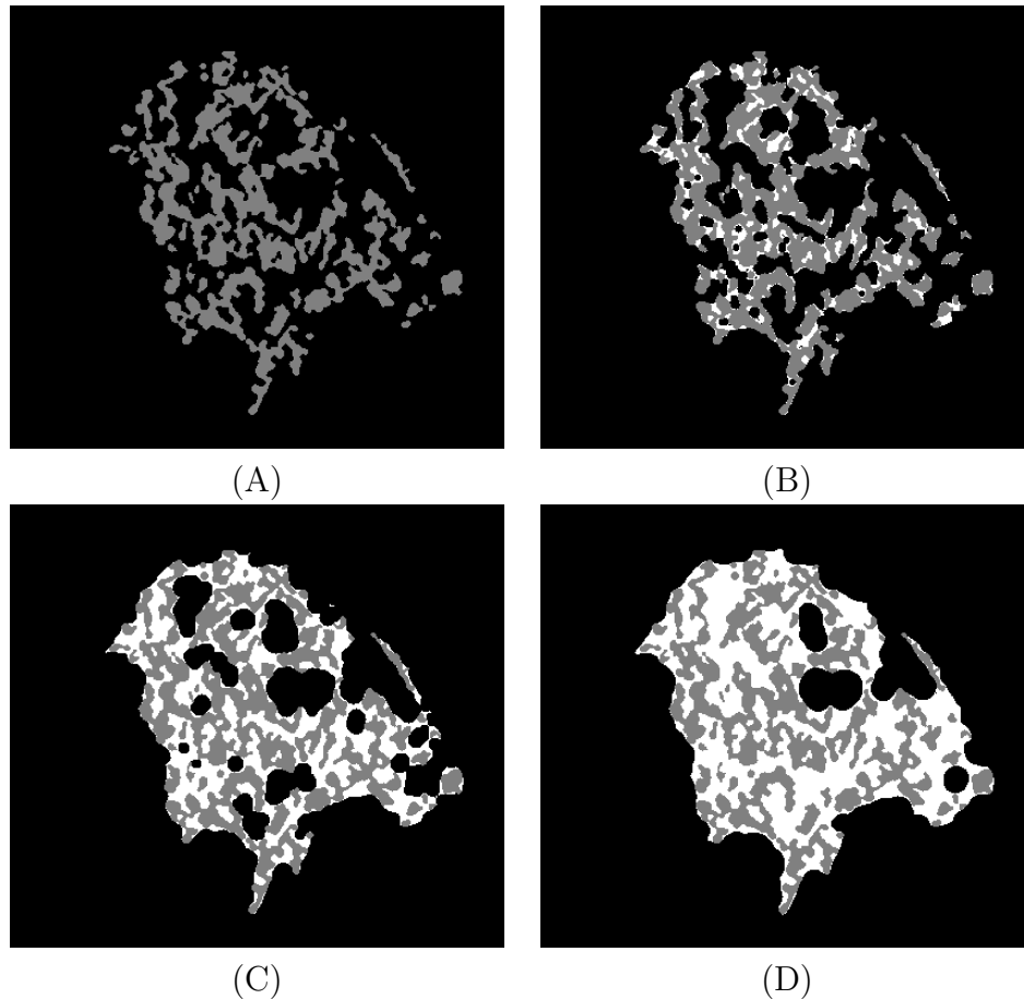
Figure 10.11: 2D sections during the capillary condensation simulation on the tomographic reconstruction of the mesoporous sample. (A) r_p = 0 nm, (B) r_p = 3.5 nm, (C) r_p = 7 nm, (D) r_p = 10.5 nm.
