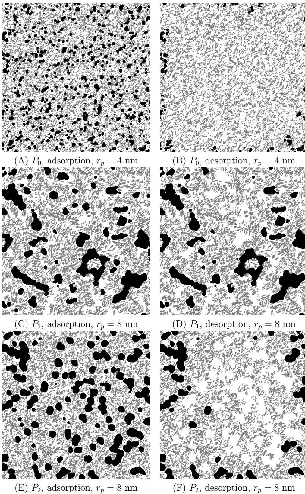
Figure 10.14: 2D sections of equilibrium states during the condensation & vaporization simulation on random models of platelets P_0 , P_1 and P_2 .
