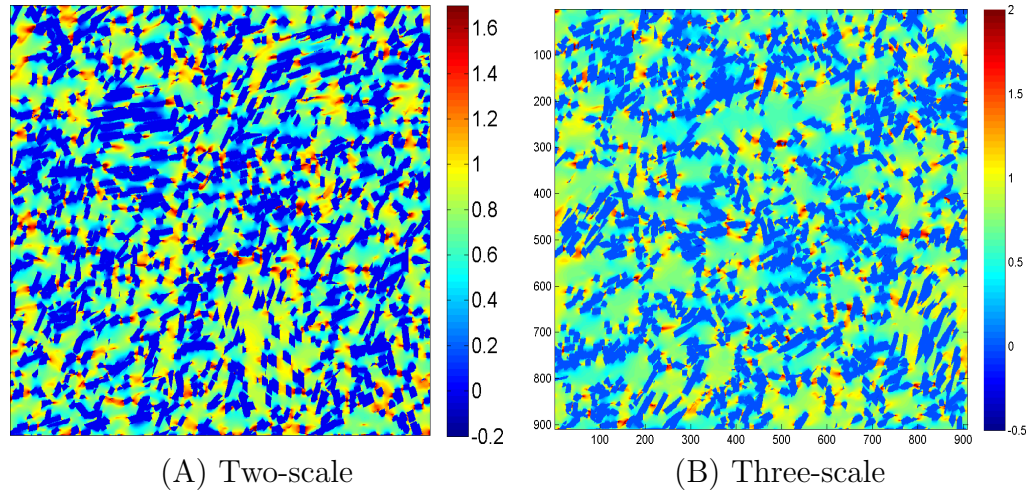
Figure 11.8: 2D sections of the first component of the flux field J_1 in the plane z = 256 obtained by FFT method on the identified random models of platelets with parameters shown in Tab. 11.5.
