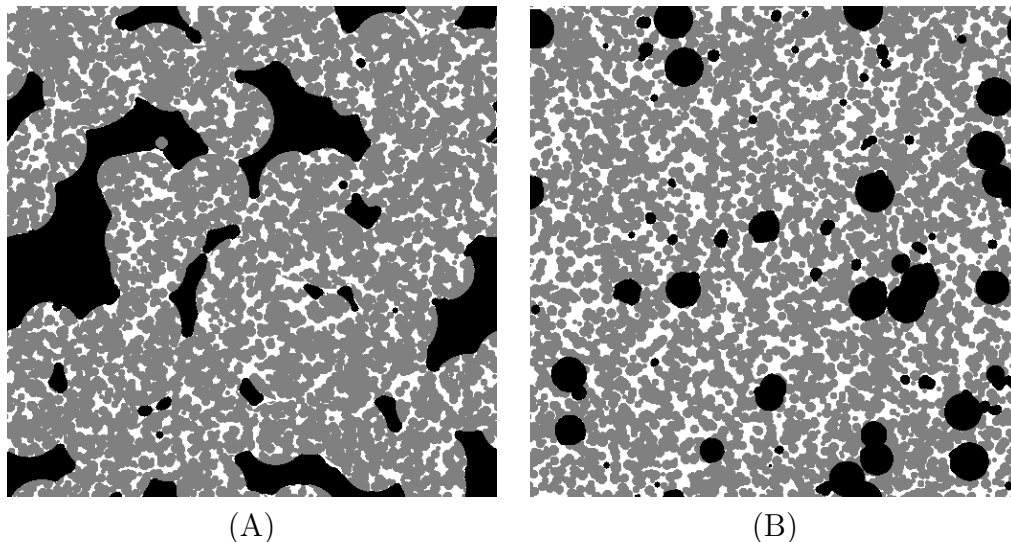
Figure 9.28: 2D sections of capillary condensation simulation during the adsorption at r_p=7 voxels. (A) Two-scale model D_1 . (B) Two-scale model D_2 .
