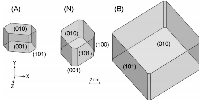
Figure 2.1: Bohemite particle morphology determined by XRD. The three samples are synthesised at different pH values: (A) pH=4.5, (N) pH=6.5 and (B) pH=11.5 (Chiche et al., 2008).
