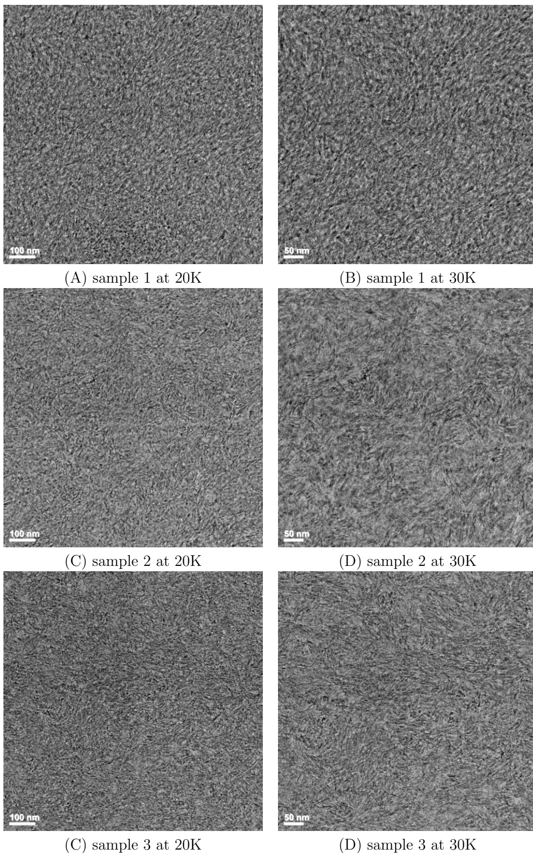
Figure 5.3: TEM images of 70 nm thick specimen of mesoporous alumina. The field of view for images at 20000 magnification is 1003 \text{ nm} \times 1003 \text{ nm} , and 676 \text{ nm} \times 676 \text{ nm} for 30000 magnification.
