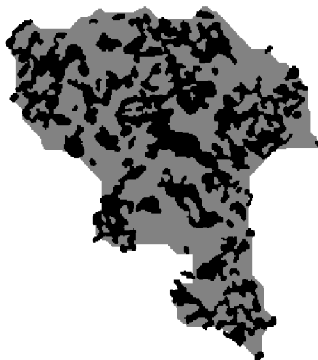
Figure 8.12: Porous volume of the tomography image after closing with rhombicuboctahedron of 30 voxels and erosion by 3 voxels (2D section). Alumina grains are in dark, while in grey is the porosity.
