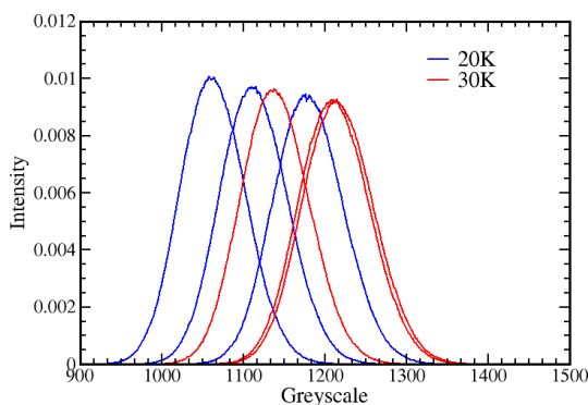
Figure 7.1: Histograms of TEM images of vacuum. Their greyscale means and standard deviations are listed in Tab. 7.1.
