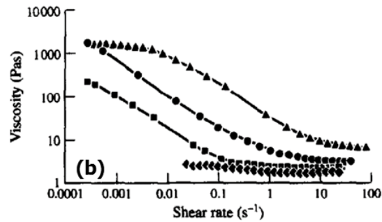
Fig. 5. Flow curves of plastisols with ETINOX resins: ● ETINOX 420, ▲ ETINOX 430, ◆ ETINOX 440, ■ ETINOX 450.
