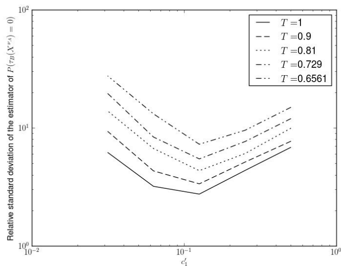
Figure 6.6 – Relative standard deviation of the estimators of \mathbb{P}(\tau_B(X^{\nu_A}) = 0) with respect to the dissipation c_1^{\nu} for various temperatures.
