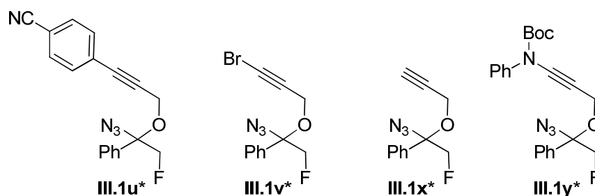
Figure 3.28- Unreactive substrates
