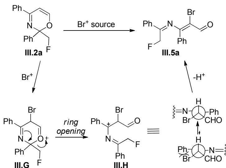
Figure 3.32 – Suggested mechanism for the brominative ring opening
