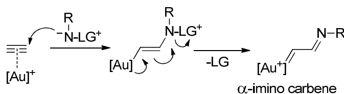
Figure 3.12 – Gold-catalyzed addition of nitrenoids to alkynes
