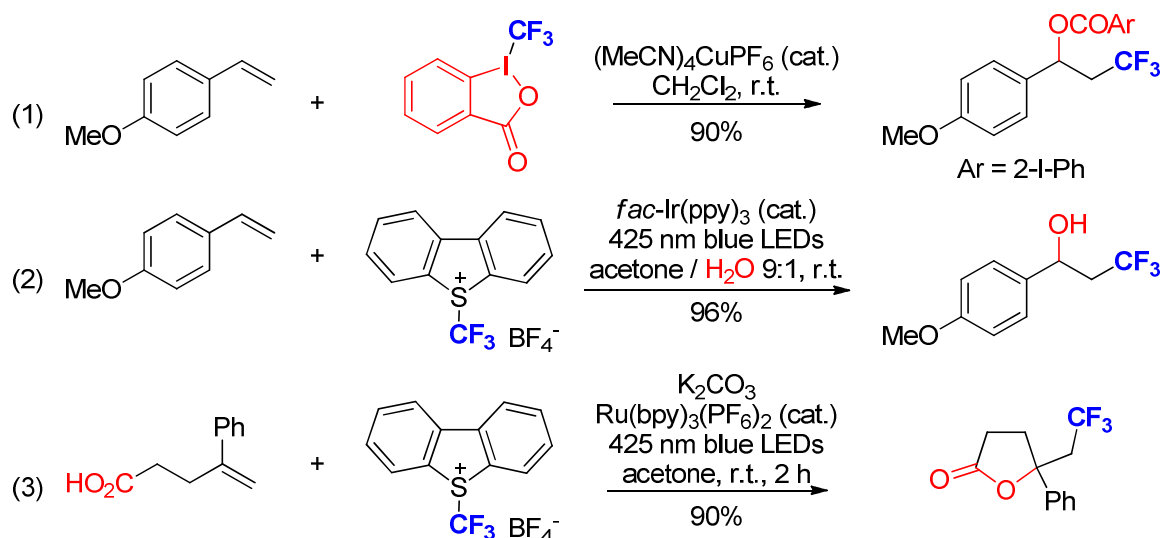
Figure 4.17 – Examples of oxytrifluoromethylation of unactivated alkenes
