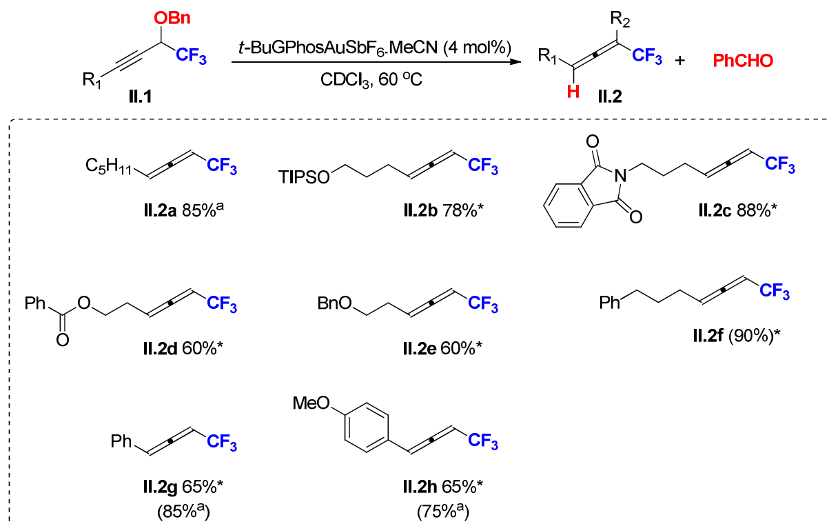
Figure 2.42 – Substrate scope for synthesis of 1,3-di-substituted trifluoromethyl allenes
