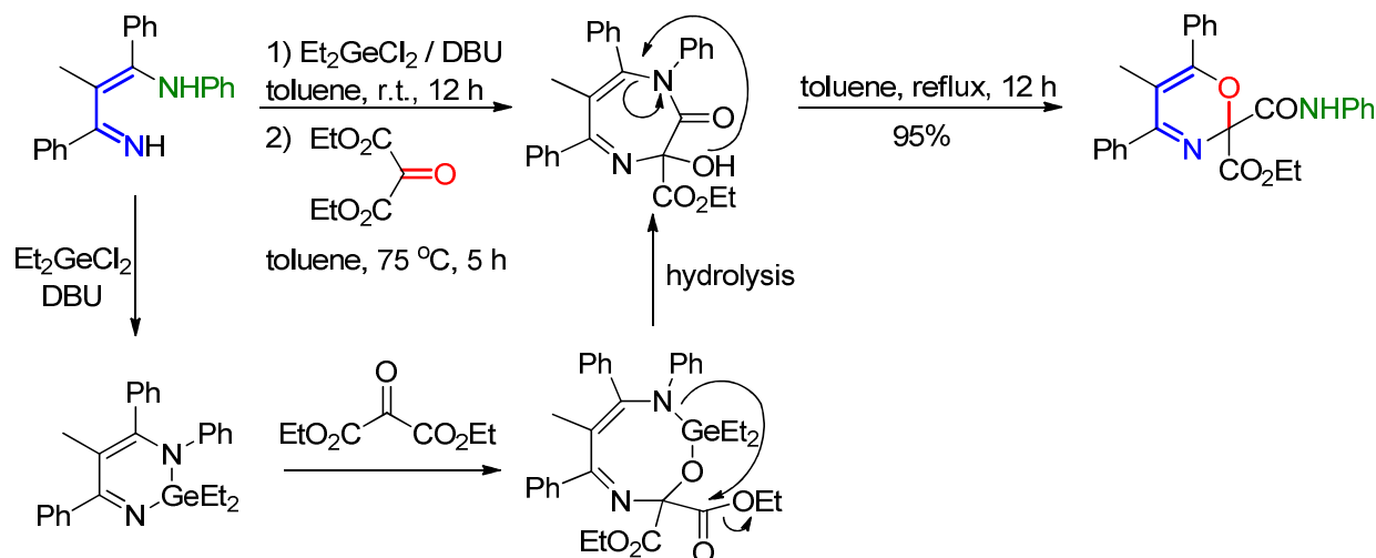
Figure 3.7 – Germanium-mediated synthesis of 2H-1,3-oxazines
