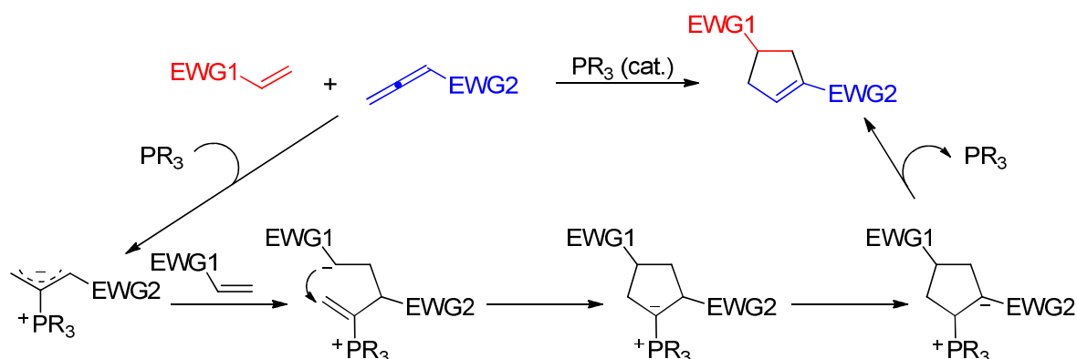
Figure 2.5 – [3+2] cycloadditions of allenes with activated alkenes
