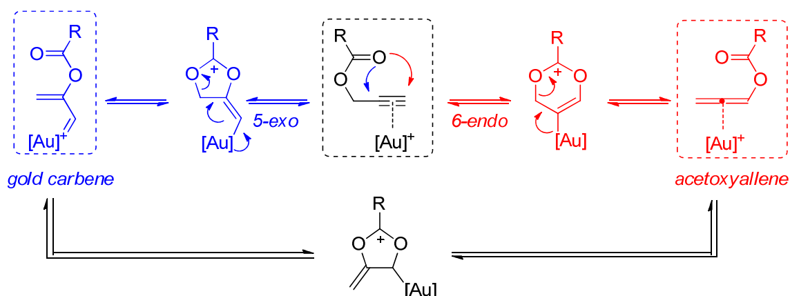
Figure 1.28 – Golden carousel of propargyl esters
