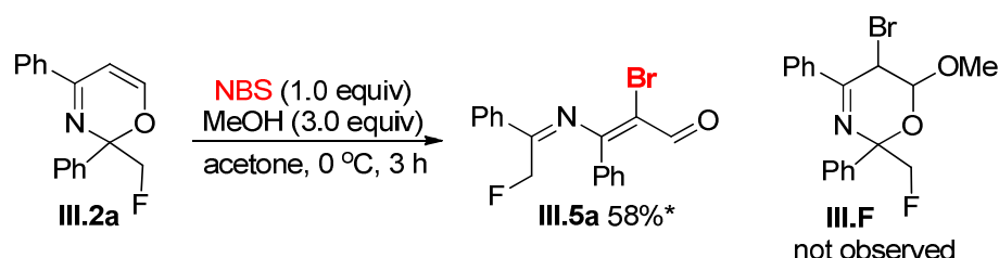
Figure 3.30 – First attempt for bromination of 2 H -1,3-oxazines
