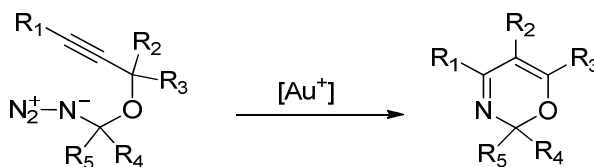
Figure 3.19 – Reaction design
