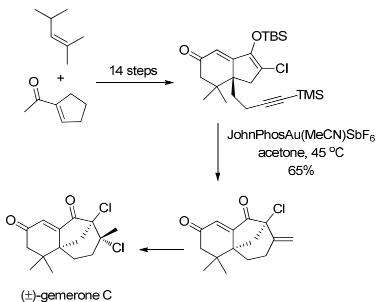
Figure 1.50 - Example of gold-catalyzed addition of carbon nucleophile Synthesis of ( \pm )-gemerone C
