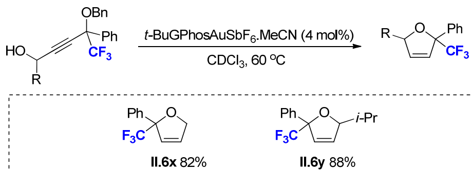
Figure 2.55 – Gold-catalyzed synthesis of trifluoromethyl dihydrofuranes
