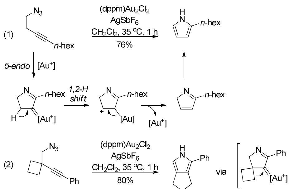
Figure 3.16 – Examples of 5-endo azide-yne cyclizations followed by rearrangement
