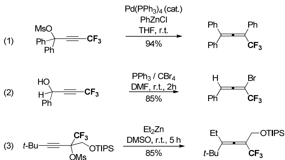
Figure 2.17 – Examples of synthesis of trifluoromethyl allenes by S_{N2}' substitution on trifluoromethyl alkynes
