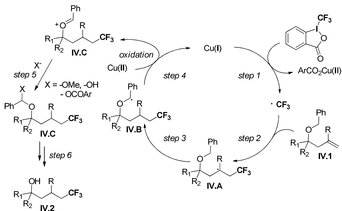
Figure 4.31 – Proposal for a formal hydrotrifluoromethylation of homoallylic alcohols using a benzyl group as a traceless hydrogen donor
