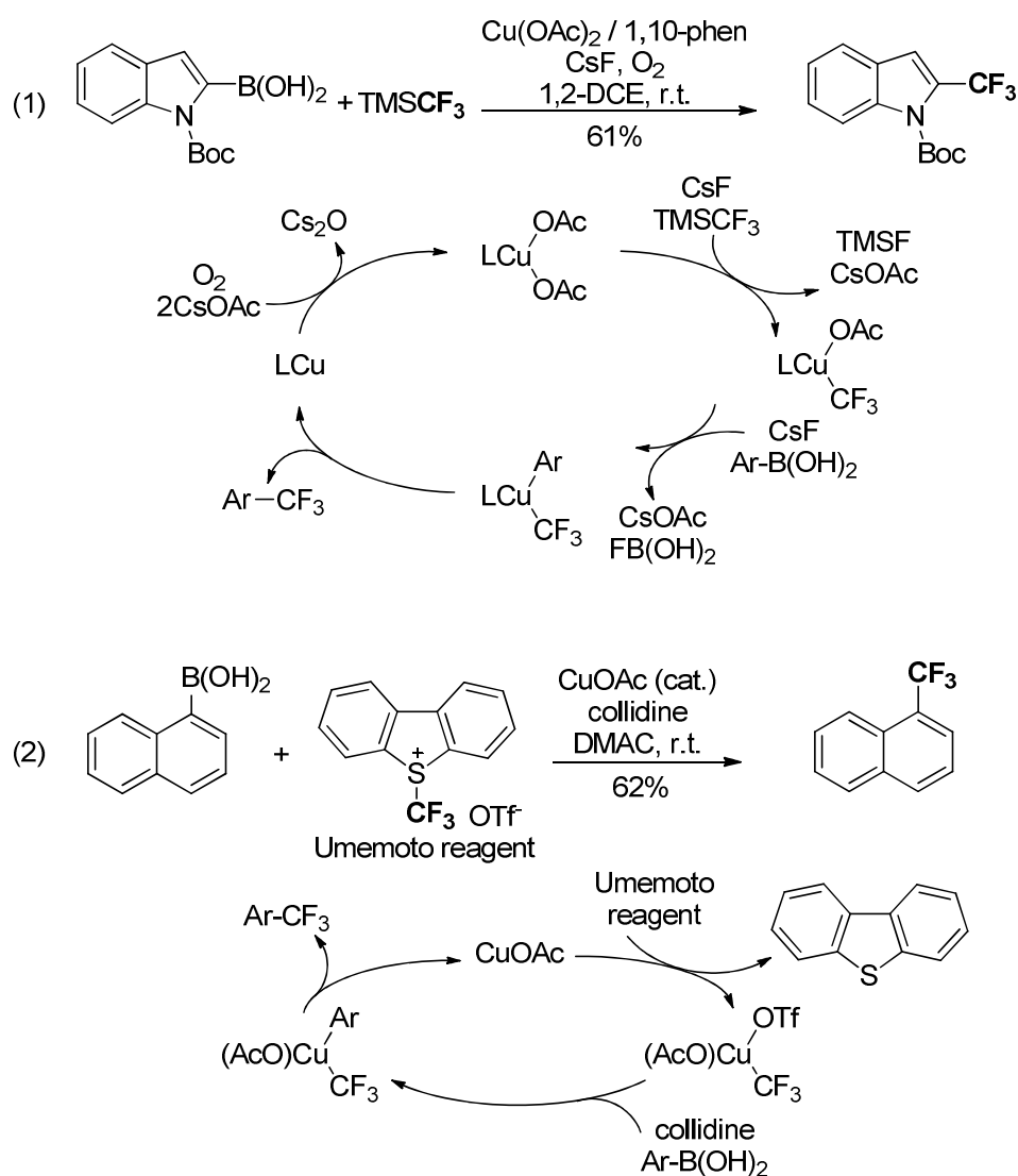
Figure 4.11 - Examples of cross-coupling trifluoromethylation reactions
