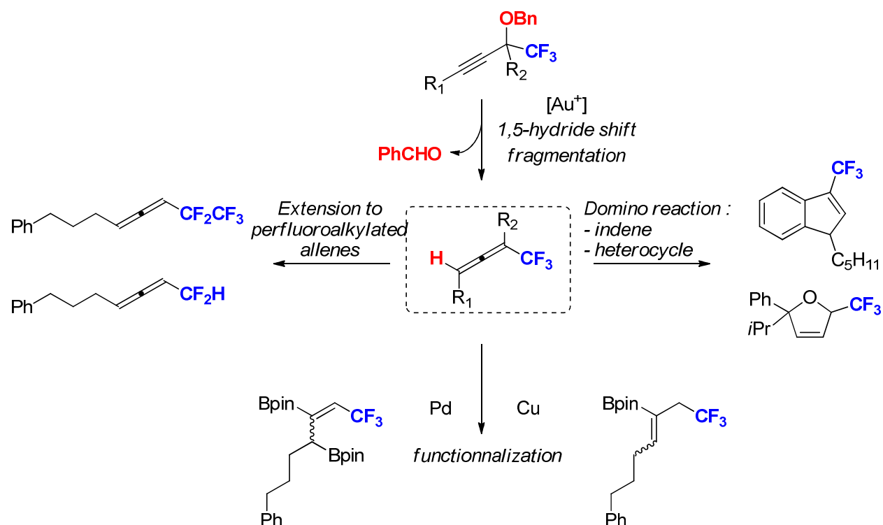
Figure 2.60 – Recapitulative scheme
