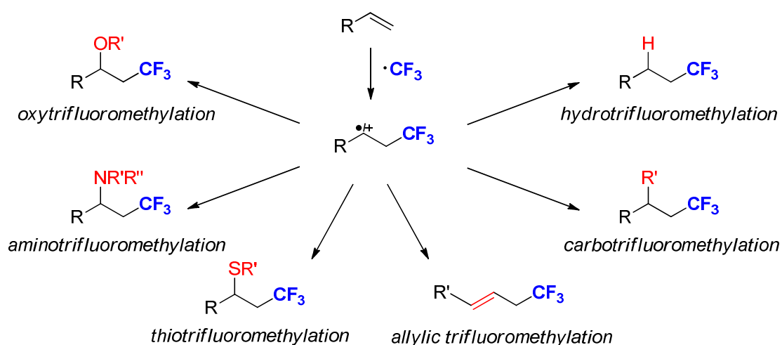
Figure 4.14 – General scheme for radical trifluoromethylation of alkenes
