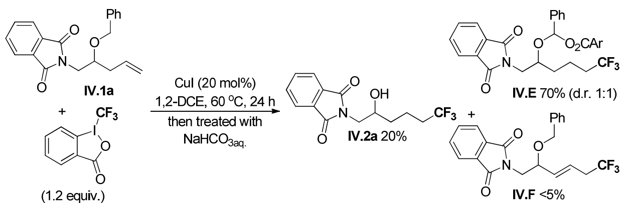
Figure 4.35 – First attempt for the hydrotrifluoromethylation of benzylic homoallylic ethers*
