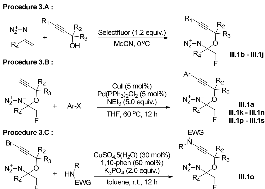
Figure 3.27 – General procedures for the preparation of the substrates
