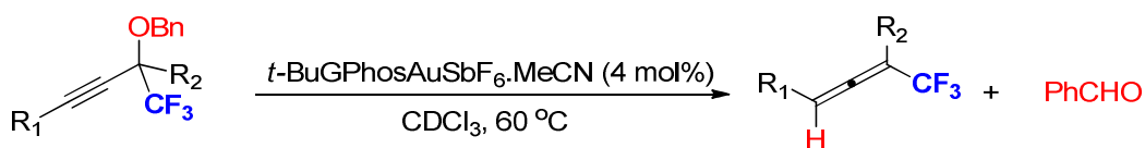
Gold-catalyzed synthesis of trifluoromethylated allenes
