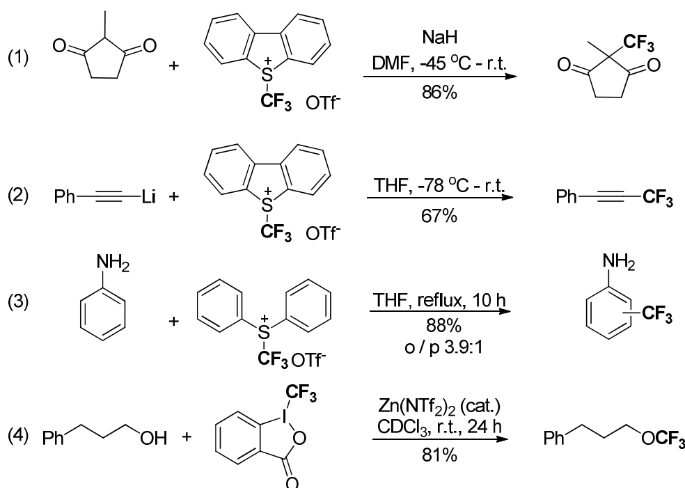
Figure 4.10 - Examples of electrophilic trifluoromethylation reactions
