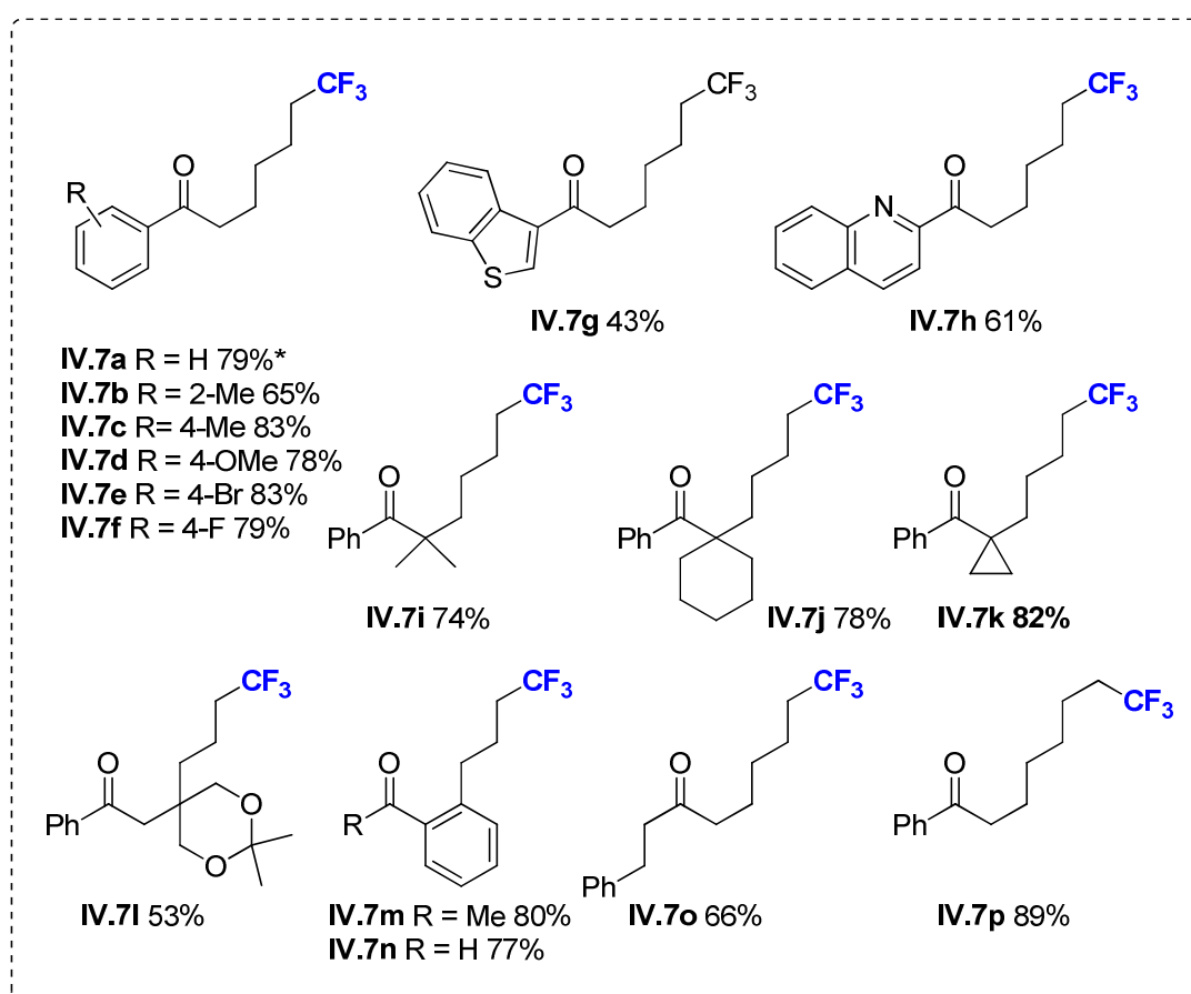
Figure 4.49 – Substrate scope for the trifluoromethylation of 5-alkenol substrates
