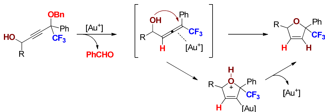
Figure 2.54 – Design of the cascade heterocyclization reaction
