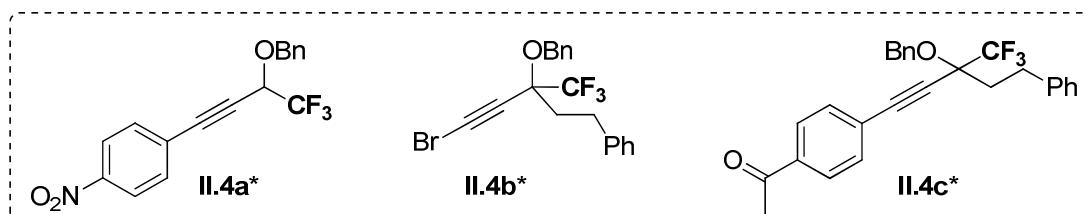
Figure 2.47 – Unreactive substrates showing the importance of the C≡C bond polarization
