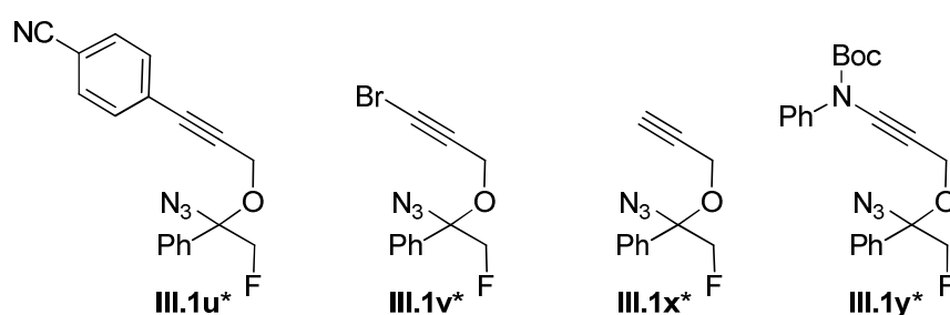
Figure 3.28- Unreactive substrates
