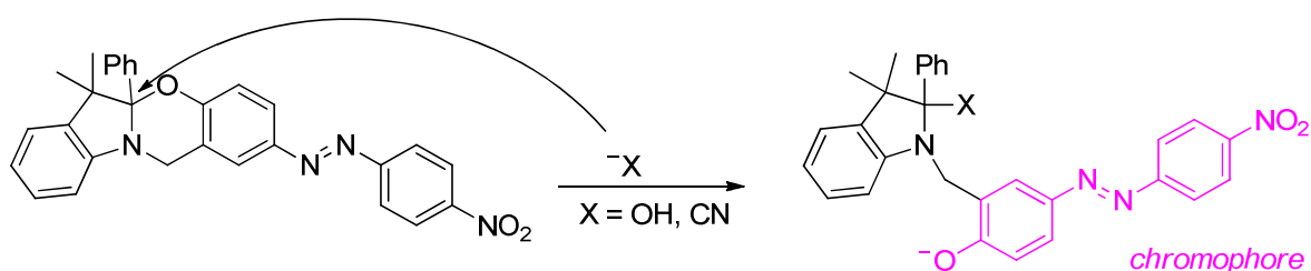
Figure 3.3 – Example of use of oxazines in chromophore cyanide and pH change detectors
