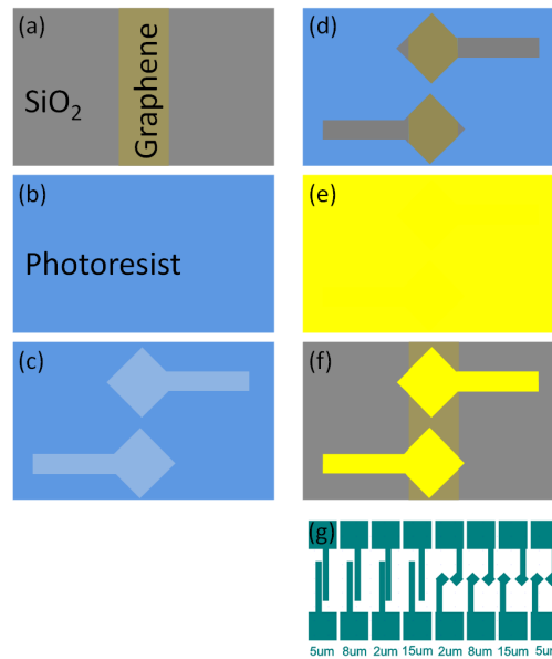
Figure 2.4: Patterning of the electrodes. (a) Graphene band on SiO 2 . (b) Spin-coating of negative photoresist. (c) UV light exposure through the mask. (d) Development. (e) Electron beam evaporation of Ti/Au. (f) Lift-off. (g) Design of the mask for electrode patterning.
