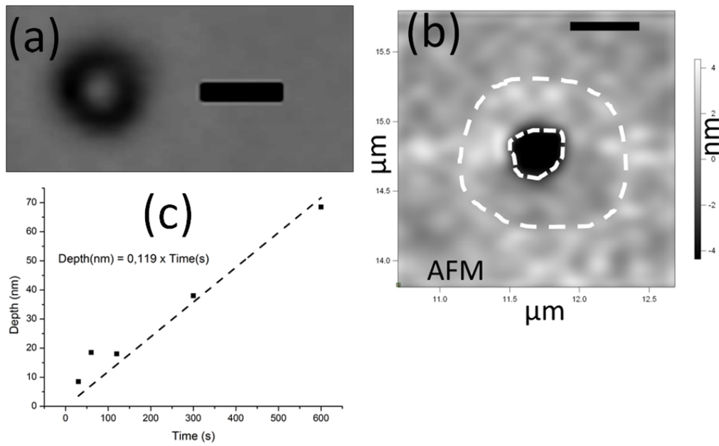
Figure 3.2: Morphology of laser-annealed textured carbon. (a) Optical image (scale bar 1 \mu\text{m} ) of a laser-annealed region with energy density 5.9 \cdot 10^6 \text{ J} \cdot \text{mm}^{-2} . (b) AFM 2D height image showing a crater (black surrounded by a white dashed line) and a surrounding bulge (marked with a white dashed line) of a laser-annealed region with energy density 1.7 \cdot 10^7 \text{ J} \cdot \text{mm}^{-2} . (c) Measured depths as a function of time.
