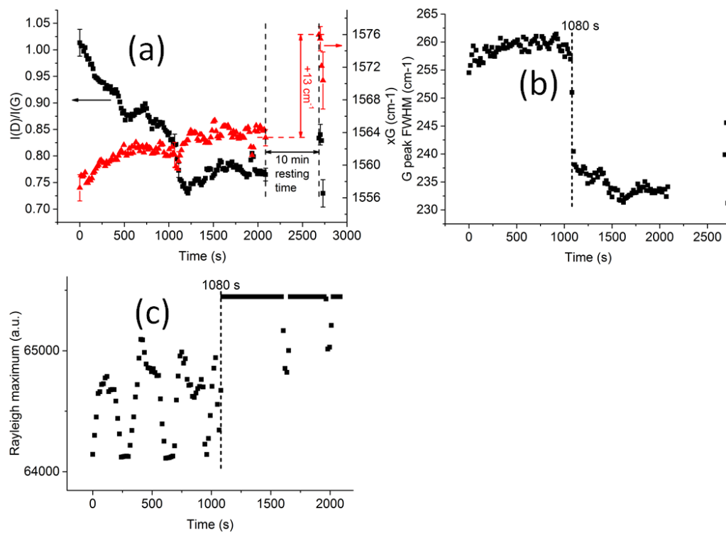
Figure 3.4: (a) Evolution of the I(D)/I(G) ratio (black squares) and G peak position values (red triangles) as a function of time for a film annealed at 16 \text{ kW}\cdot\text{mm}^{-2} . The last four spectra (after 10 min resting time) are taken with much lower Raman power densities to avoid inducing further structural changes. (b) Evolution of the G peak FWHM as a function of time for the same annealing experiment. (c) Evolution of the maximum of the Rayleigh peak as a function of time for the same annealing experiment.
