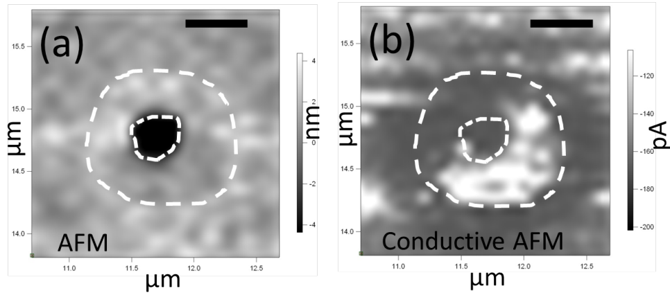
Figure 3.5: conductive AFM data suggest that sp^2 clustering takes place around the crater. ( 1.7 \cdot 10^7 \text{ J} \cdot \text{mm}^{-2} ) (a) AFM image. (b) c-AFM image of a laser-annealed crater showing that the highest conduction regions are at the location of the bulge surrounding the hole.
