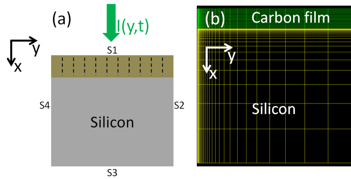
Figure 4.11: Geometry defined in Cast3M. (a) Carbon thin film ( x -size = 300 nm, y -size = 100 \mu\text{m} ) on top of a silicon substrate ( x -size = 2 \mu\text{m} , y -size = 100 \mu\text{m} ). (b) Geometry and meshing implemented in Cast3M. The entirety of the simulated structure is not shown as it is too long in the y direction.
