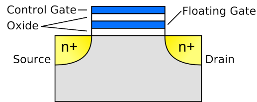
Figure 1.6: Schematic of a floating-gate-transistor (Flash). Reproduced from http://elec424.rice.edu/gigamesh/blog/index.php?m=01&y=09&d=18&entry=entry090122-181953 .
