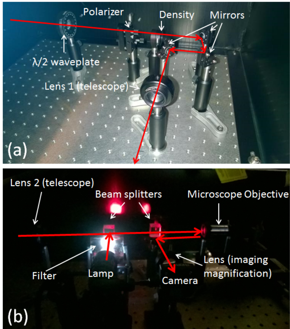
Figure 2.8: Femtosecond laser-annealing setup. (a) Control of the power via the \lambda/2 waveplate, the polarizer and the density. (b) Confocal imaging system and annealing setup.
