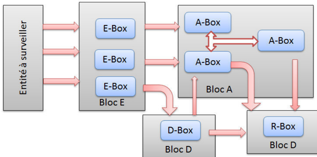
FIGURE 3.1 – Architecture Common Intrusion Detection Framework.
