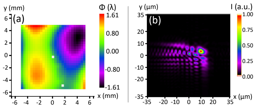
Figure 2.15: (a) Wavefront of the harmonic beam measured after focusing by the KB and (b) its calculated focal spot, with a Strehl ratio of 0.066. The wavefront has RMS and PV values of 0.794\lambda and 3.228\lambda , respectively.
