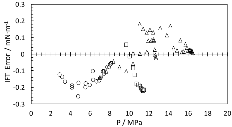
Figure 5.9. Deviation between prediction and experimental IFT data ( \text{IFT}_{\text{Error}} = \text{IFT}^{\text{EXP}} - \text{IFT}^{\text{CALC}} ). Symbols: \text{CO}_2+n\text{-C}_4 (○), \text{CO}_2+n\text{-C}_{10} (△) and \text{CO}_2+n\text{-C}_4+n\text{-C}_{10} (□) systems.
