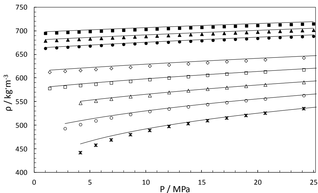
Figure 4.21. Single-phase density predictions using the SAFT- \gamma Mie. Symbols are data for the system 0.66 mol n -C 4 + 0.34 mol n -C 10 at ( \diamond ) 344, ( \square ) 377, ( \triangle ) 410, ( \circ ) 444 and ( \times ) 477 K [190] and for the system 0.53 mol n -C 8 + 0.47 mol n -C 10 at ( \blacksquare ) 323 K, ( \blacktriangle ) 343 K and ( \bullet ) 363 K [191].
