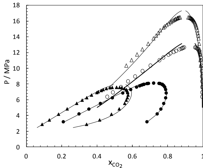
Figure 5.4. Pressure-composition diagram of \text{CO}_2+n\text{-C}_4 (black [214]) and \text{CO}_2+n\text{-C}_{10} (white [215]) systems using the SAFT-VR Mie EoS. Symbols: ( \bullet\circ ) T=344.3 and ( \blacktriangle\triangle ) T=377.6\text{K} .
