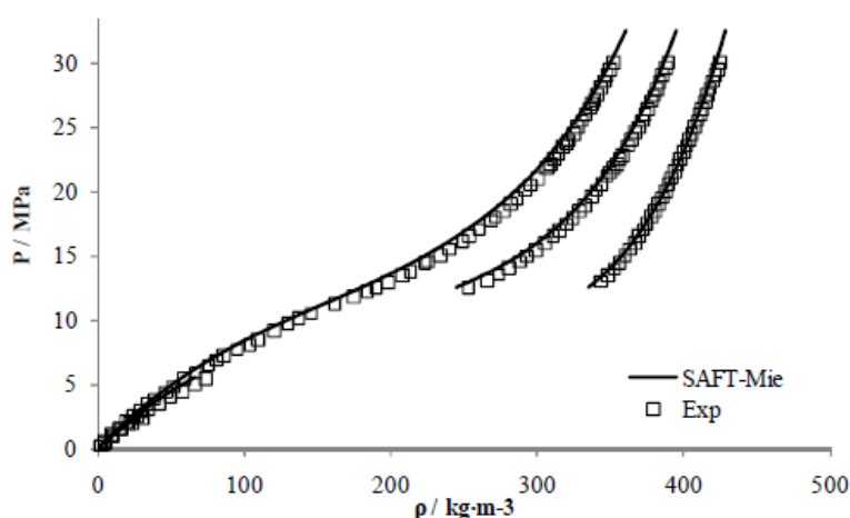
Fig. 1: Density of binary system \text{CH}_4 - 28.6% \text{H}_2\text{S} at 253, 273 and 293K. Continuous line is the predicted density by SAFT-VR Mie and symbols are experimental data (this work).
