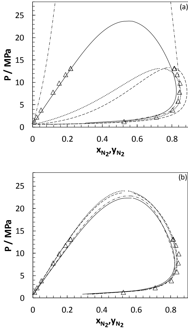
Figure 4.8. Pressure–composition diagrams of the \text{CO}_2 + \text{N}_2 system at 218K. Experimental data ( \Delta ) [176]. The SRK (dashed lines), PR (dotted line), PC-SAFT (continuous line) and SAFT-VR Mie (dot-dashed line) EoS with k_{ij}=0 (a) and with regressed k_{ij} (b).
