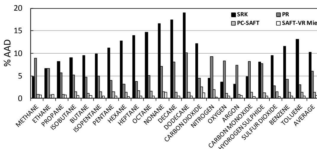
Figure 4.12. Deviations in the correlated saturated liquid density by SRK (black), PR (dark gray), PC-SAFT (light gray) and SAFT-VR Mie (white) EoS.
