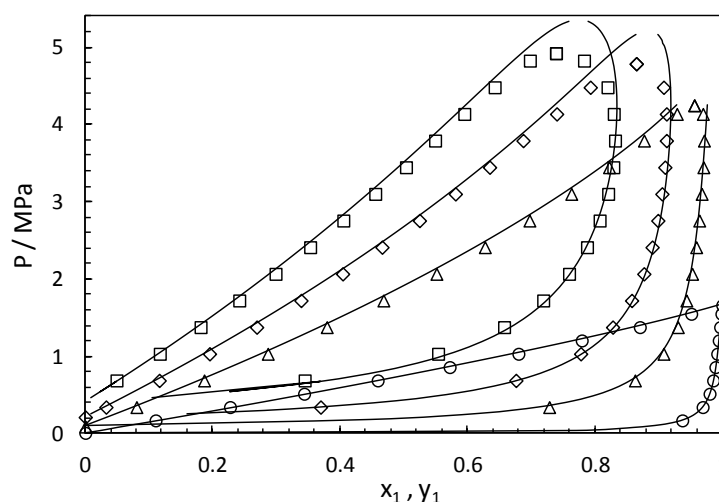
Figure 4.20. VLE of the binary mixture of n -butane (1) and n -decane (2). The continuous curves represent the prediction using the SAFT- \gamma Mie EoS and the symbols the experimental data at (○) 377 K, (△) 444 K, (◇) 477 K and (□) 511 [189].
