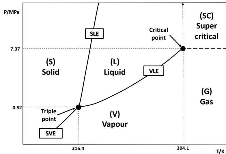
Figure 3.4. P-T simplified phase diagram of CO 2 [80].
