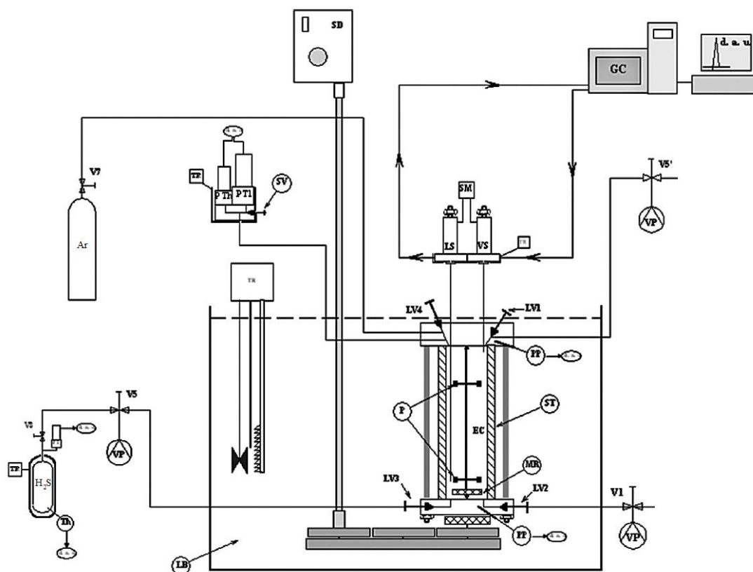
Figure 2.1. Schematic diagram of the VLE equipment [27]: EC, equilibrium cell; LB, liquid bath; LS, liquid sampler; PP, platinum resistance probe; PT, pressure transducer; TR temperature regulator, VS, vapour sampler; VP, vacuum pump.
