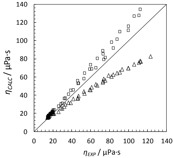
Figure 6.25. Viscosity predictions from ST ( \square ) and CO 2 -ST ( \triangle ) models against experimental measurements.
