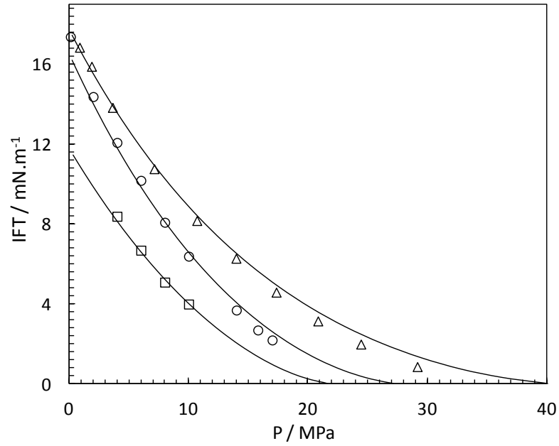
Figure 5.13. Experimental and predicted IFT using the DGT-SAFT VR Mie model for the systems: \text{CH}_4 +propane at 338K ( \square ) [220], \text{CH}_4 + n -hexane at 350K ( \circ ) [223] and \text{CH}_4 + n -decane at 343K ( \triangle ) [219].
