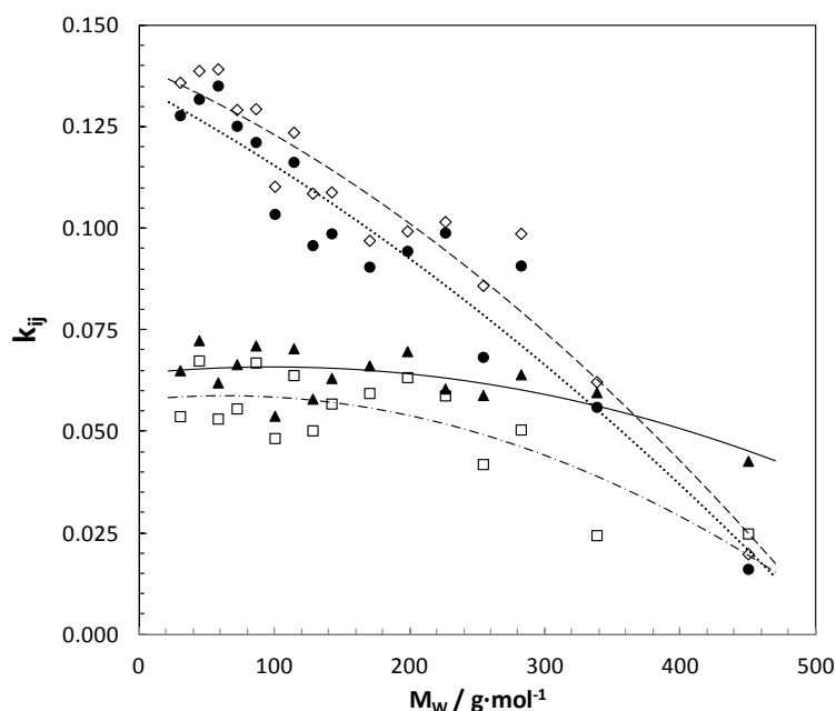
Figure 4.7. Binary interaction parameters of n-alkanes + CO 2 binary system and their trend curves for the SRK (◇, dashed lines), PR (●, dotted line), PC-SAFT (▲, continuous line) and SAFT-VR Mie (□, dot-dashed line) EoS.
