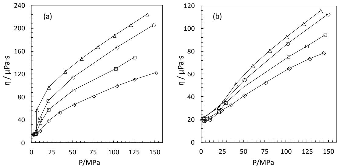
Figure 6.26. Experimental viscosity of pure CO 2 and three multicomponent CO 2 -rich mixtures at 298 (a) and 423 (b) K. Data: pure CO 2 ( \triangle ) [171], MIX2( \circ ) [55], MIX3 ( \square ) [24] and MIX4 ( \diamond ) (this work).
