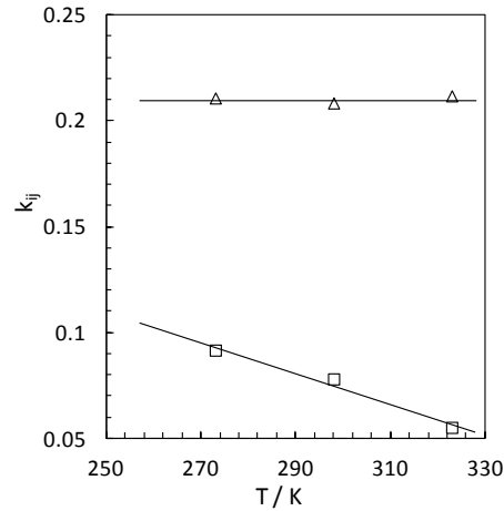
Figure 6.2. Regressed values and trends of the BIPs for the Ar-H 2 S system with the ( \Delta ) PR and ( \square ) SAFT-VR Mie EoS.
