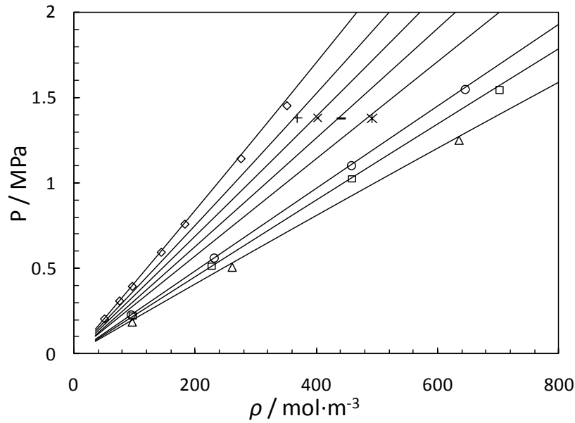
Figure 6.15. P- \rho diagram of several systems of \text{H}_2\text{S} + \text{CH}_4 at 8 isotherms. Comparison of predictions with low pressure virial EoS and experimental data: T=253\text{K} and x_{\text{CH}_4}=0.87 ( \Delta ), T=273\text{K} and x_{\text{CH}_4}=0.82 ( \square ), T=293\text{K} and x_{\text{CH}_4}=0.71 ( \circ ), T=344\text{K} and x_{\text{CH}_4}=0.4 ( * ), T=377\text{K} and x_{\text{CH}_4}=0.5 ( - ), T=411\text{K} and x_{\text{CH}_4}=0.6 ( + ), T=444\text{K} and x_{\text{CH}_4}=0.8 ( \times ) and T=500\text{K} and x_{\text{CH}_4}=0.5 ( \diamond ) [32,33].
