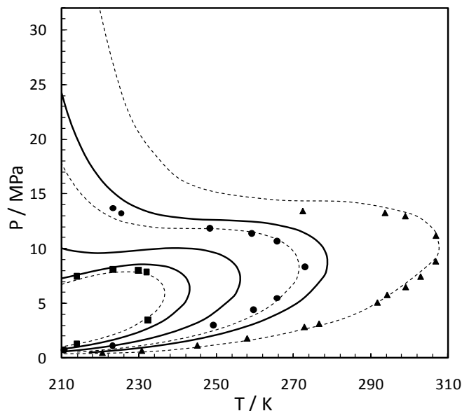
Figure 2.3. Predicted phases envelopes with the PR EoS of the methane + hydrogen sulphide systems with 0.1101, 0.1315, 0.1803, 0.248, 0.286 and 0.458 mol fractions of \text{H}_2\text{S} . The solid lines are the compositions studied in this work and the dashed lines are other phase diagrams compared against Kohn and Kurata data [43]: (■) 0.1101, (●) 0.248 and (▲) 0.458 mol fractions of \text{H}_2\text{S} .
