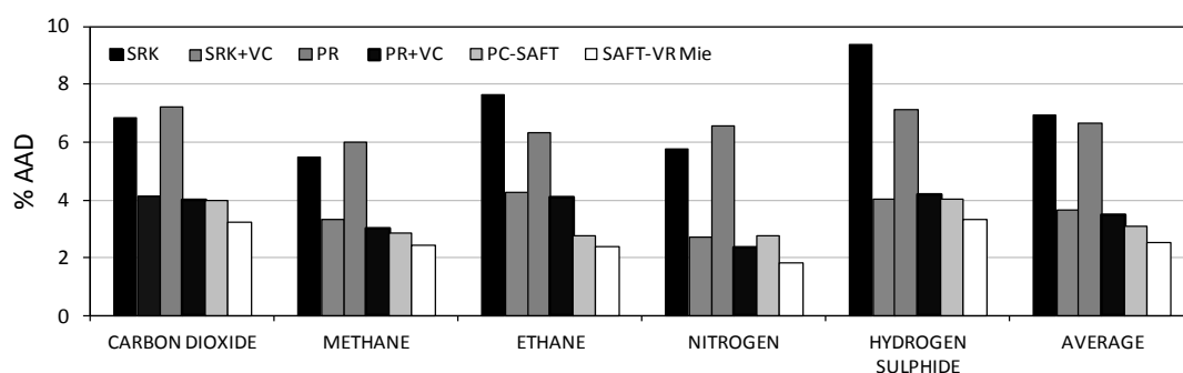
Figure 4.13. Deviations in the calculated density of binary systems of CO 2 , CH 4 , C 2 H 6 , N 2 and H 2 S + Comp2 by SRK (black), SRK+Peneloux (diagonal grey lines), PR (dark grey), PR+Peneloux (vertical grey lines) PC-SAFT (light grey) and SAFT-VR Mie (white) EoS.
