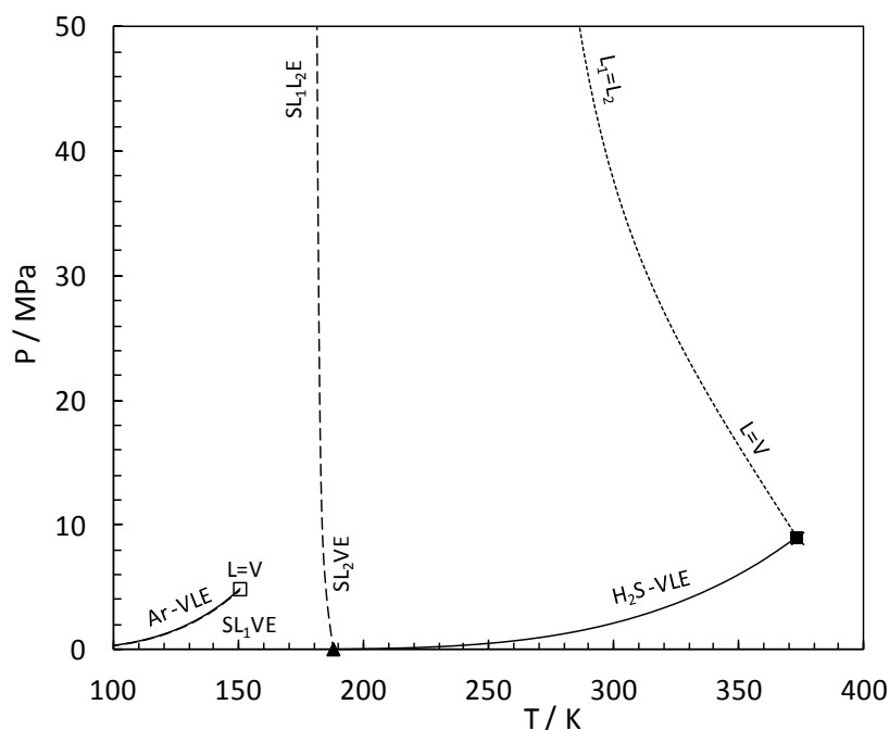
Figure 6.7. P-T diagram of the Ar (1) + \text{H}_2\text{S} (2) system. Solid lines are the saturations lines of each pure compound [42]. Doted lines and dashed lines are the critical and solid-fluid equilibrium lines predicted with the PR EoS. Symbols: (□) critical point of Ar, (■) and (▲) critical and triple points of \text{H}_2\text{S} [50]
