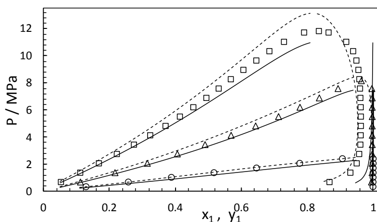
Figure 4.19. Pressure-composition representation of the VLE of the binary mixture of ethane (1) and n-decane (2). The continuous curves represent the prediction of SAFT- \gamma Mie estimation, the dashes curves the prediction of SAFT-VR Mie and the symbols the experimental data at (○) 277 K, (△) 344 K and (□) 444 K [187].
