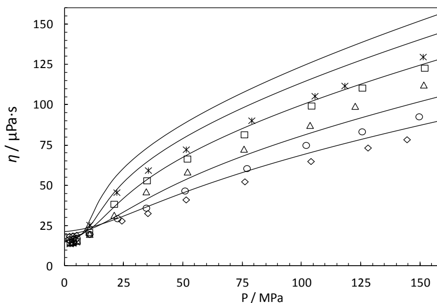
Figure 6.24. Experimental and predicted viscosity of MIX4. Continuous line: predictions using the SUPERTRAPP+SAFT-VR Mie EoS. Data at 283 (*), 298 (□), 323 (Δ), 373 (○) and 423K (◇).
