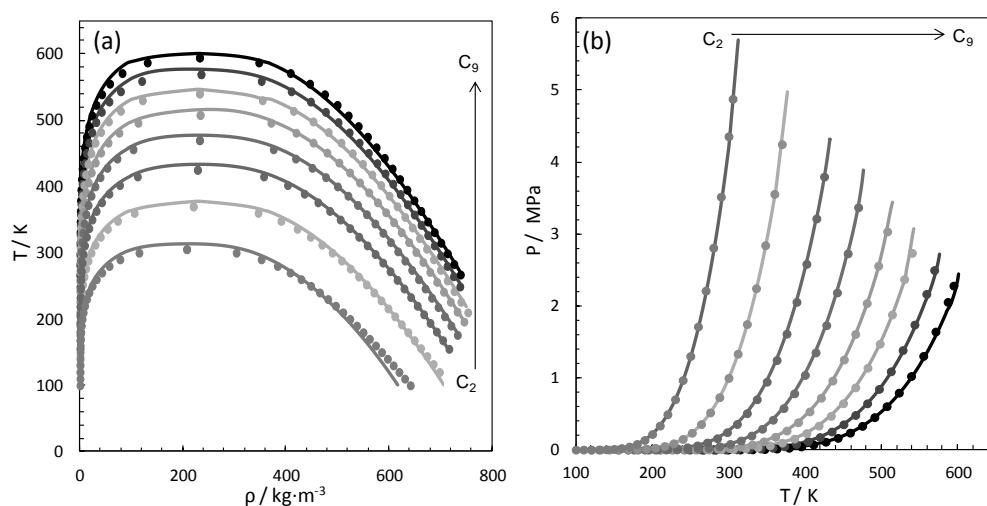
Figure 4.18. Comparison between the SAFT- \gamma Mie EoS and experimental data of saturated densities (a) and saturation pressures (b) for the C2-C9 n -alkanes series. The symbols represent the pure-component correlated data from NIST [42] and curves represent SAFT- \gamma predictions.
