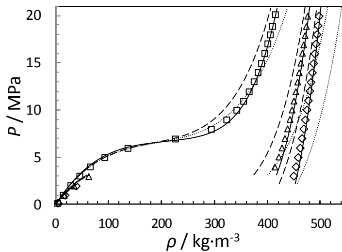
Figure 4.15. Experimental and calculated densities of the 0.857 mole \text{C}_2\text{H}_6 + 0.143 mole \text{H}_2\text{S} using SAFT-VR Mie (continuous lines), SRK+Peneloux (dashed lines) and SRK (dotted lines) EoS with the regressed k_{ij} . Symbols [20]: ( \diamond ) 268K, ( \triangle ) 283K and ( \square ) 322K.
