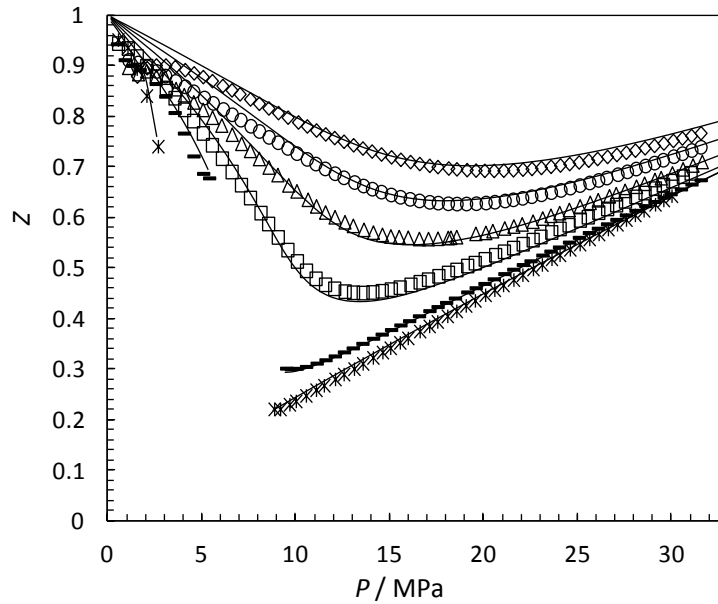
Figure 6.21. Compressibility factor of the \text{CO}_2 + \text{CH}_4 + \text{H}_2\text{S} ternary mixture. Comparison between the SAFT-VR Mie calculation and experimental data in this work: (*) 253 K, (—) 273 K, (□) 293 K, (△) 313, (○) 323 K, and (◇) 353 K.
