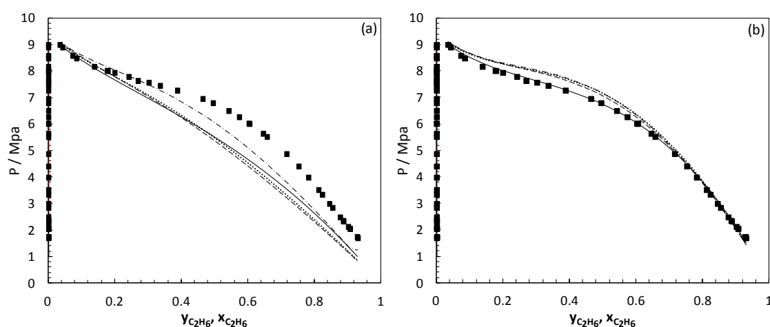
Figure 4.10. Pressure–composition diagrams of the \text{C}_2\text{H}_6 + \text{Ar} system at 116K. Experimental data ( \blacksquare ) [178]. The SRK (dashed lines), PR (dotted line), PC-SAFT (continuous line) and SAFT-VR Mie (dot-dashed line) EoS with k_{ij} = 0 (a) and with regressed k_{ij} (b).
