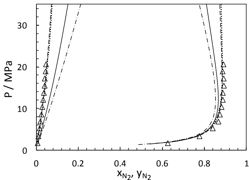
Figure 4.11. Pressure–composition diagram of the N_2 + H_2S system at 256K. Comparison between experimental data ( \Delta ) [179], the SAFT-VR Mie EoS with k_{ij}=0 (continuous line) and with regressed k_{ij} (dashed lines) and the PR EoS with k_{ij}=0 (dot-dashed line) and with regressed k_{ij} (dotted line).
