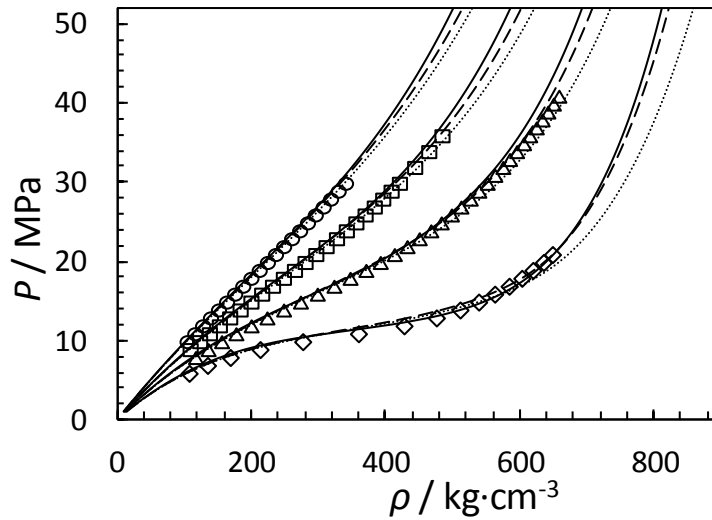
Figure 4.14. Experimental and calculated densities of the 0.514 mole \text{CO}_2 + 0.486 mole \text{H}_2\text{S} using SAFT-VR Mie (continuous lines), PR+Peneloux (dashed lines) and PR (dotted lines) EoS with the regressed k_{ij} . Symbols [182]: ( \diamond ) 350K, ( \triangle ) 400K, ( \square ) 450K and ( \circ ) 500K.
