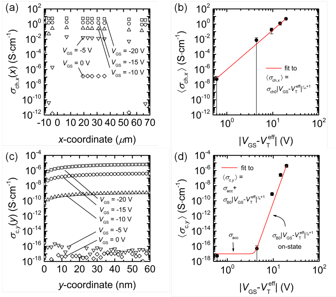
Figure 5-4: (a) Channel conductivity \sigma_{ch,x} and (b) its average on x -axis \langle\sigma_{ch,x}\rangle (at y = 2 nm), and (c) contact conductivity in the transition zone \sigma_{c,y} and (d) its average on y -axis \langle\sigma_{c,y}\rangle (at x = -5 \mu m) calculated at various gate voltage: V_{GS} = 0, -5, -10, -15 and -20 V. Note the power-law dependence of both channel and contact conductivity with respect to the effective gate voltage. In particular, \langle\sigma_{c,y}\rangle contains an asymptotic element \sigma_{acc} and a power-law dependent element \sigma_B .
