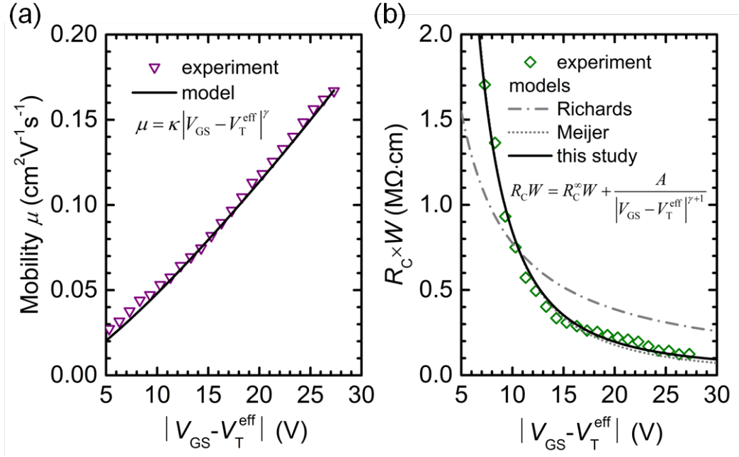
Figure 5-11: (a) Mobility and (b) contact resistance as a function of the effective gate voltage |V_{\text{GS}} - V_{\text{T}}^{\text{eff}}| extracted by the TLM. The solid lines are a fit to the power-law mobility and contact resistance models (inset equations). Thanks to pre-determined parameters by the ratio method ( V_{\text{T}}^{\text{eff}} = -12.7 V and \gamma = 1.24 ), all the rest ( \kappa , A and R_{\text{C}}^{\infty}W ) can be determined by linear extrapolation. Dotted and dash-dot lines correspond to the model of Richards and Meijer, which is a specific case of the proposed model where \gamma = 0 or R_{\text{C}} = 0 .
