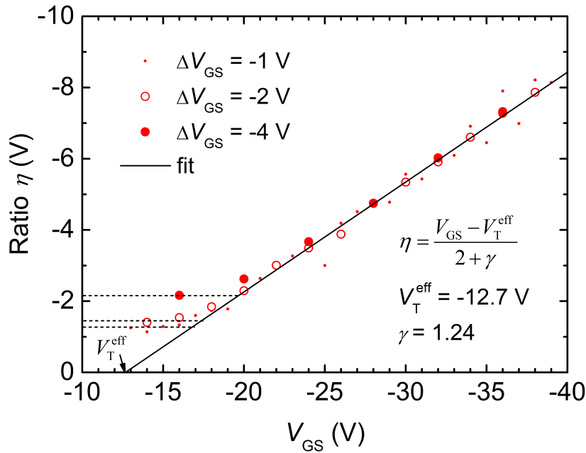
Figure 5-9: Ratio \eta as a function of V_{GS} calculated for different values of \Delta V_{GS} using (5.39) from the transfer characteristics of a pentacene-based OFET with L = 60\text{ }\mu\text{m} (symbols). The solid line is a fit to (5.37) for the extraction of the effective threshold voltage V_T^{\text{eff}} and power-law exponent \gamma . Dotted lines are a guide to the eye for the asymptotic behaviour calculated by (5.43).
