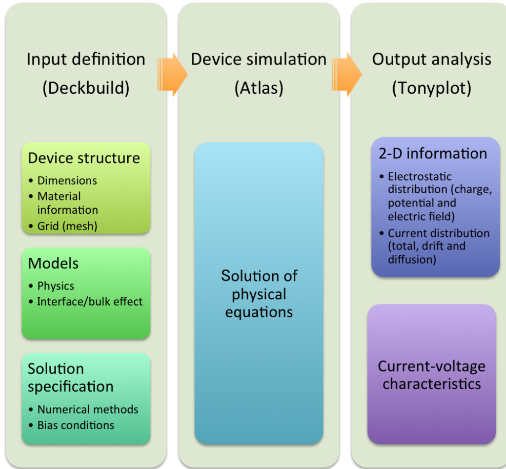
Figure 3-6: Device simulation process and tasks at each step for 2-D physically-based finite-element simulator.
