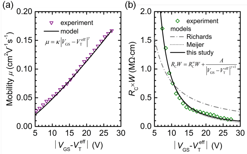
Figure 5-11: (a) Mobility and (b) contact resistance as a function of the effective gate voltage |V_{GS} - V_T^{\text{eff}}| extracted by the TLM. The solid lines are a fit to the power-law mobility and contact resistance models (inset equations). Thanks to pre-determined parameters by the ratio method ( V_T^{\text{eff}} = -12.7 V and \gamma = 1.24 ), all the rest ( \kappa , A and R_C^\infty W ) can be determined by linear extrapolation. Dotted and dash-dot lines correspond to the model of Richards and Meijer, which is a specific case of the proposed model where \gamma = 0 or R_C = 0 .
