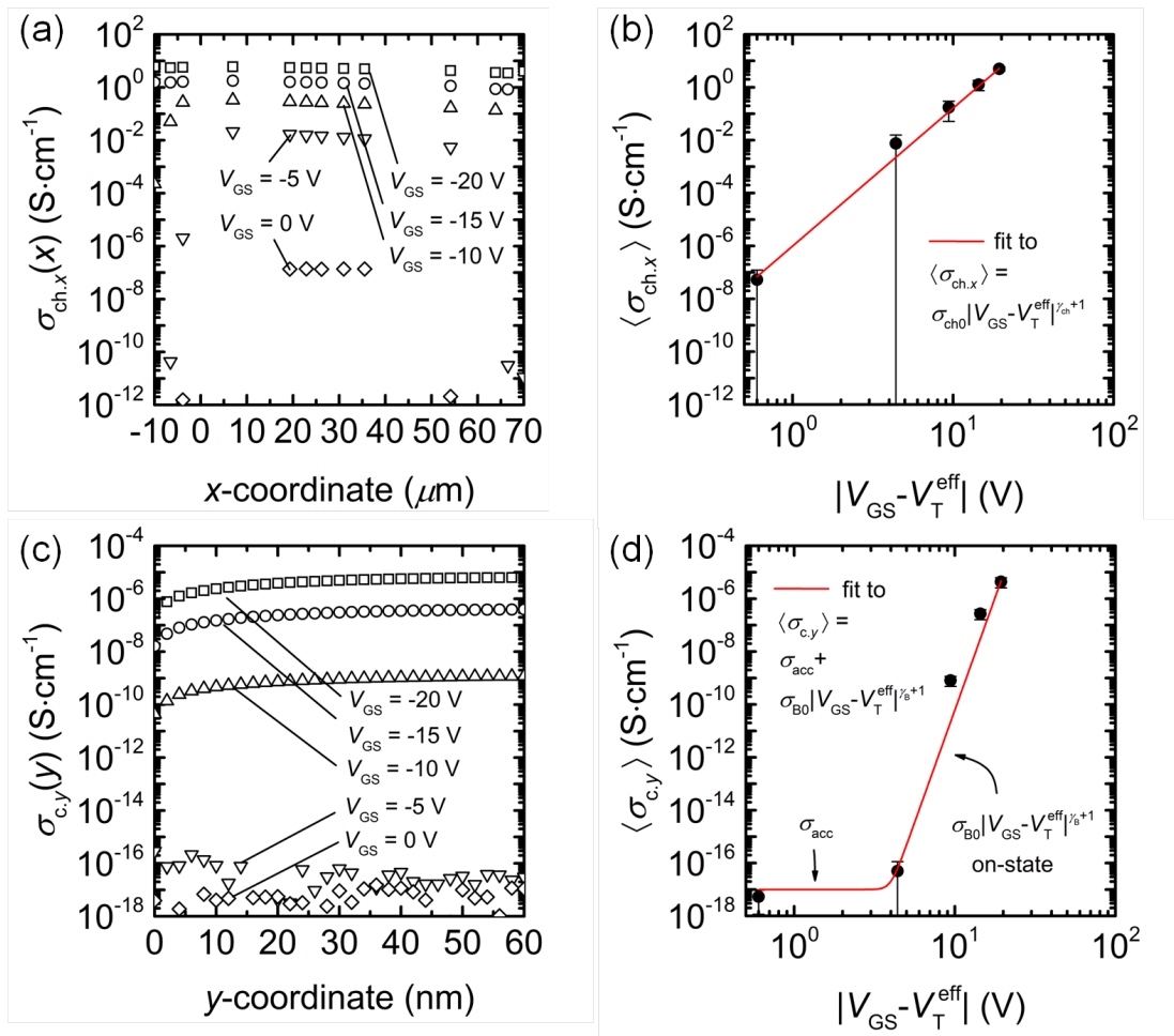
Figure 5-4: (a) Channel conductivity \sigma_{\text{ch},x} and (b) its average on x -axis \langle\sigma_{\text{ch},x}\rangle (at y = 2 nm), and (c) contact conductivity in the transition zone \sigma_{\text{c},y} and (d) its average on y -axis \langle\sigma_{\text{c},y}\rangle (at x = -5 \mu\text{m} ) calculated at various gate voltage: V_{\text{GS}} = 0, -5, -10, -15 and -20 V. Note the power-law dependence of both channel and contact conductivity with respect to the effective gate voltage. In particular, \langle\sigma_{\text{c},y}\rangle contains an asymptotic element \sigma_{\text{acc}} and a power-law dependent element \sigma_{\text{B}} .
