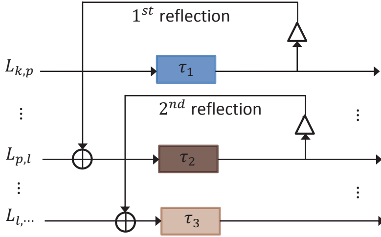
Figure 6.5: Illustration of the feedback of the signals described by the discretized acoustic rendering equation for specular reflections.
