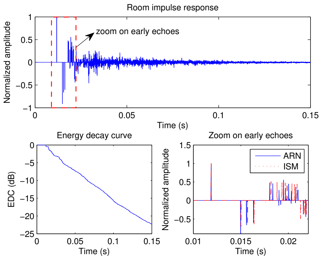
Figure 6.12: Simulation results of Room 2 with absorption \alpha = 0.25 .
