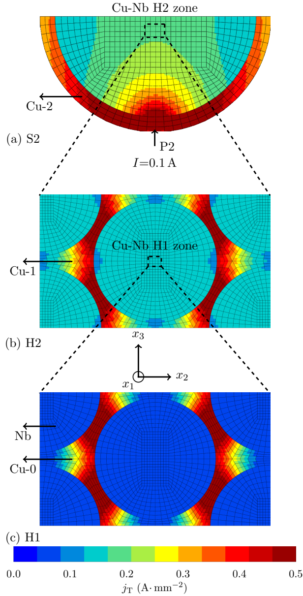
FIGURE 3.8: Transverse current density j_T = \sqrt{j_2^2 + j_3^2} distribution for N=85^2 Cu-Nb Filamentary wires with a diameter of 2.10 mm at (a) the effective scale S2, (b) H2 and (c) H1.
