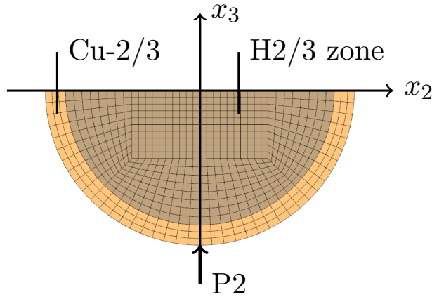
FIGURE 3.6: Section view of the FE mesh at S2/3 scale for N=85^2 and N=85^3 respectively.
