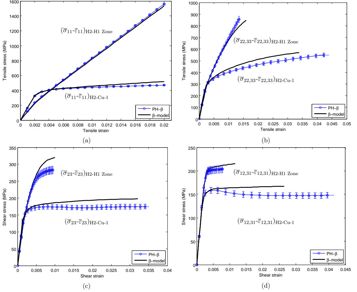
FIGURE 5.10: Individual behavior of the H1 Cu-Nb composite zone and Cu-1 component at H2 predicted by PH- \beta and \beta -model for the: (a) LT test, (b) TT test, (c) TS test and (d) LS test.
