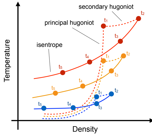
Figure 3.7: Scheme of the experimental strategy of this campaign. The laser intensity and the time delay set the conditions measured with the absorption spectroscopy.
