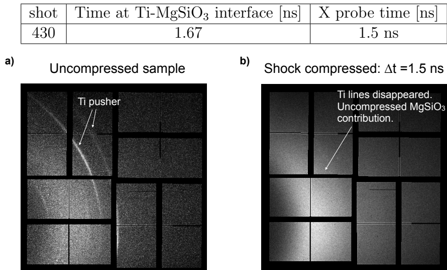
Figure 4.17: a) Reference measurements showing the xrd pattern of the unshocked sample (shot 430). Ti contributions is evident in the two sharp lines (pointed by the white arrows) and the \text{MgSiO}_3 glass contributes with the typical broad peak. b) XRD pattern of the same target of the reference signal shown on the left shock compressed and with a drive laser probe delay time equal to 1.5 ns (shot 430).
