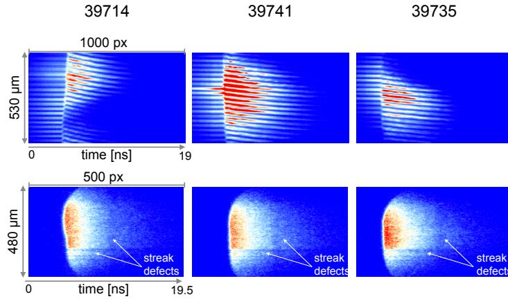
Figure 2.44: Typical VISAR and SOP signals obtained for the \text{MgSiO}_3 .
