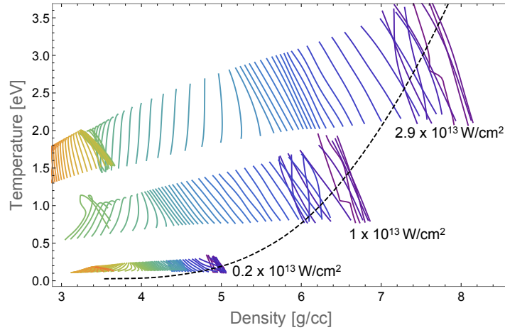
Figure 3.13: Time evolution of the thermodynamic conditions in the MgO layer obtained with MULTI simulations performed with drive laser pulses with intensities of 0.2 \cdot 10^{13} \text{ W/cm}^2 , 1 \cdot 10^{13} \text{ W/cm}^2 , 2.9 \cdot 10^{13} \text{ W/cm}^2 . Each set of lines correspond to the intensity pointed at its bottom right. Each line represents an instantaneous of the thermodynamic conditions in the MgO layer and are taken each 10 ps. Each color represent a time and the discretisation is 10 ps.
