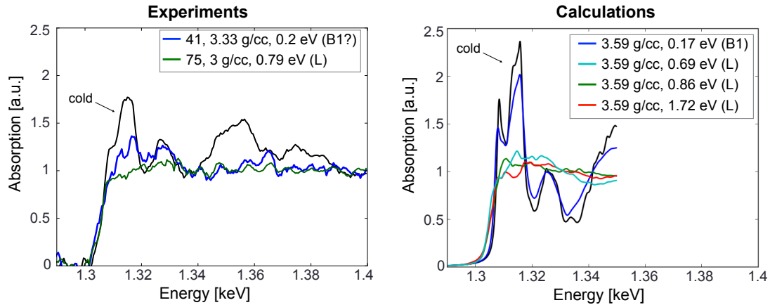
Figure 3.34: Experimental XANES spectra (left) and spectra obtained with ab-initio calculation for various temperature along the isochore at 3.59 g/cc. B1 and L denotes B1 solid phase and the liquid phase.
