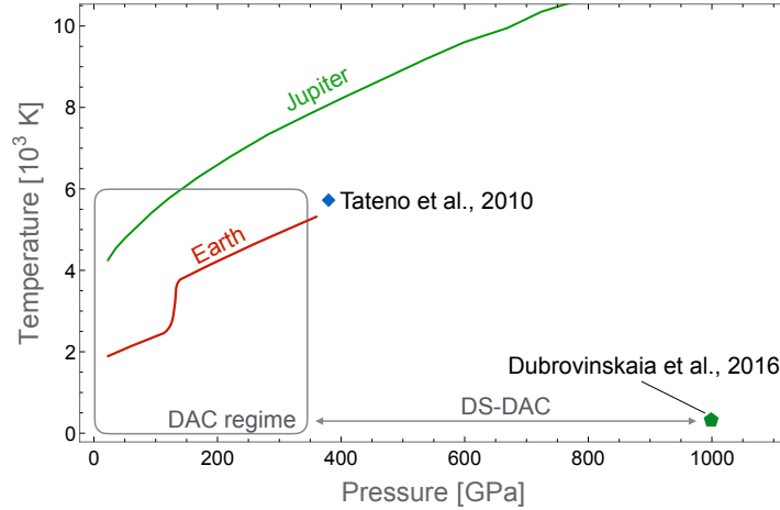
Figure 6: Conditions achievable using different methods of static pressure generation.
