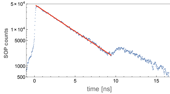
Figure 2.27: Example of a thermal emission time profile obtained at LULI for the MgO. This profile was obtained with a 1.2 ns laser pulse of 726.7 J and 600 \mu m
