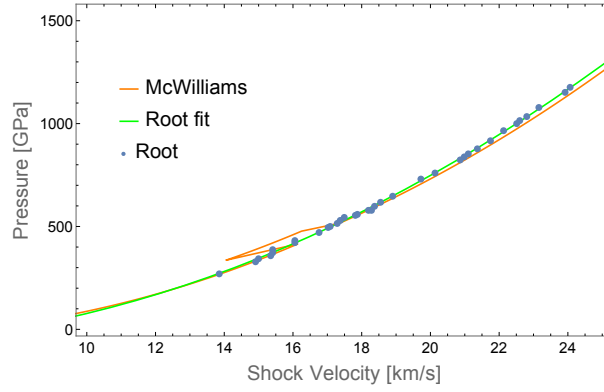
Figure 2.32: The interpolation of MgO P-Us data (blue dots) collected by [Root et al., 2015] is represented with a green line and is compared to the Mie-Grüneisen-Debye model reported by McWilliams et al. [2012] showing no significant differences
