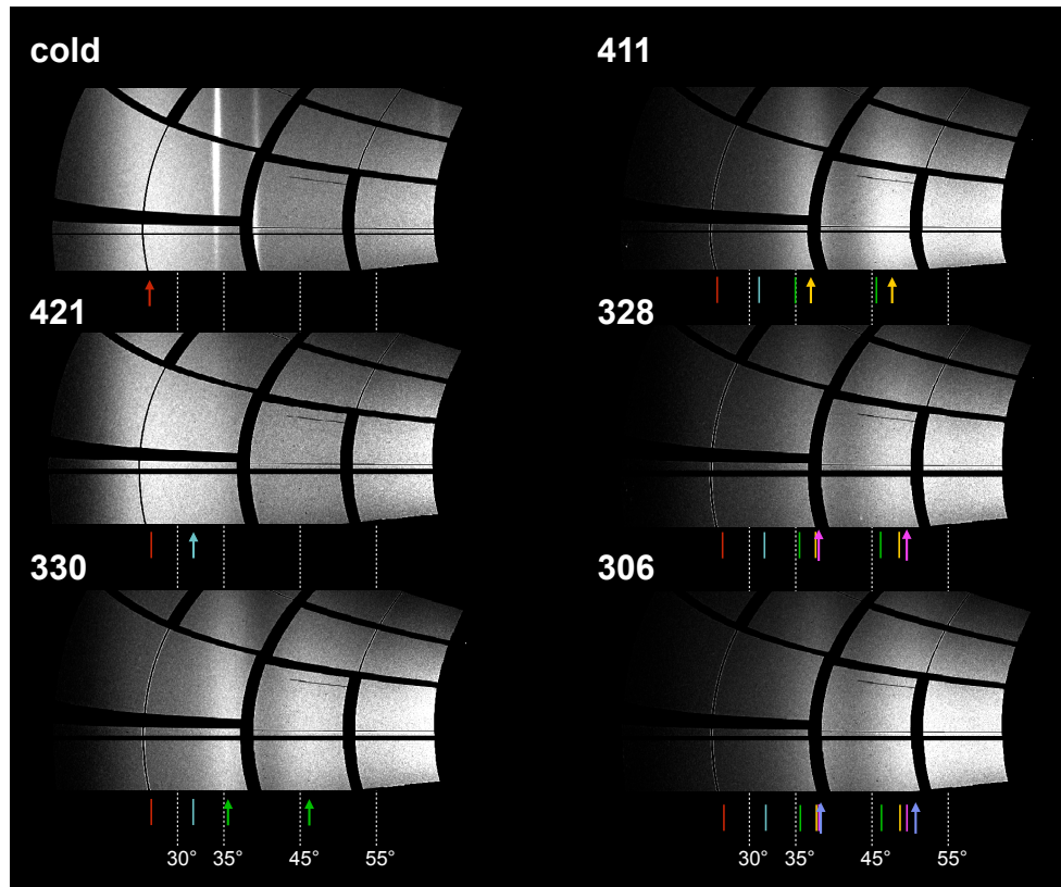
Figure 4.12: XRD patterns of shocked \text{MgSiO}_3 glass
