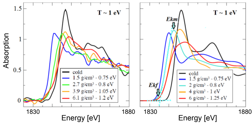
Figure 3.29: Experimental (left) and theoretical (right) SiO 2 XANES spectra for different densities and fixed temperature ( \sim 1 eV) as reported in [Denoeud et al., 2016a].
