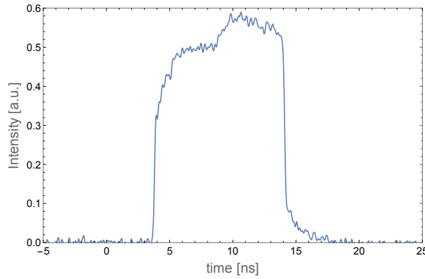
Figure 4.4: Typical drive laser time profile used during this experimental campaign.
