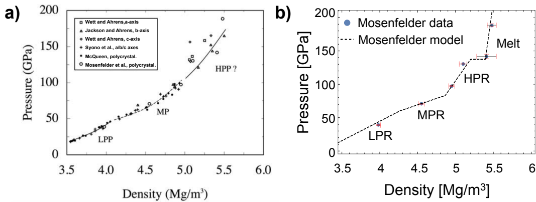
Figure 4.2: a) from [Mosenfelder et al., 2007] Fo shock P - \rho data from various gas gun and laser driven shock compression experiments. b) The Fo theoretical Hugoniot obtained with a Mie-Grüneisen proposed by [Mosenfelder et al., 2007]
