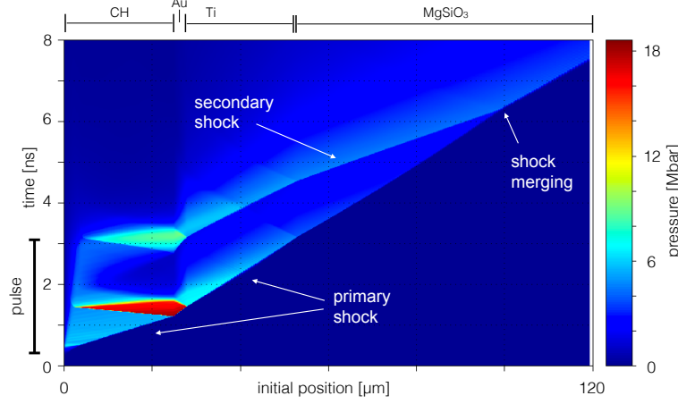
Figure 2.21: Color plot of the pressure versus time and initial position of a 25\text{ }\mu\text{m} CH + 3\text{ }\mu\text{m} Au + 25\text{ }\mu\text{m} Ti + 300\text{ }\mu\text{m} MgSiO 3 target compressed by a shock generated by a laser pulse of 2.5\text{ ns} and 2.4 \cdot 10^{13}\text{ W/cm}^2 obtained with a MULTI simulation. In this case a second shock forms and reaches the first shock at 6.5\text{ ns}
