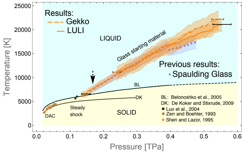
Figure 2.47: The experimental \text{MgSiO}_3 glass P-T curves measured along the Hugoniot at LULI (orange full line) and at Gekko (dotted orange line) are represented in \text{MgSiO}_3 phase diagram in comparison with previous experimental results (blue disk and square) [Spaulding et al., 2012]. Black lines represent theoretical melting lines.
