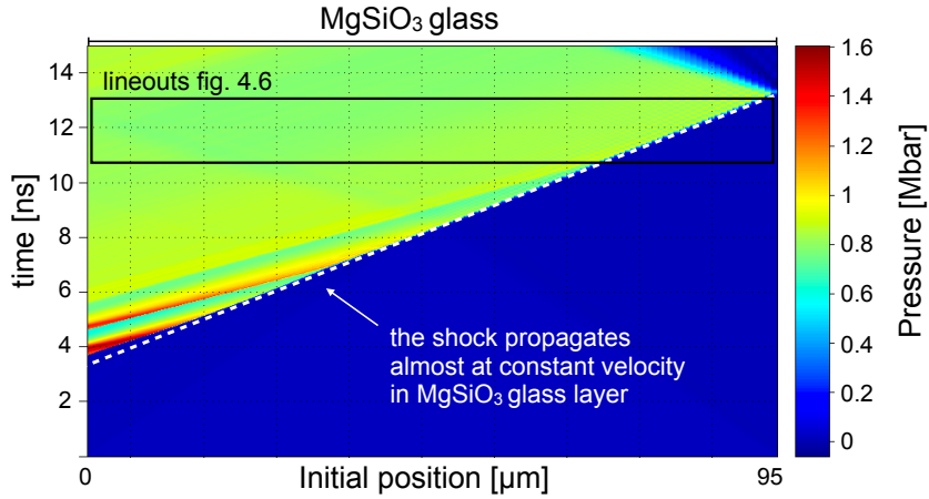
Figure 4.5: Color plot of the pressure in the time-initial position plane obtained with MULTI hydrodynamic simulation for a 10 ns long drive pulse of 4 \cdot 10^{12}\ \text{W}/\text{cm}^2 irradiated on a 10\ \mu\text{m} CH+ 2\ \mu\text{m} Ti+ 95\ \mu\text{m} \text{MgSiO}_3 glass target.
