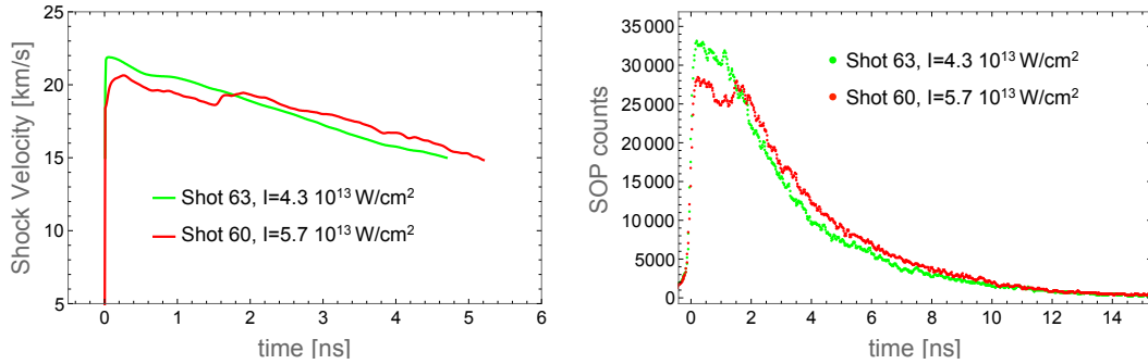
Figure 2.24: On the left, shock velocities profile for shot 60 (1.5 ns pulse of 5.7 \cdot 10^{13} \text{ W/cm}^2 ) and 63 (1.5 ns pulse of 4.3 \cdot 10^{13} \text{ W/cm}^2 ) obtained respectively with pusher 1 and pusher 2 on \text{SiO}_2 samples. Shot 60 exhibits a clear jump due to a reverberation since in quartz no transition is expected in the range of the measured velocities. Shot 63 indeed exhibits the typical behavior of a decaying shock propagation in a single phase. On the right, luminance profile for shot 60 and 63. As for the shock velocities, the luminance of shot 60 exhibits a clear jump due to a reverberation while shot 63 indeed exhibits the typical behavior of a decaying shock propagation in a single phase also for the thermal emission.
