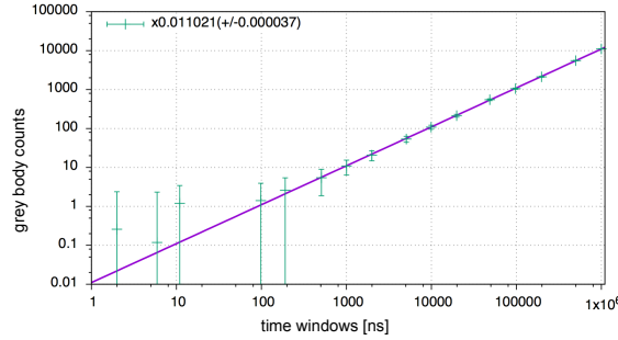
Figure 2.9: The number of SOP counts produced by the light emitted by a lamp at 2588 \text{ K} \pm 15 \text{ K} and selected with a gaussian filter centered at 450 nm and with a FWHM of 40 nm is represented for each SOP time window with green cross. Each point is the result of an average over 100 measurements. Here, gray-body count stays for the measured signal minus the dark noise of the SOP (the background signal measured with the shutter closed).
