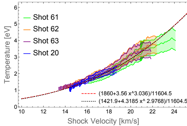
Figure 2.12: The \text{SiO}_2 T - U s curves obtained for different shots (20,63,61,62) at LULI are compared to T - U s interpolation of data from [Hicks et al., 2006] reported in literature [Brygoo, 2006; Millot et al., 2015]
