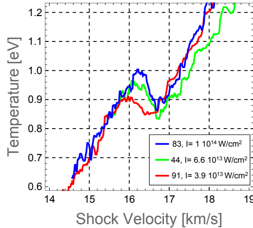
Figure 2.34: Zoom of the bump for the MgO P-T curves obtained with shot 83, shot 44 and shot 91 that have been performed with 1.2 ns laser pulse of 600 \mu m diameter and energies of 726 J, 448 J and 265 J respectively. The bump varies for shots performed with different energies, suggesting that we are observing a non-equilibrium phenomenon.
