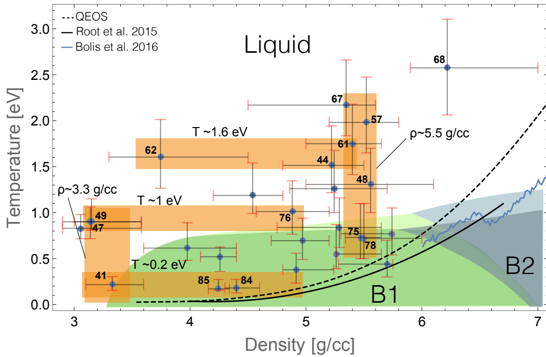
Figure 3.24: Thermodynamic conditions probed with the absorption spectroscopy (blue dots) represented on the MgO phase diagram. The orange areas point the selected isochores and isotherms.
