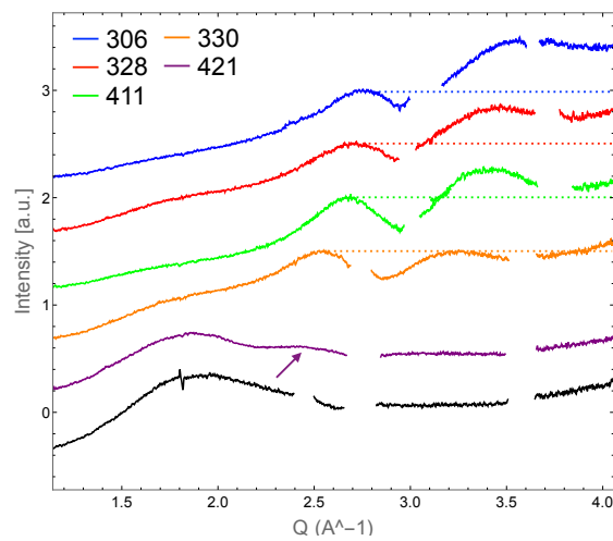
Figure 4.13: X ray diffraction spectra obtained on shocked \text{MgSiO}_3 glass for increasing laser intensities (coloured lines) are compared with the spectrum at standard conditions (black line).
