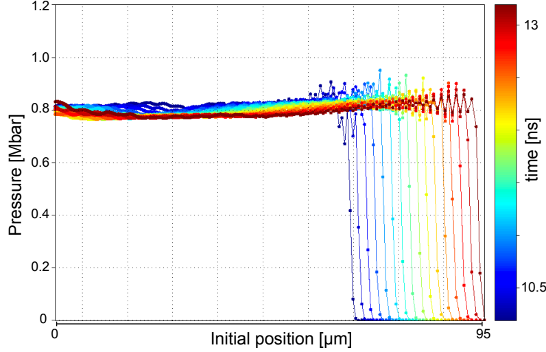
Figure 4.6: Pressure versus initial position curves for times close to the time break out obtained with MULTI hydrodynamic simulation for a 10 ns long drive pulse of 4 \cdot 10^{12} W/cm 2 irradiated on a 10 \mu\text{m} CH+ 2 \mu\text{m} Ti+ 95 \mu\text{m} \text{MgSiO}_3 glass target. Uniform pressures of 0.8 Mbar are obtained over the whole samples.
