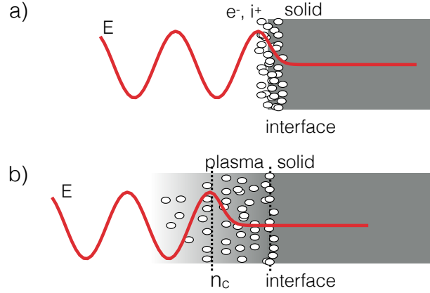
Figure 1.1: Laser-matter interaction at the first stages. a) In the first femto-picoseconds the laser ionises the atoms of the solid in a region near to the surface. The spatial range of interaction between the laser and the atoms inside the solid is given by the laser penetration depth (skin depth). b) Later in time the ionised atoms forms a plasma that expands as it is heated by the laser. However the laser can transfer its energy to the plasma just in the low density region, i.e. before plasma critical density n_c .
