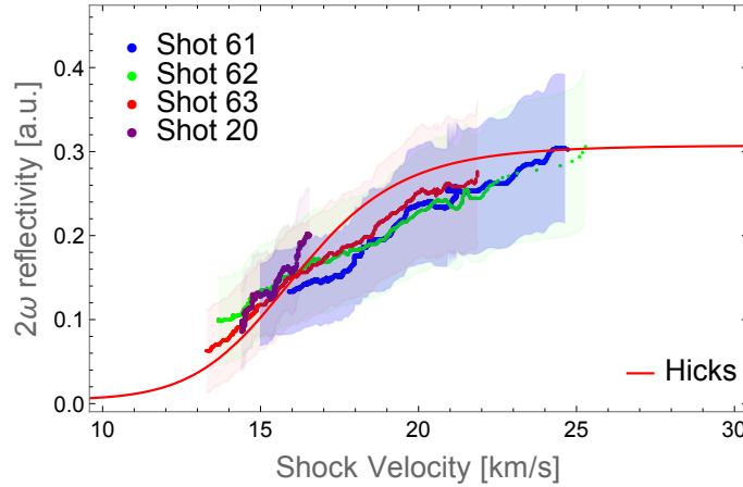
Figure 2.26: \text{SiO}_2 2\omega reflectivity (coloured small dots) obtained at LULI in comparison with [Hicks et al., 2006] curve (red line).
