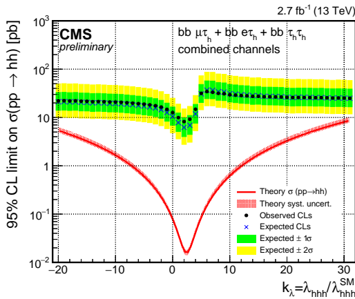
(a) Nonresonant search
