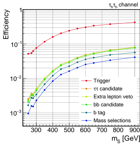
(e) spin-0, \tau_h \tau_h
