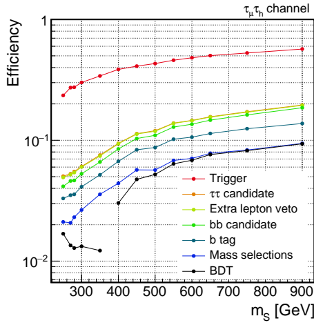
(a) spin-0, \tau_\mu \tau_h
