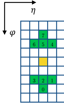
Figure 3.8 – Schematic representation of the area used for cluster merging. Every square represents a TT, the yellow one is the seed TT and the green one are the TTs considered as seeds for the secondary cluster. The numbering scheme of the secondary cluster seeds adopted in the firmware implementation is reported in the figure.
