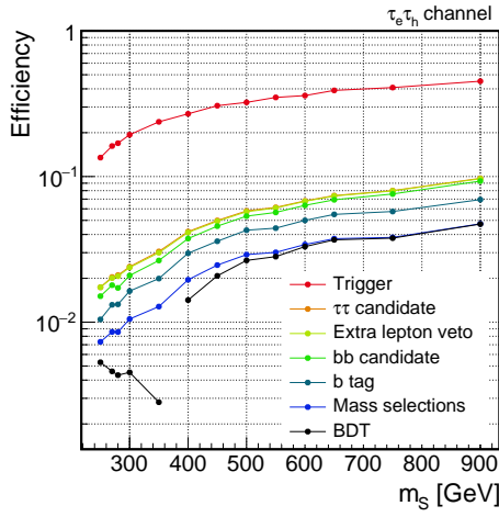
(c) spin-0, \tau_e \tau_h
