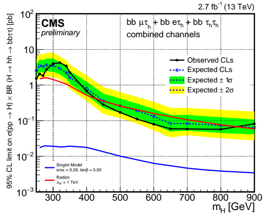
(b) Resonant search
